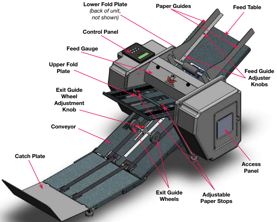
Figure 6: Machine Diagram
