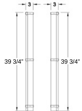
Cleats
