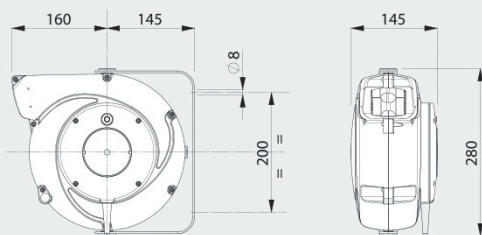
5907 Series dimensions
