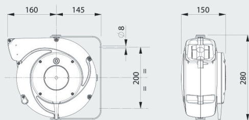
5908 Series dimensions
