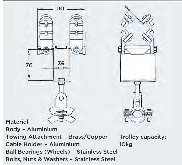
Towing Trolley Ref. 2307(A1)/A/B/C-6-Ex
