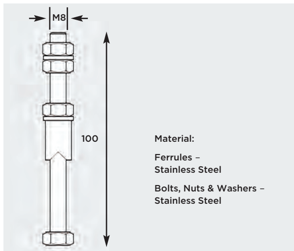
Track Support Ref. 2307-4-Inox
