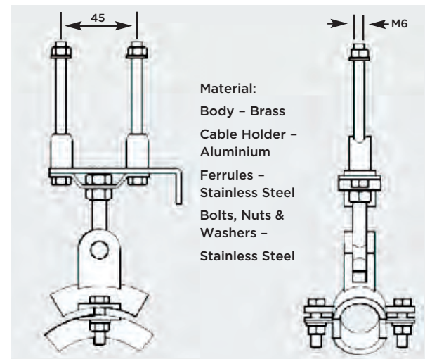
End Clamp Ref. 2307/A/B/C-2-Ex
