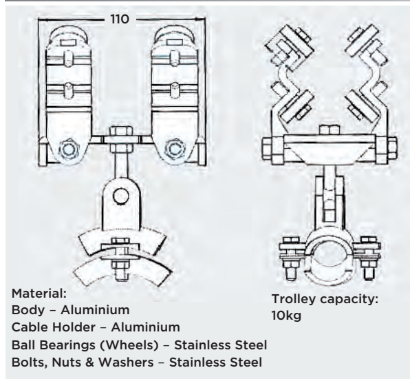
Cable Trolley Ref. 2307(A1)/A/B/C-5-Ex
