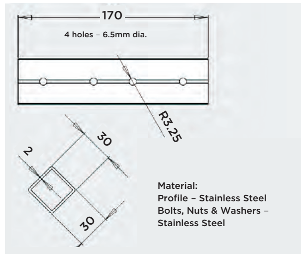
Track Joint Ref. 2307-3-Inox
