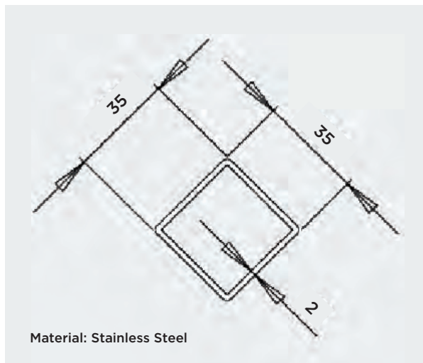
Track Profile Ref. 2307-1-Inox
