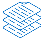
DATA CLASSIFICATION
