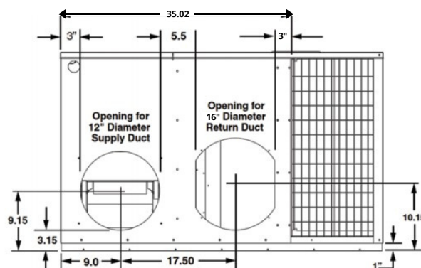
REAR VIEW
