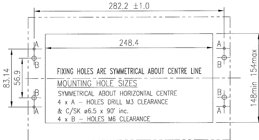
PANEL CUT OUT DETAIL FOR MOUNTING OF RACK
