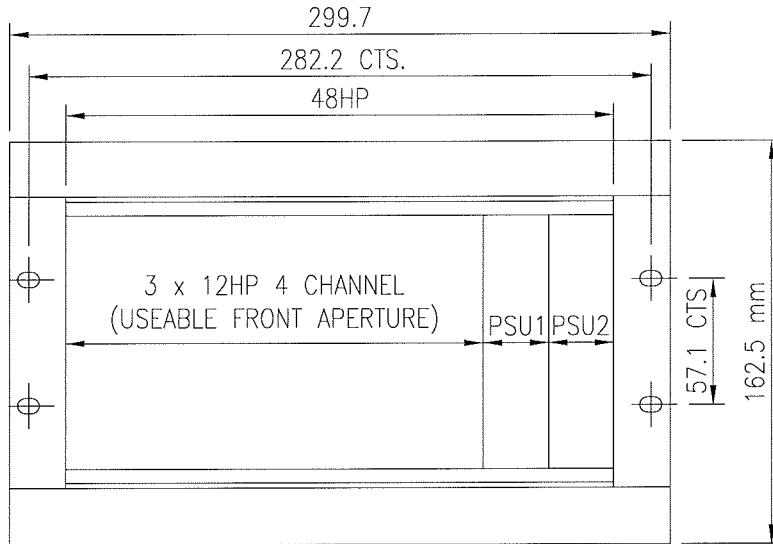
FRONT OF THE RACK
