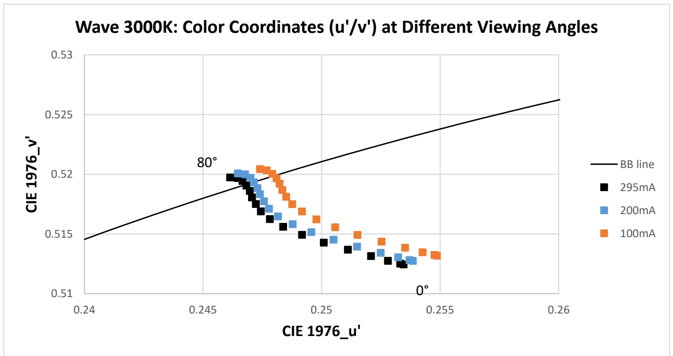
Figure 24: CIE u'/v' as function of the viewing angle. Driving currents I= 0.100 A, 0.200 A, 0.295 A, 3000K, level I
