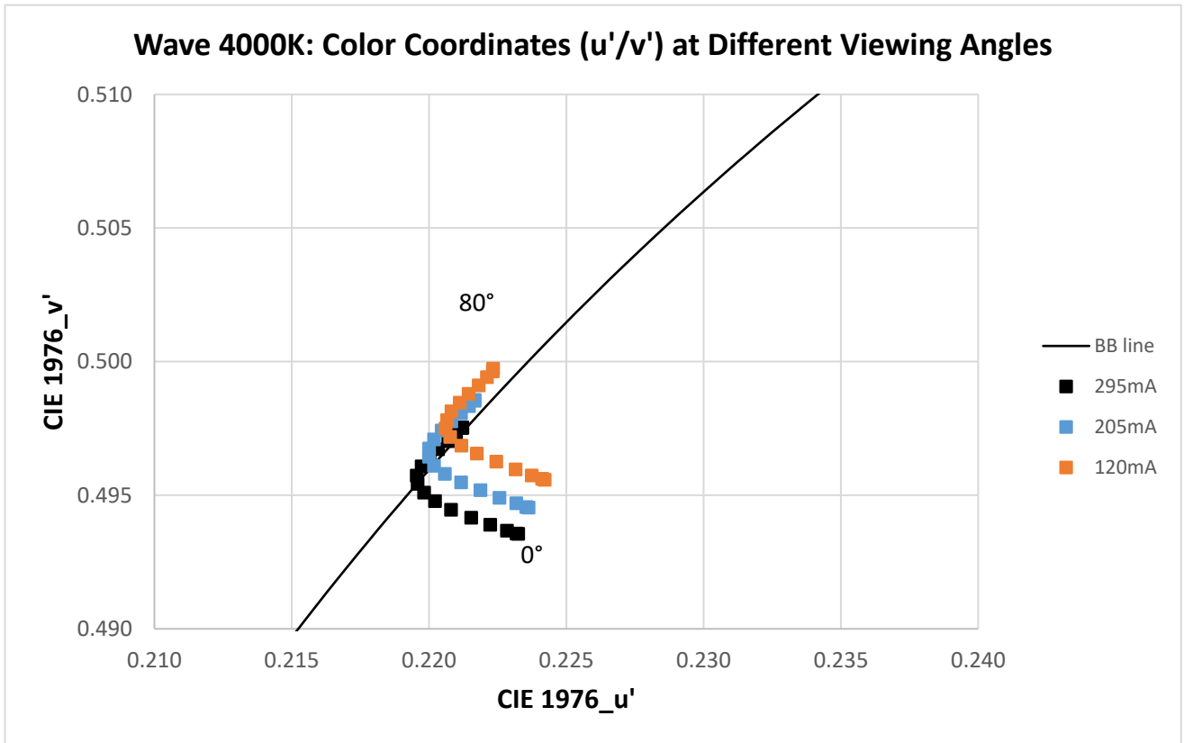
Figure 23: CIE u'/v' as function of the viewing angle. Driving currents I= 0.120 A, 0.205 A, 0.295 A, 4000K, level I
