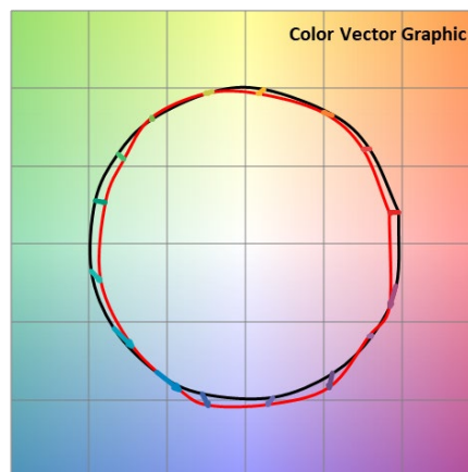
Figure 11: Color vector graphic based on TM-30 metrics for Brite 3 Rectangle 3000K
