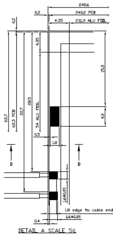
Figure 4: Brite 3 Rectangle Level 1.5 - Detail A of Figure 3
