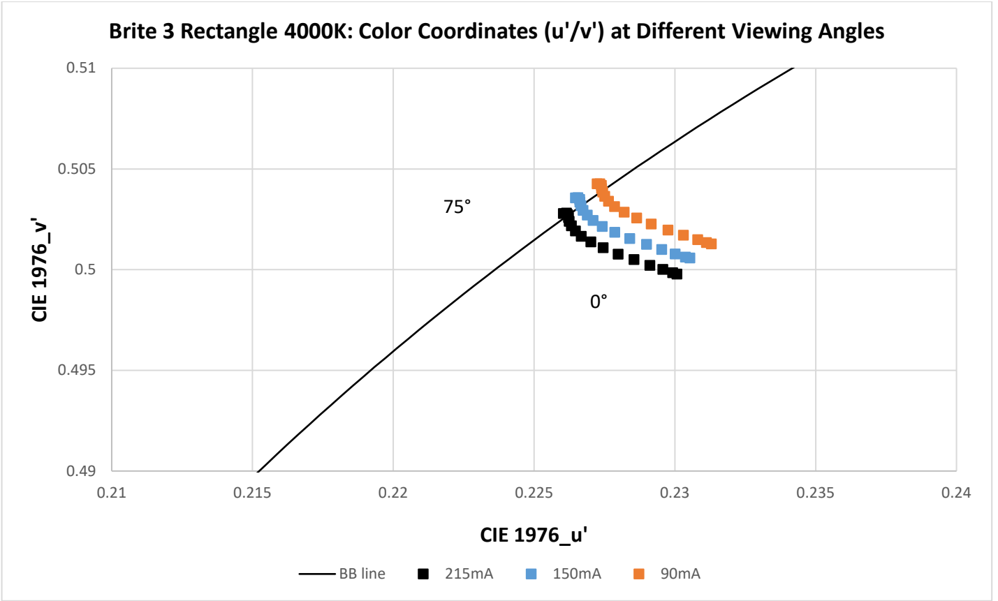
Figure 27: CIE u'/v' as function of the viewing angle. Driving currents I= 0.090 A, 0.150 A, 0.215 A, 4000K
