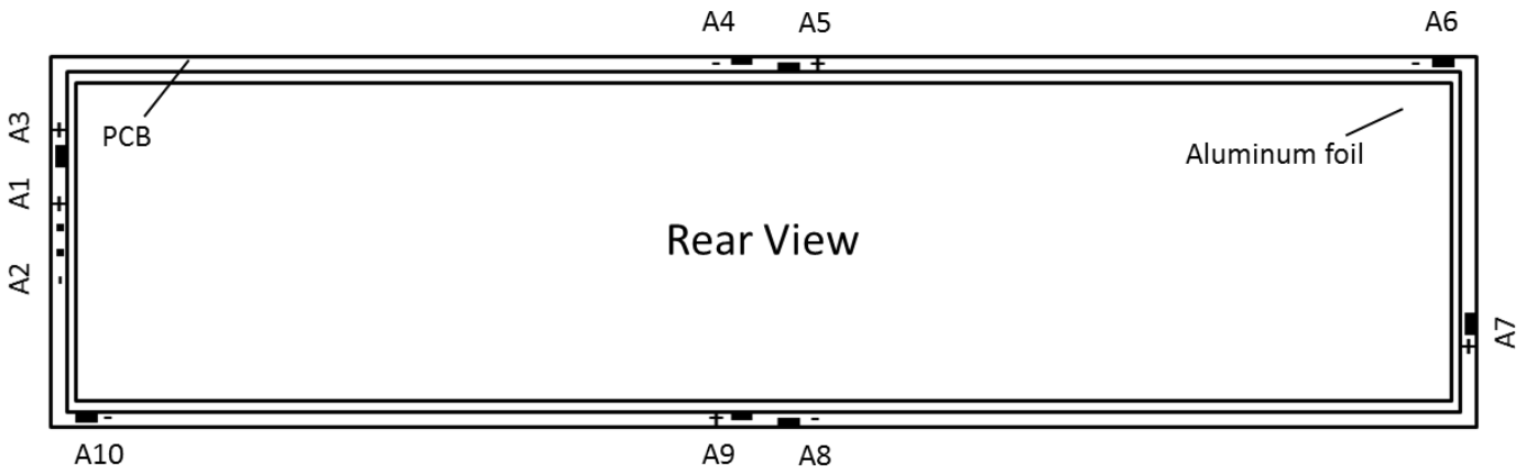
Figure 7: Contact pads of the Brite 3 Rectangle Level 1
