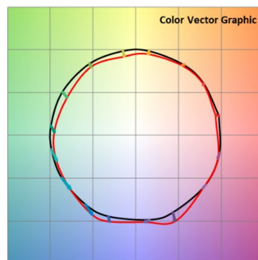
Figure 10: Color vector graphic based on TM-30 metrics for Brite 3 Rectangle 4000K
