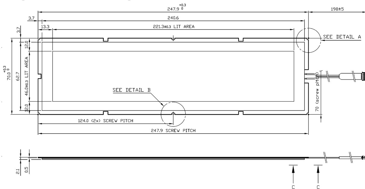
Figure 5: Brite 3 Rectangle Level 2 – front and side view (top), side view (bottom)
