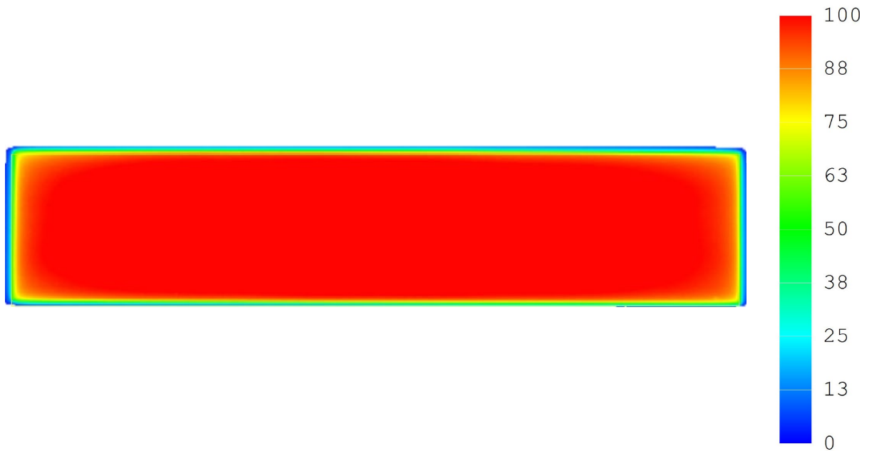
Figure 22: Typical luminance distribution for a Brite 3 Rectangle Level 1. Operation conditions: vertical in air, RT (= 25 °C), I = I_{in\ rated}
