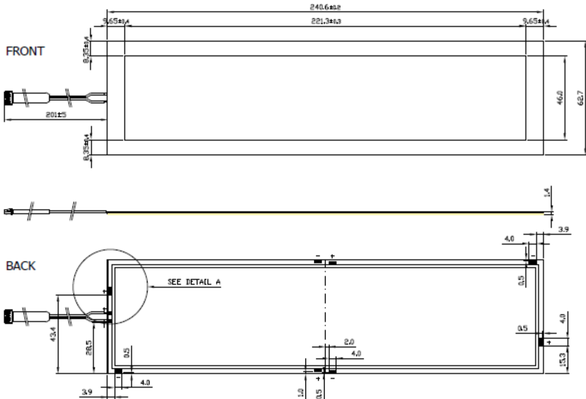
Figure 3: Brite 3 Rectangle Level 1.5 – front (top), side view (middle), rear view (bottom)
