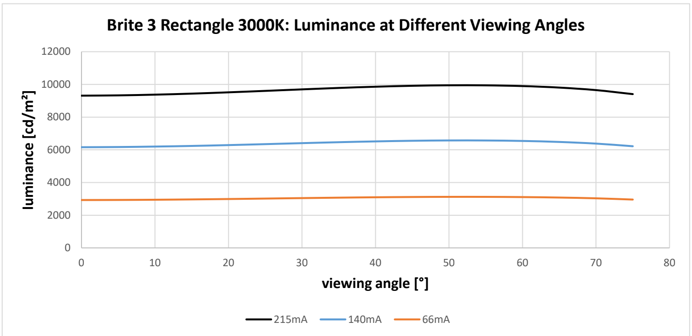
Figure 24: Luminance as function of the viewing angle. Driving currents I = 0.066 \text{ A}, 0.140 \text{ A}, 0.215 \text{ A}, 3000\text{K}
