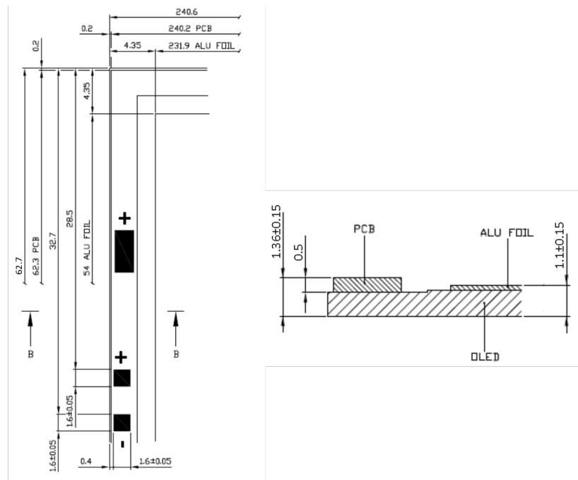
Figure 2: Detail A of Figure 1 (left) and cross section B-B (right); Brite 3 Rectangle Level I
