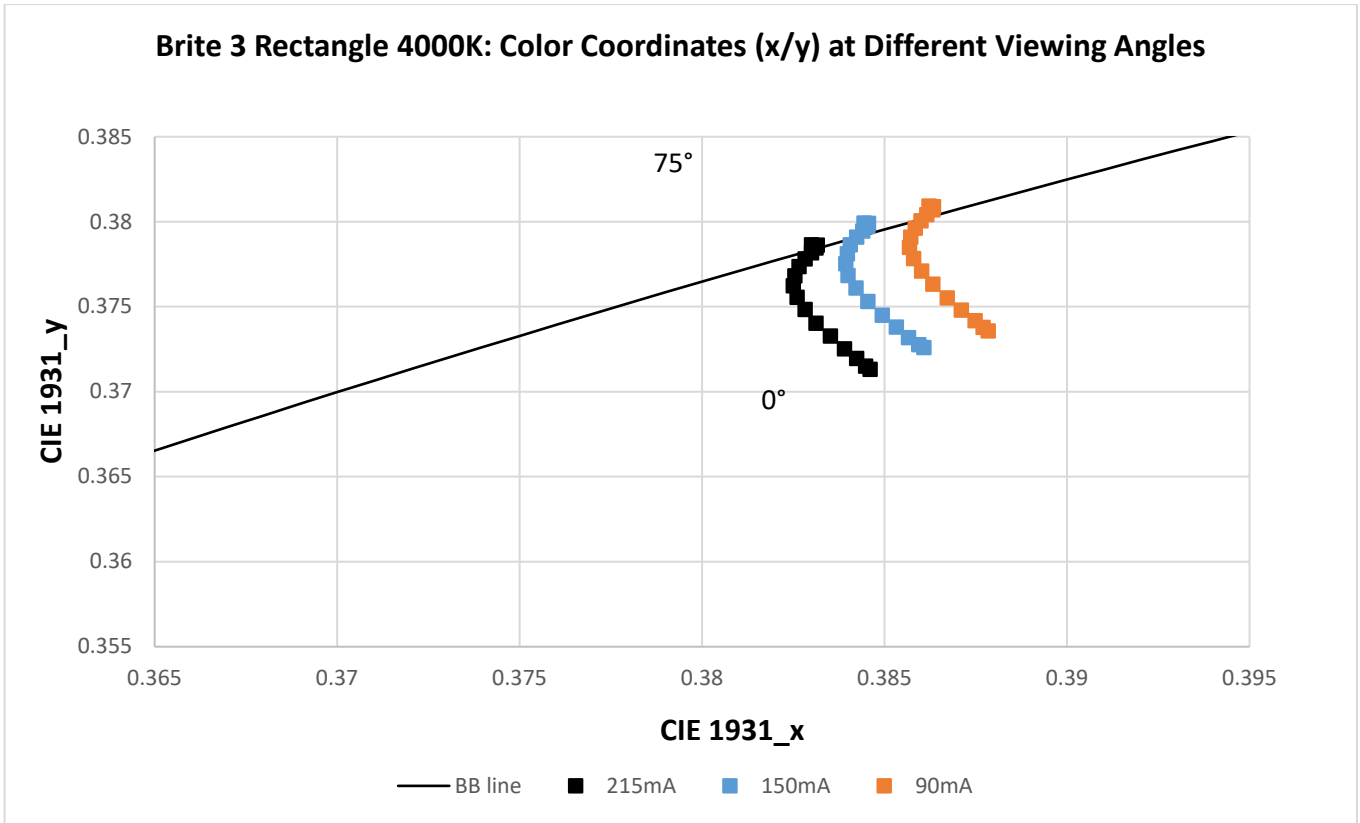
Figure 25: CIE x/y as function of the viewing angle. Driving currents I= 0.090 A, 0.150 A, 0.215 A, 4000K
