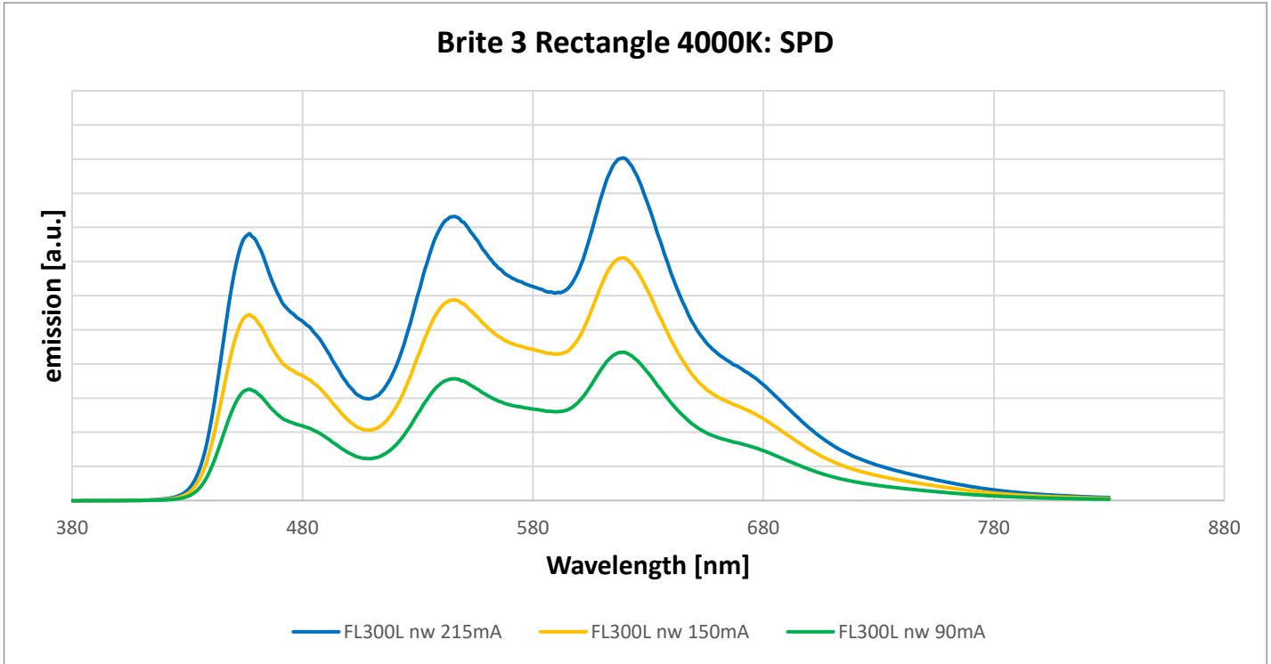
Figure 12: typical emission spectra of the Brite 3 Rectangle 4000K at different driving currents ( I = 0.090\text{ A}, 0.150\text{ A}, 0.215\text{ A} )
