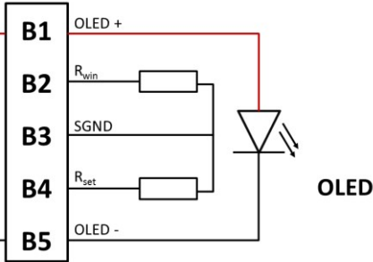
Figure 8: Channel connections from driver to the Brite 3 Rectangle Level 2
