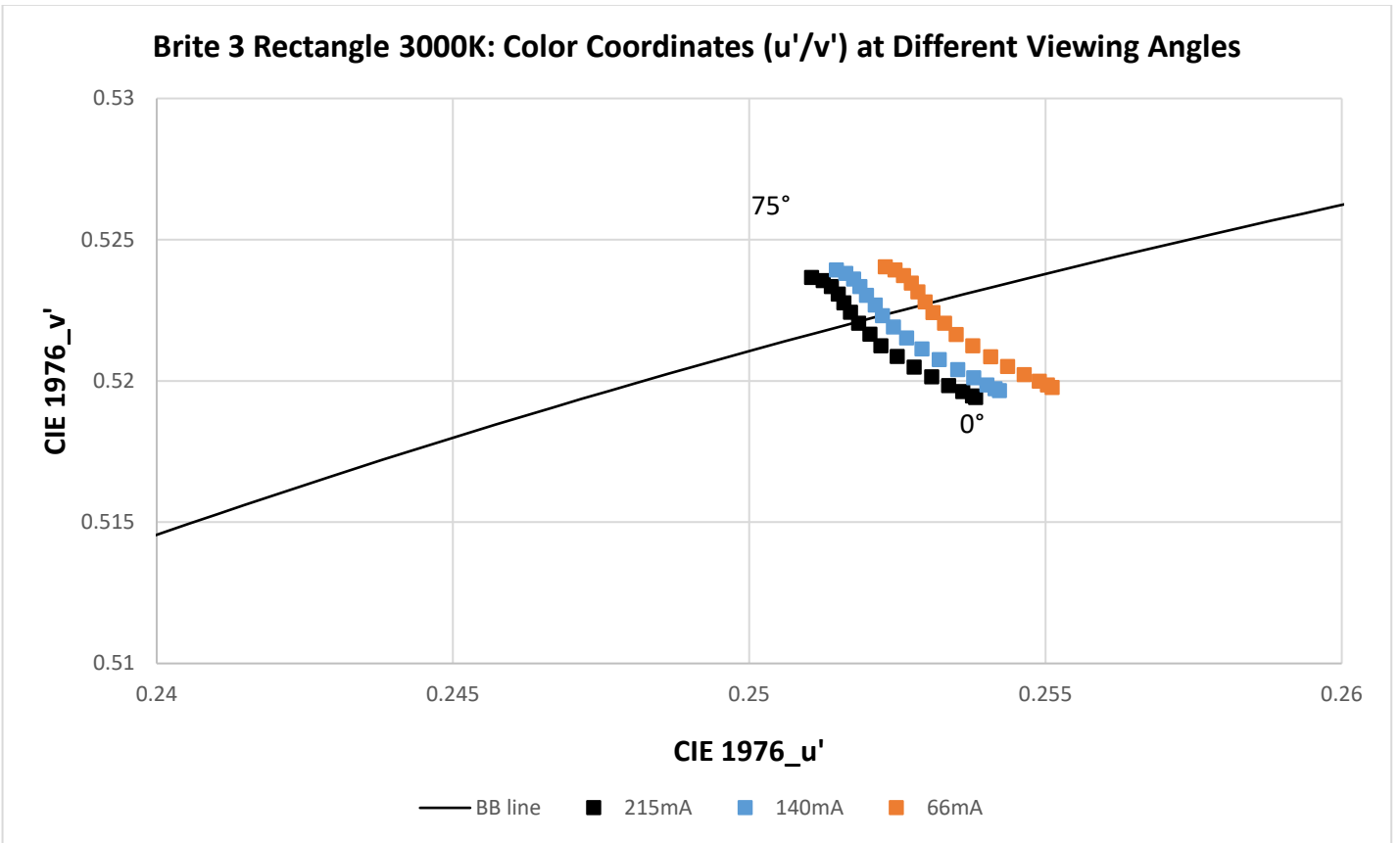
Figure 28: CIE u'/v' as function of the viewing angle. Driving currents I= 0.066 A, 0.140 A, 0.215 A, 3000K
