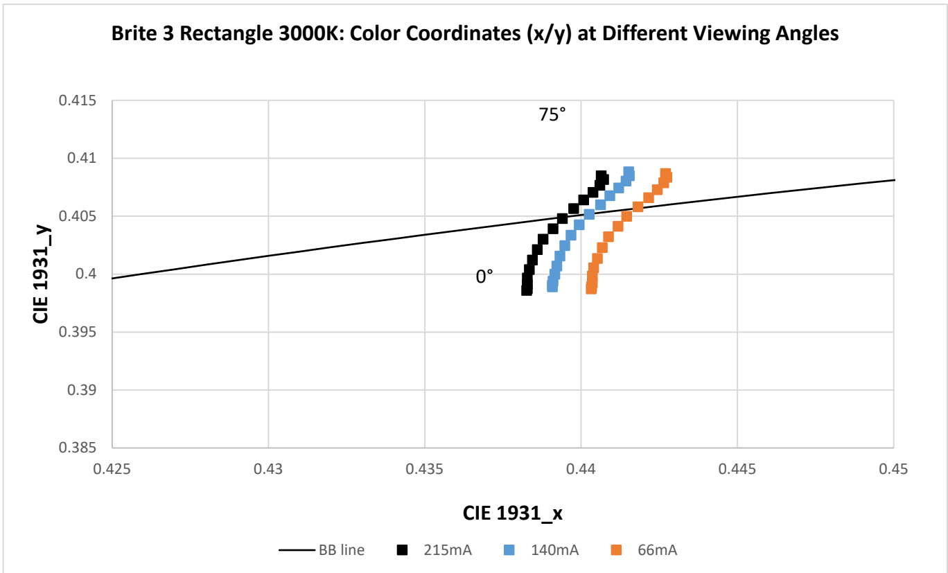
Figure 26: CIE x/y as function of the viewing angle. Driving currents I= 0.066 A, 0.140 A, 0.215 A, 3000K
