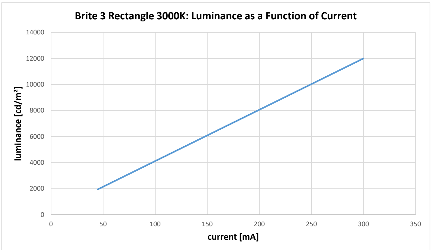
Figure 15: Luminance versus forward current at room temperature, 3000K, level 1
