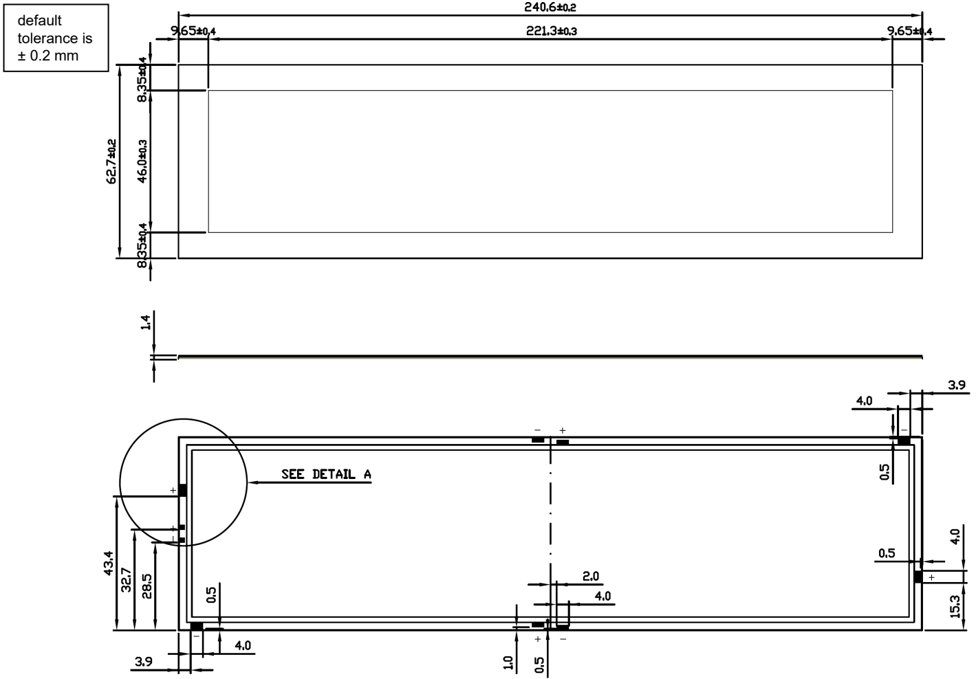
Figure 1: Brite 3 Rectangle Level I – front (top), side view (middle), rear view (bottom)
