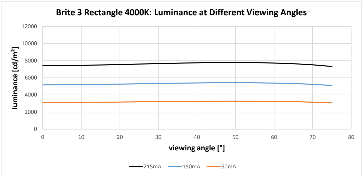
Figure 23: Luminance as function of the viewing angle. Driving currents I = 0.090 \text{ A}, 0.150 \text{ A}, 0.215 \text{ A}, 4000\text{K}
