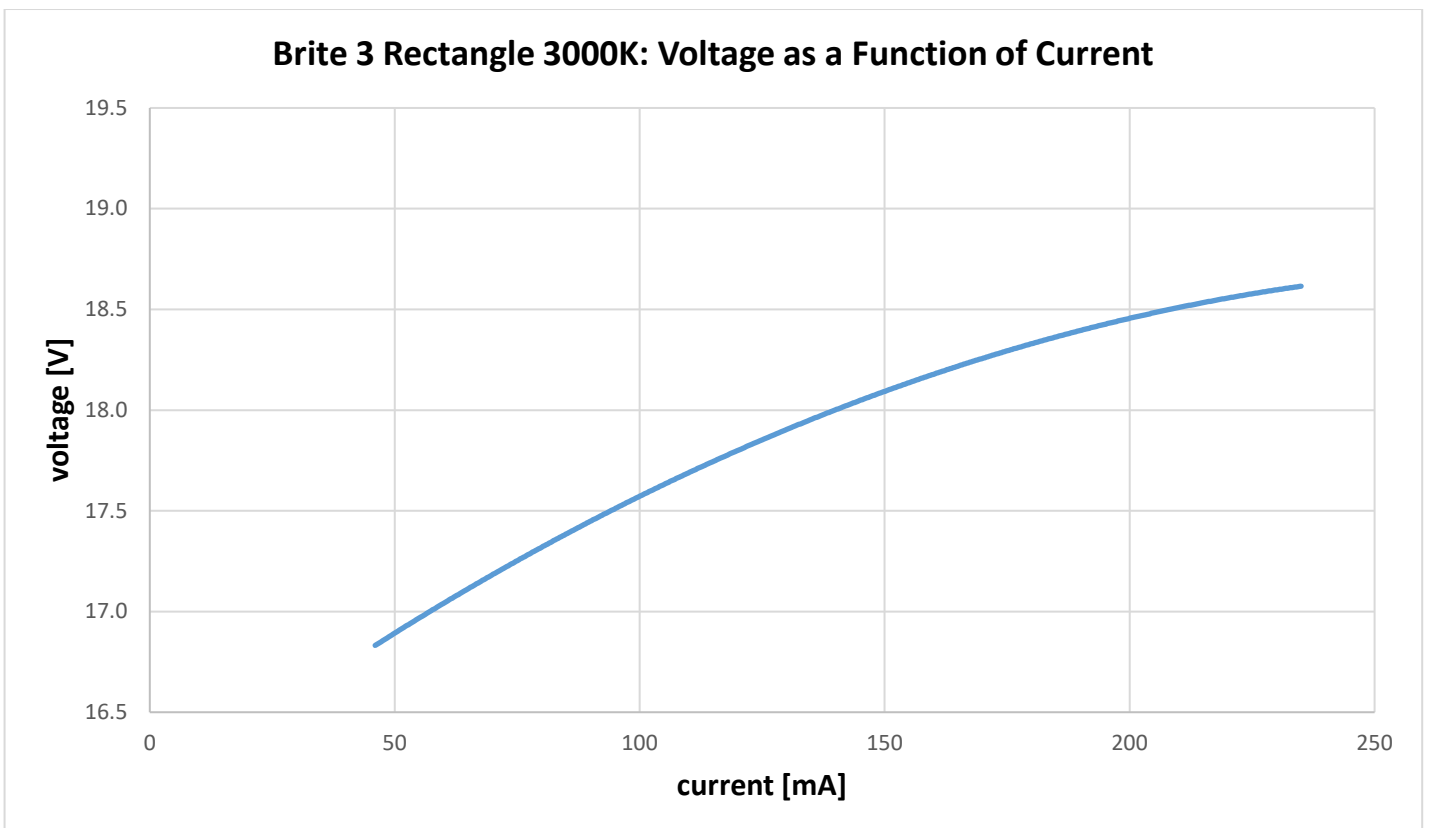
Figure 19: Voltage versus forward current at room temperature, 3000K, level 1
