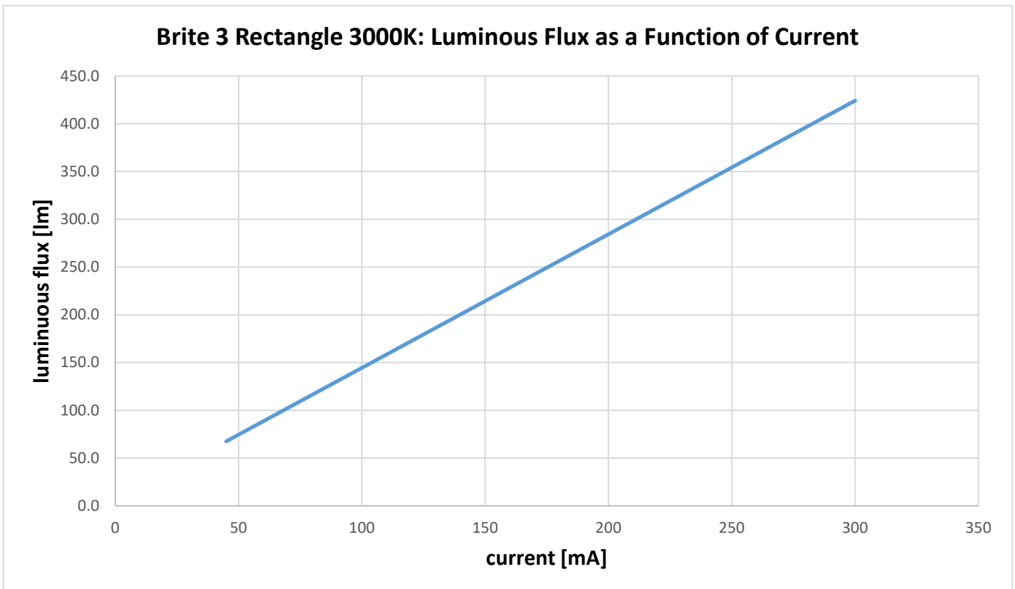
Figure 17: Luminous flux vs current, 3000K, level 1
