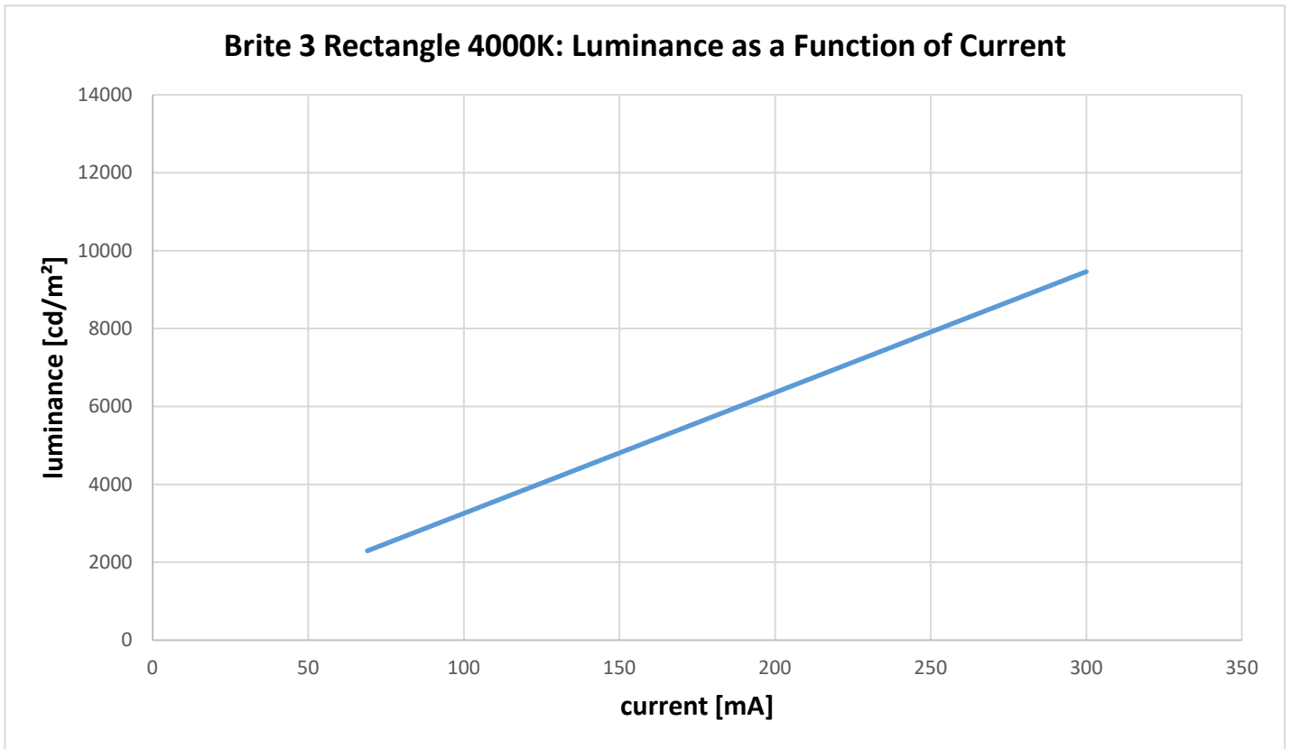
Figure 14: Luminance versus forward current at room temperature, 4000K, level 1
