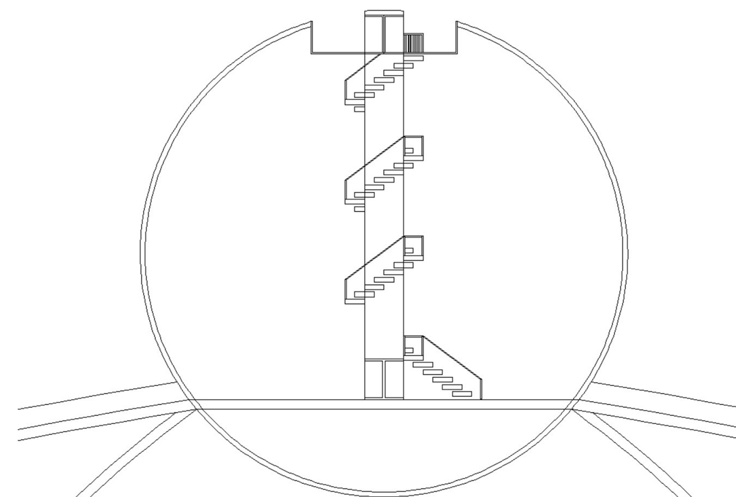
Cross Section of Sphere Showing Observation Deck, Elevator and Staircase
