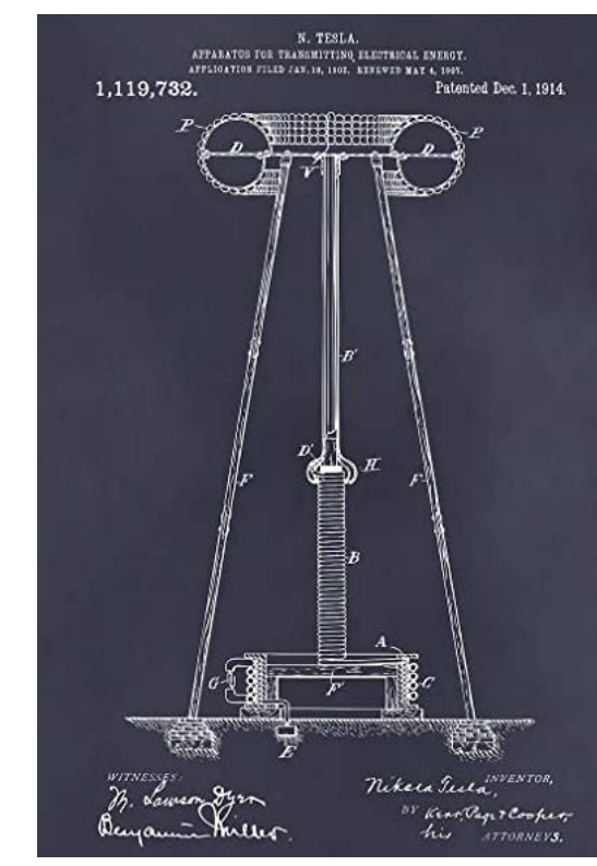
APPARATUS FOR TRANSMITTING, ELECTRICAL ENERGY NIKOLAS TESLA PATENT
