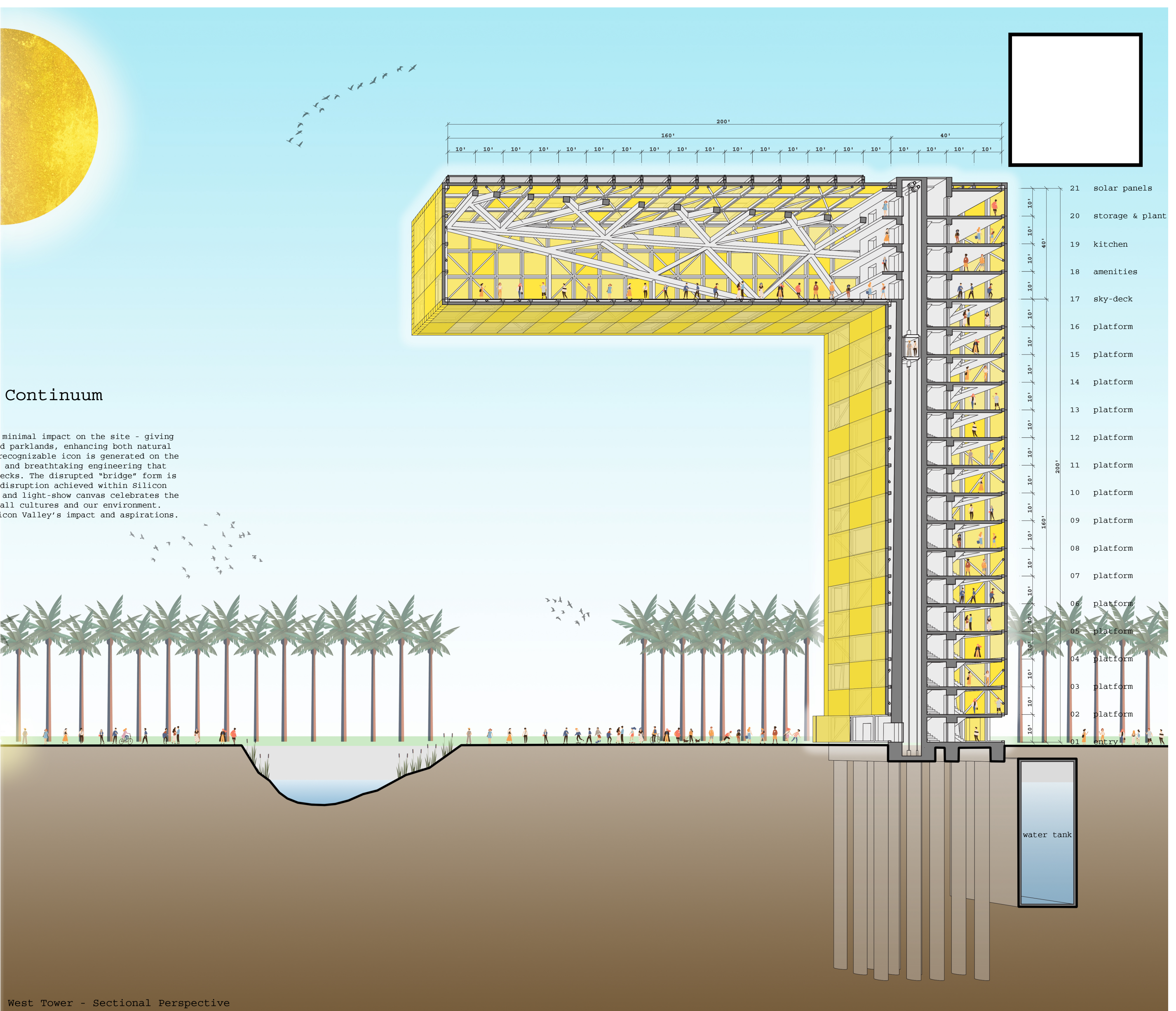
West Tower - Sectional Perspective
