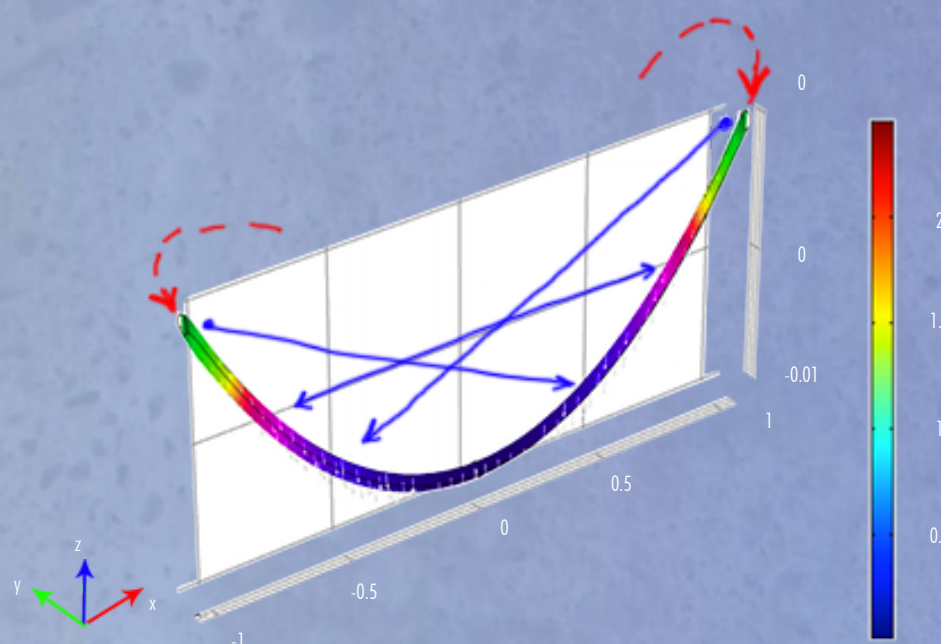
Tension Distribution On Catenary Compression Ring
