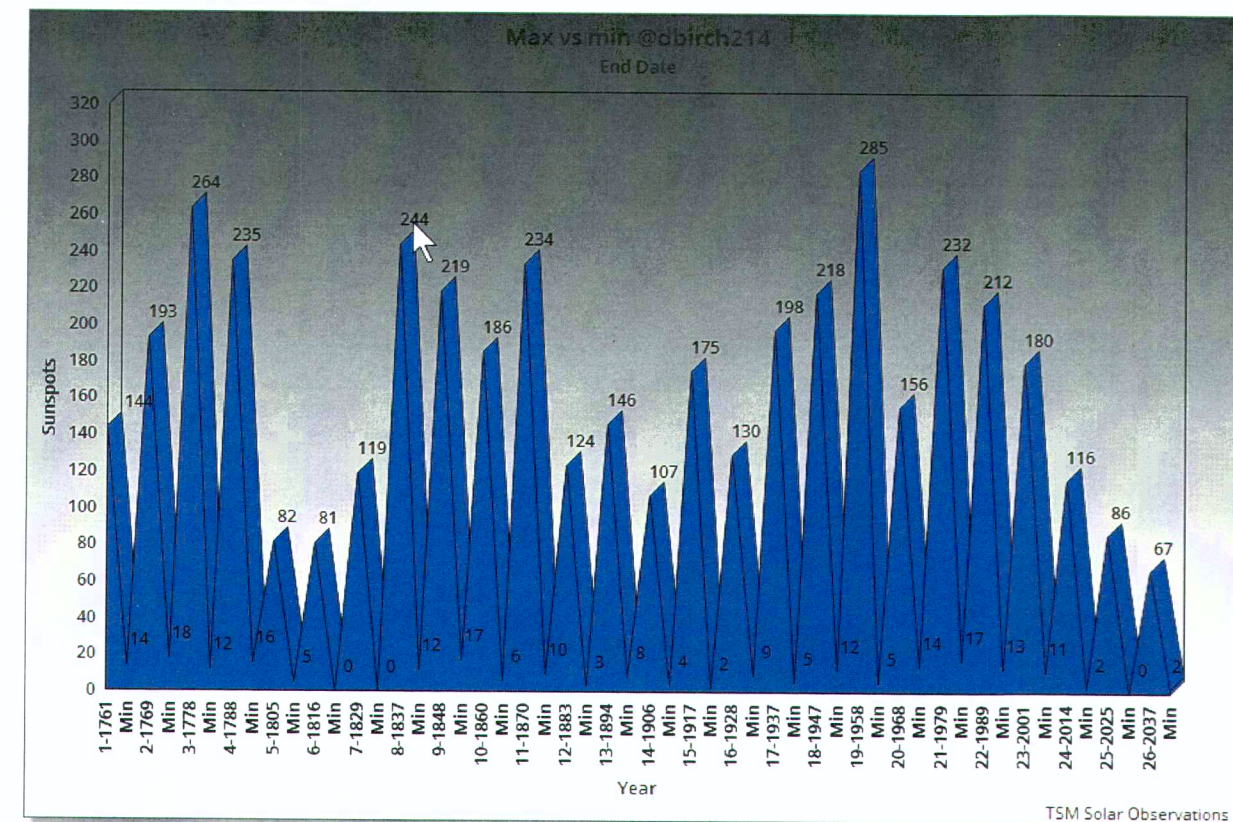
SUNSPOT CYCLES
