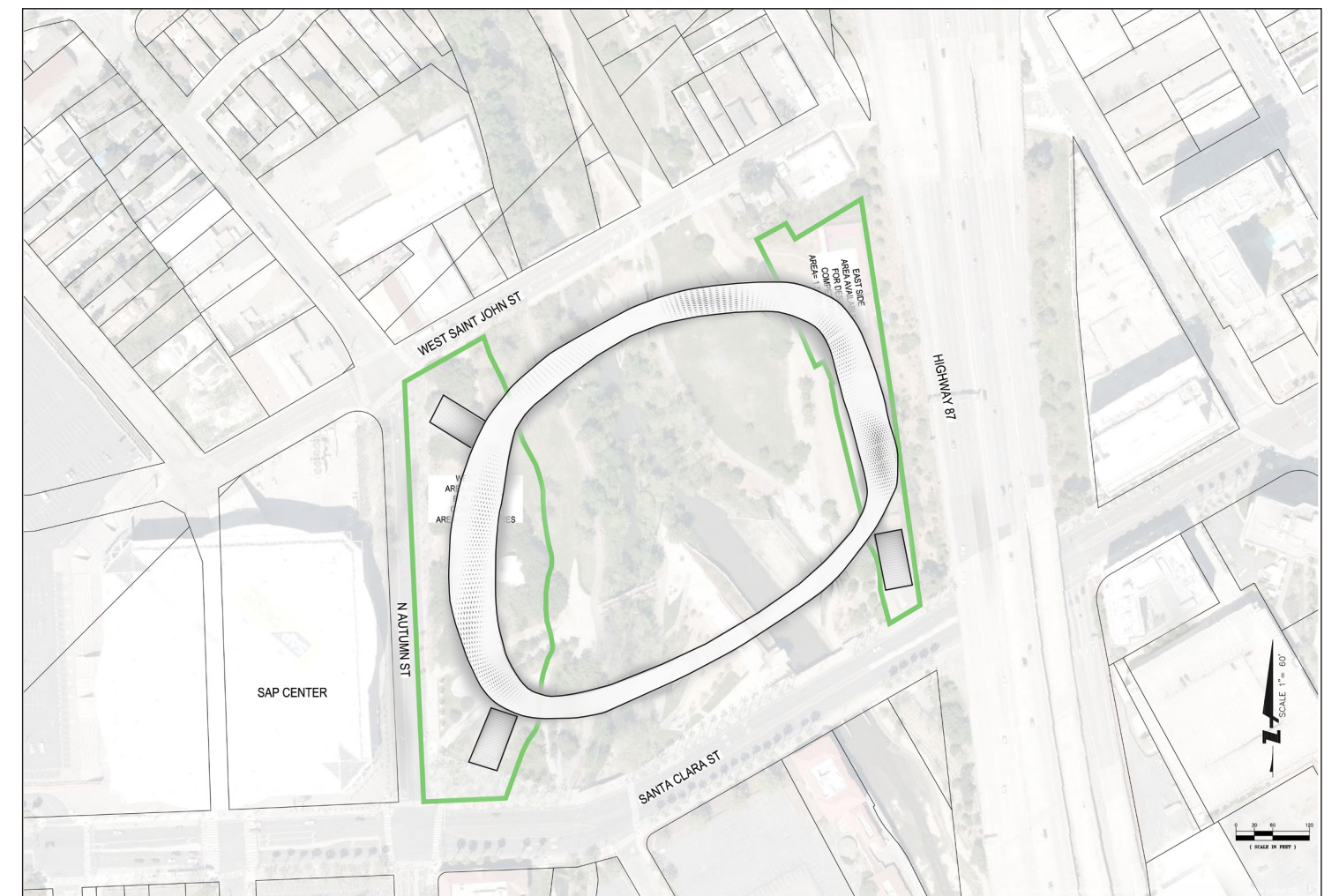
The LOOP Site Plan
