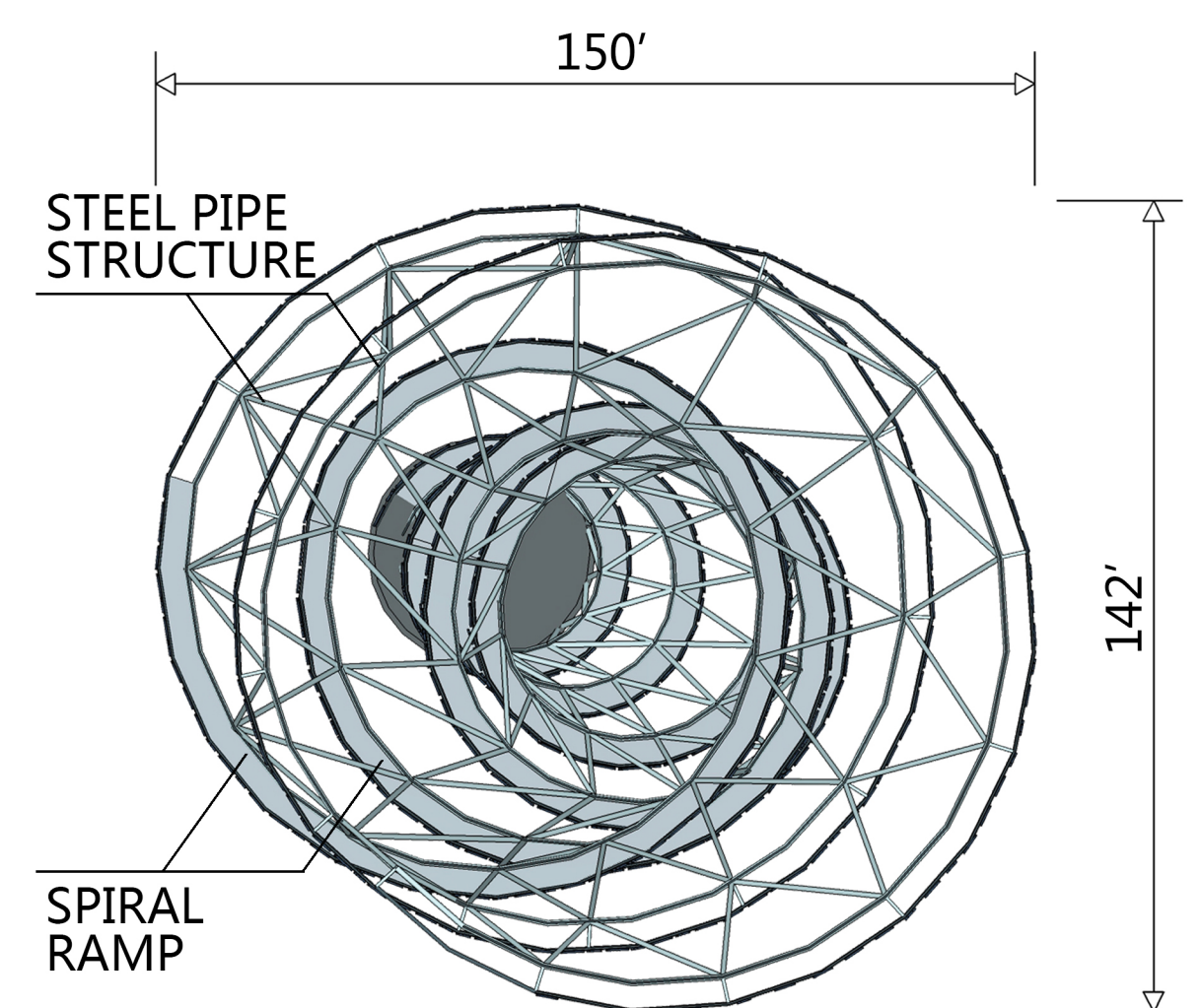
TOP VIEW
