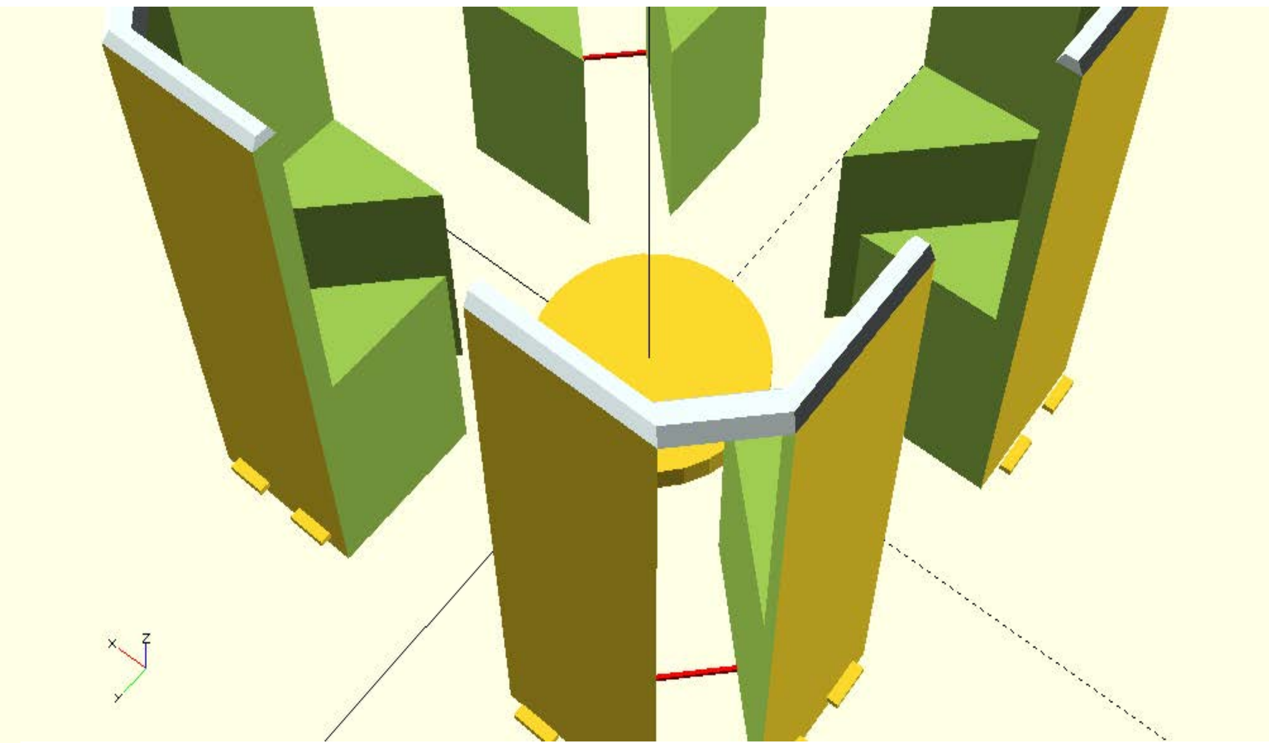
Prisms
