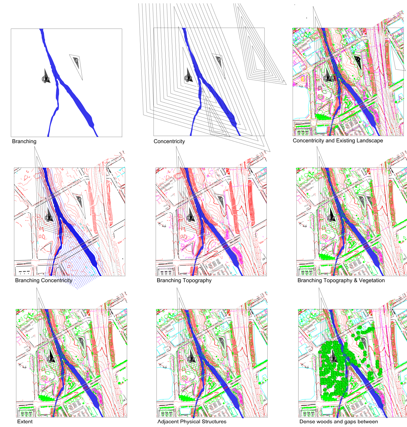
Conceptual Site Plan Studies
