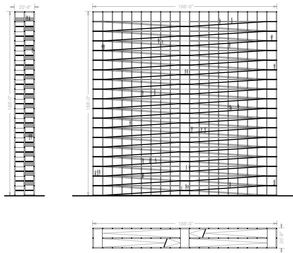
Plan and sections
