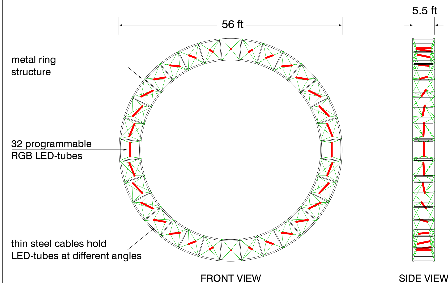
STRUCTURE OF A SINGLE RING
