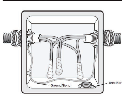
Pigtail Tape Splice
