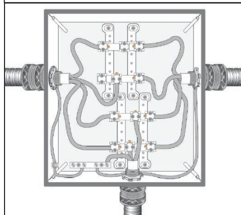
Block Splice
