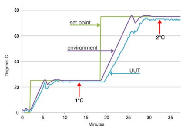
Fig. 2. Environment-control mode results in a 1°C and 2°C UUT temperature offset from set point temperatures at 25°C and at 75°C, respectively.
