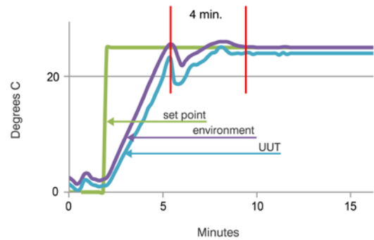
Fig. 1. Time needed for UUT temperature to stabilize after set point is reached using an environment sensor.
