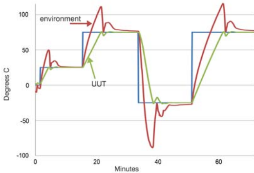
Fig. 3. UUT control results in a significant over or undershoot of environment temperature to bring the device to set point.
