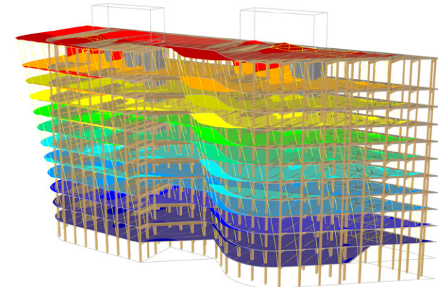
Fig. 41.3 | SMTT | Seismic Loading Lateral Deformation
