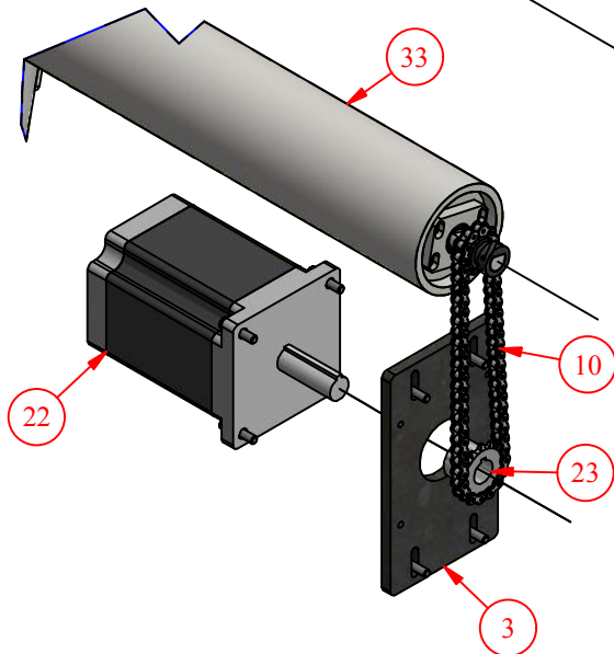
DETAIL B SCALE 1 / 6 LOWER ROLLER DRIVE
