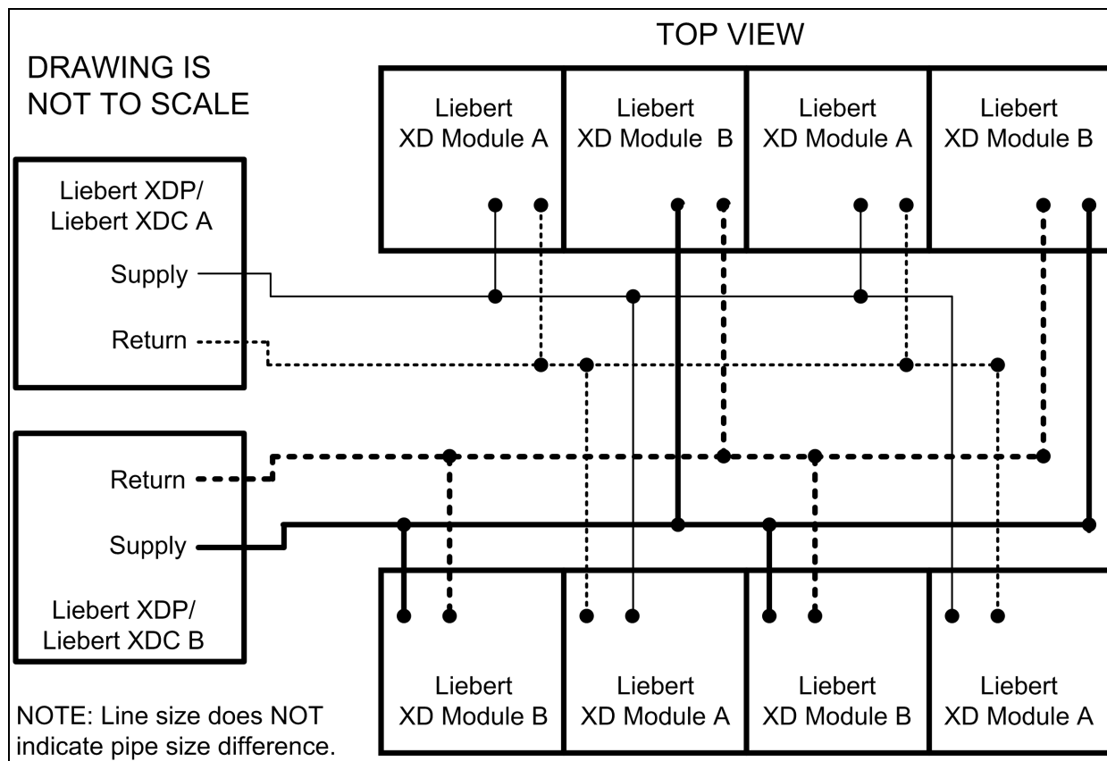
Figure 3.1 Typical Liebert XDR piping—interlaced connections
