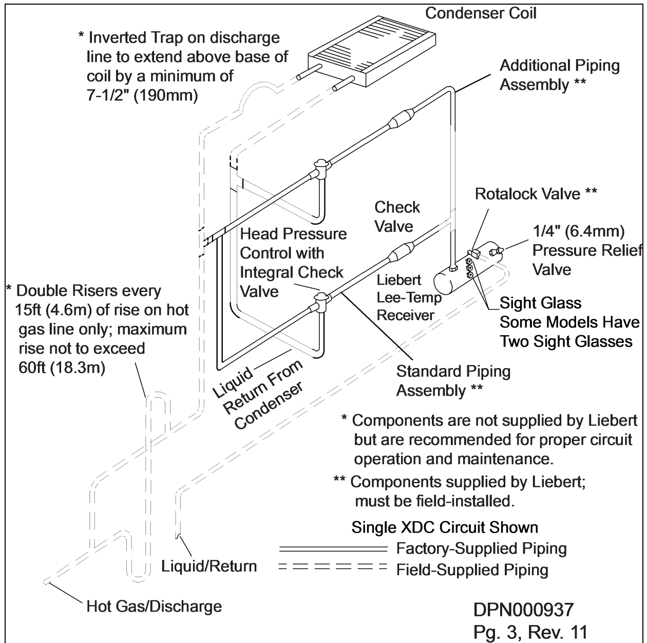
Figure 6.8 General arrangement air-cooled Liebert XDC Liebert Lee-Temp Control
