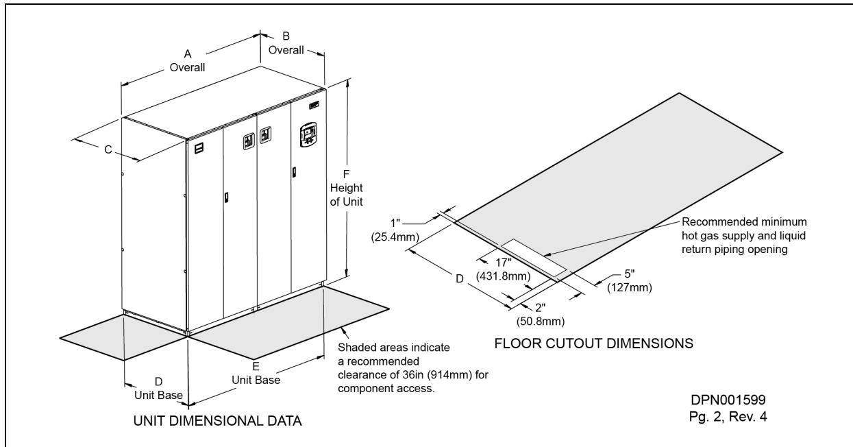
Figure 5.1 Dimensional data
