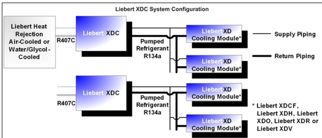
Figure 1.2 Liebert XDC generic piping layout
