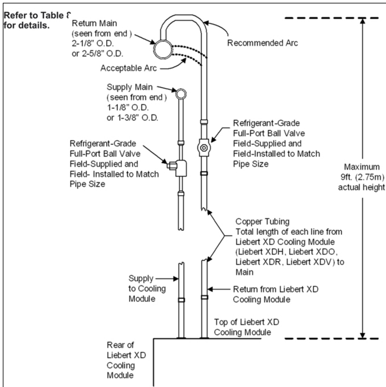
Figure 3.21 Hard-pipe connection diagram for Liebert cooling modules
