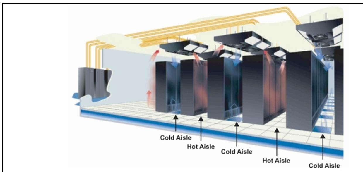
Figure 1.6 Suspended Liebert XDO modules in hot aisle-cold aisle arrangement
