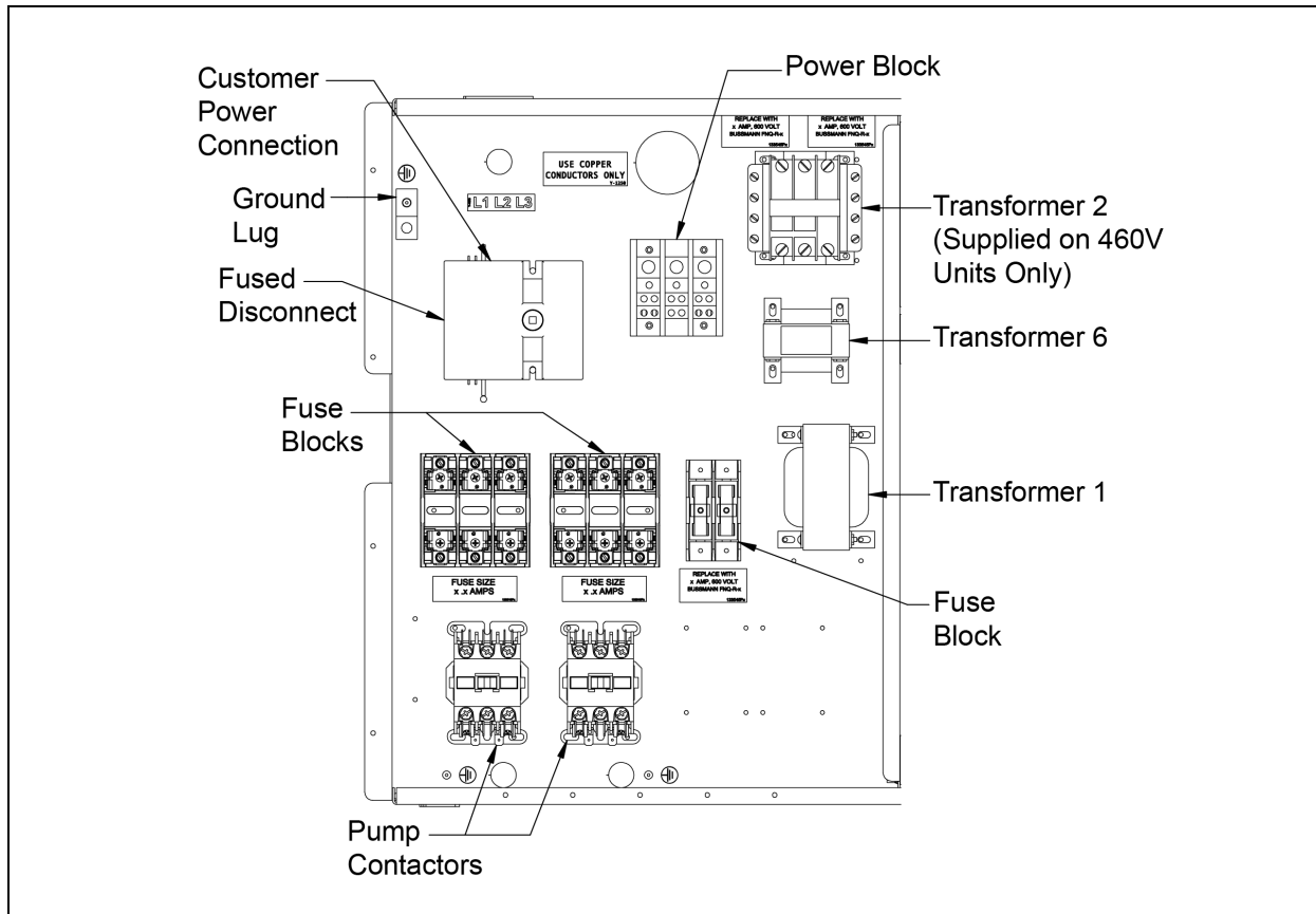
Figure 5.19 Liebert XDP high-voltage connections—60Hz
