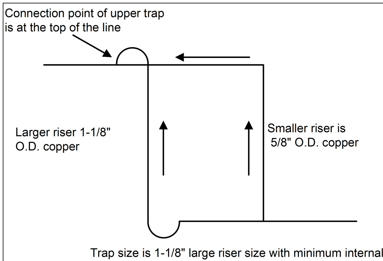
Figure 6.4 Double discharge riser layout
