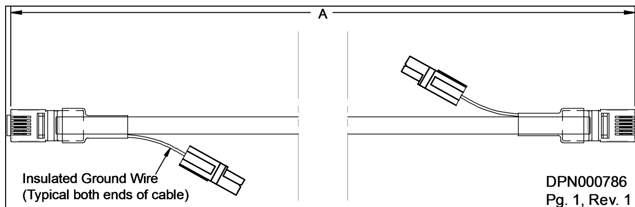
Figure 7.9 CANbus cable
