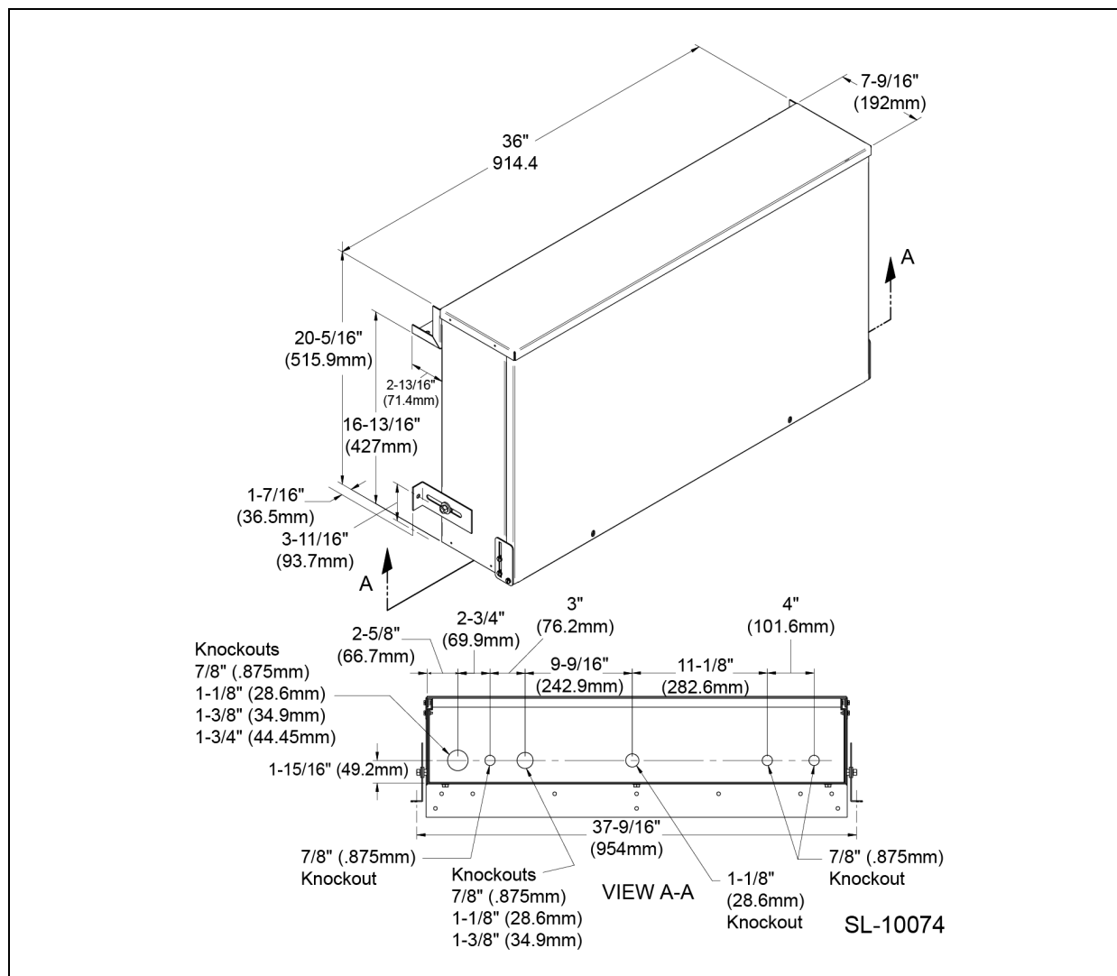
Figure 6.18 Dimensions and knockout sizes, 36-inch models
