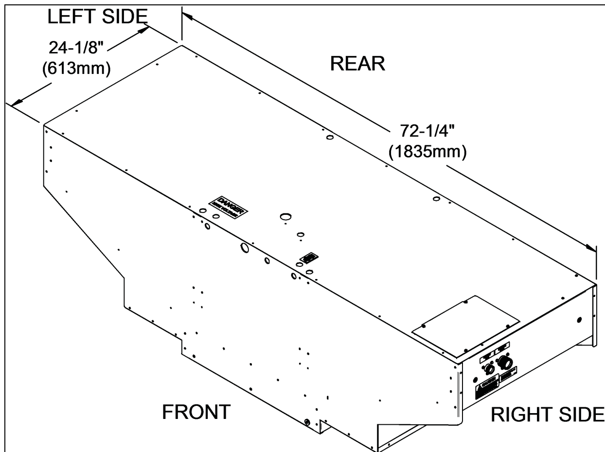
Figure 4.11 Dimensional data—Liebert XDO with pre-charged option
