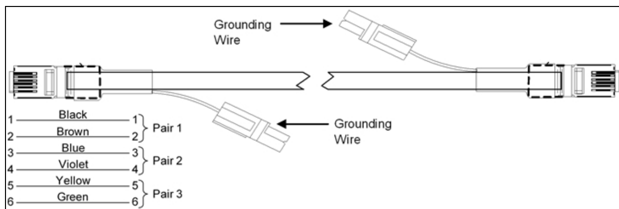
Figure 3.31 CANbus cable wiring
