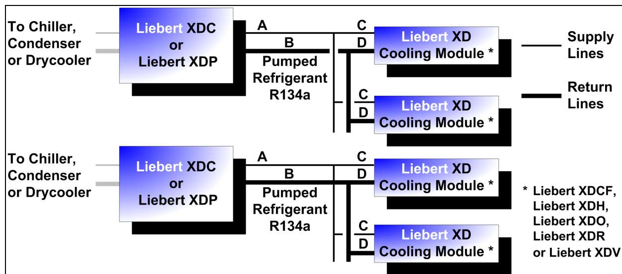
Figure 3.15 Generic piping layout
