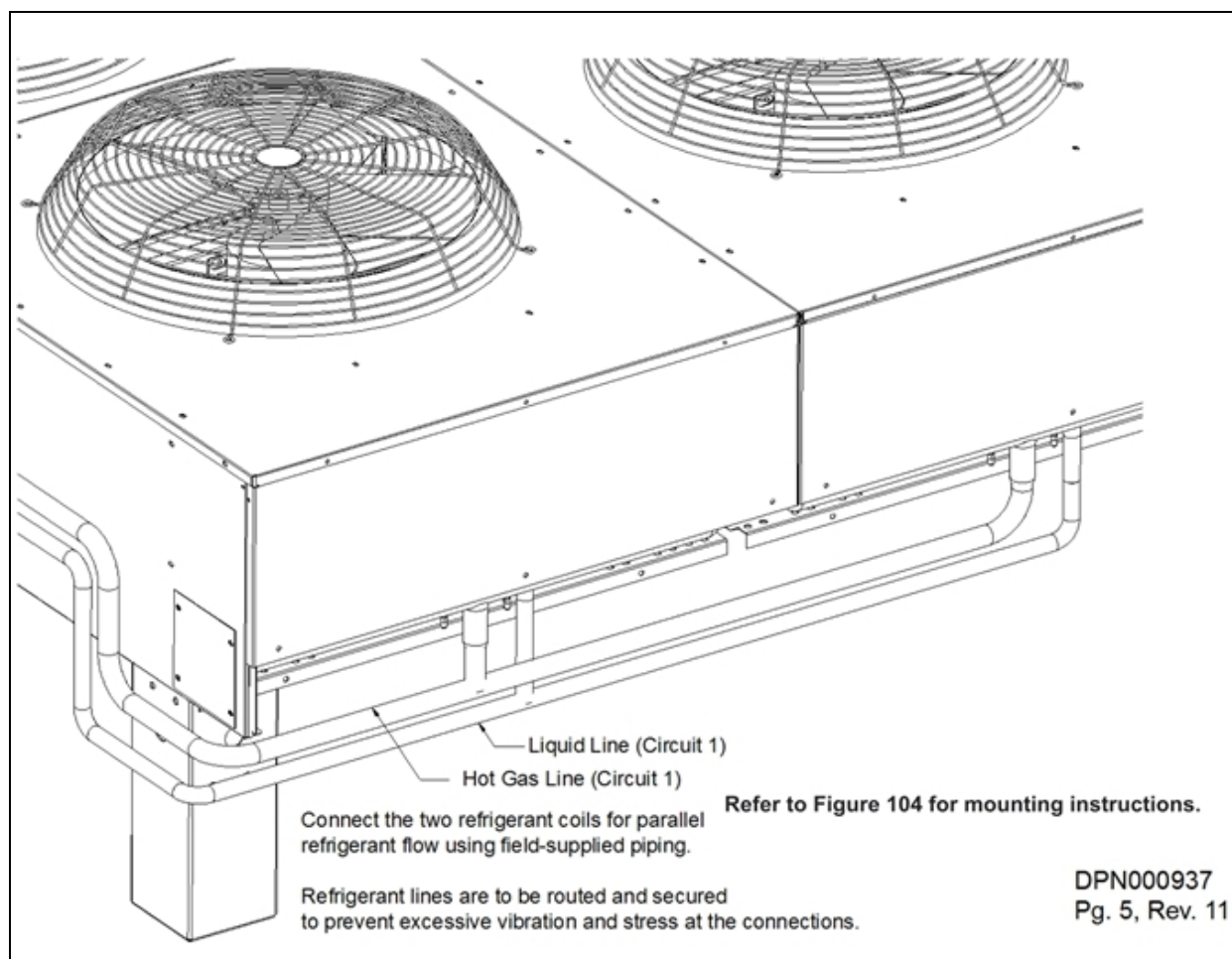
Figure 6.10 DCSL616 piping connections—two refrigerant circuits connected for parallel refrigerant flow
