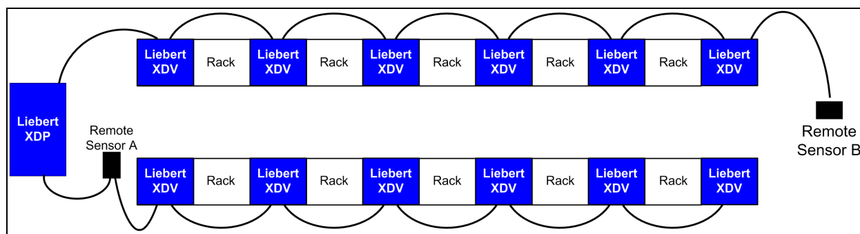
Figure 3.35 Dual daisy chain of Liebert XDV smart modules in CANbus network
