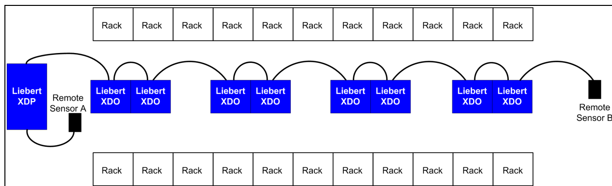
Figure 3.32 Single daisy chain of Liebert XDO smart modules in CANbus network
