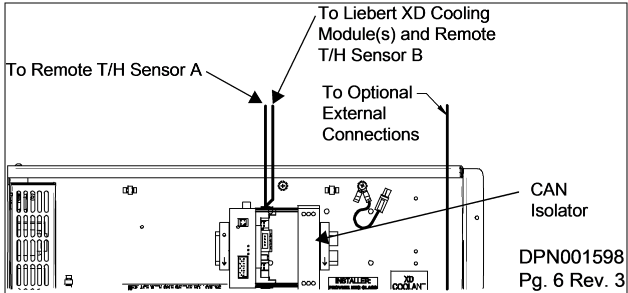
Figure 7.11 CAN Isolator location within the Liebert XDP/XDC
