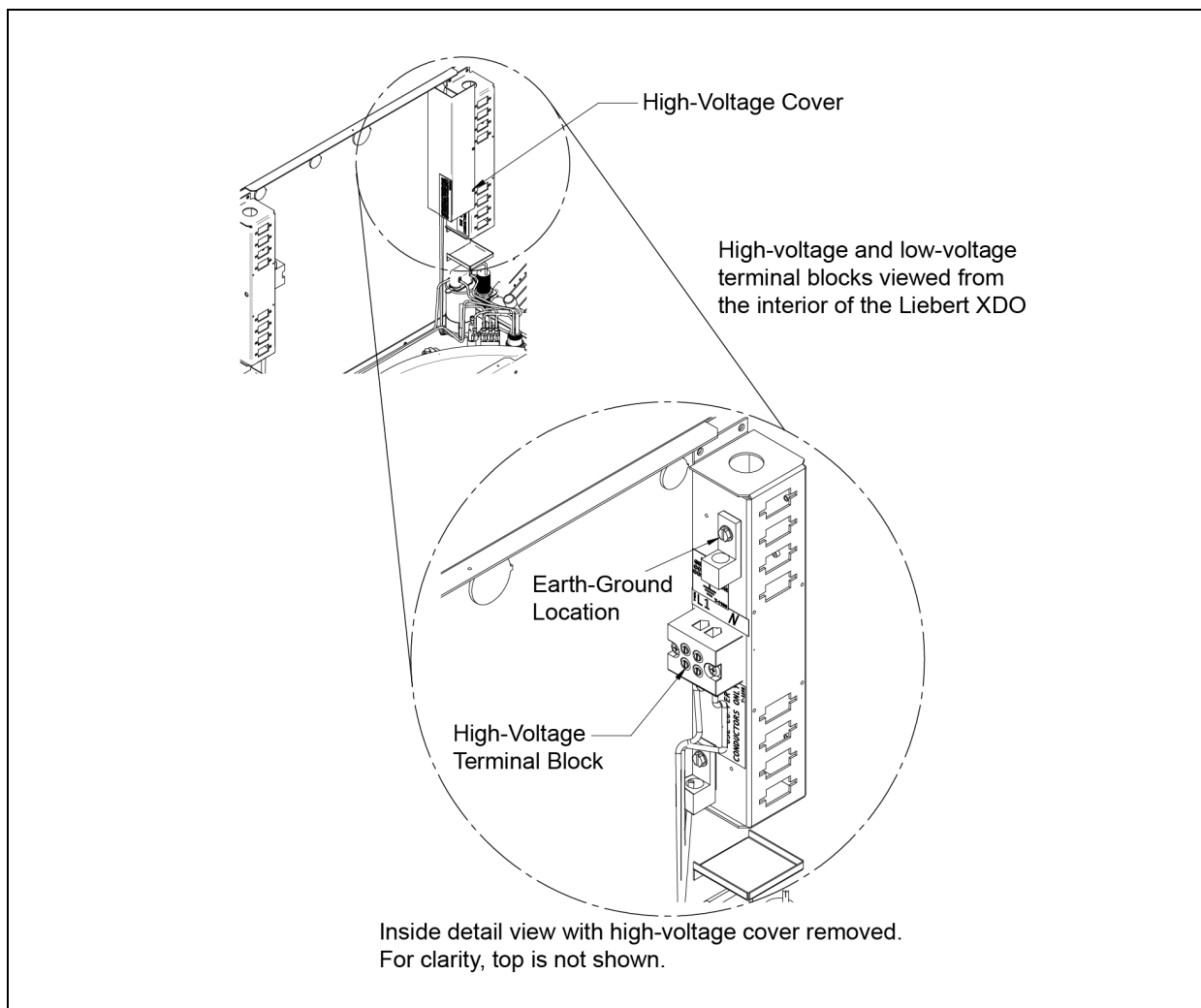
Figure 4.14 High-voltage terminal block and connection locations—standard Liebert XDO modules
