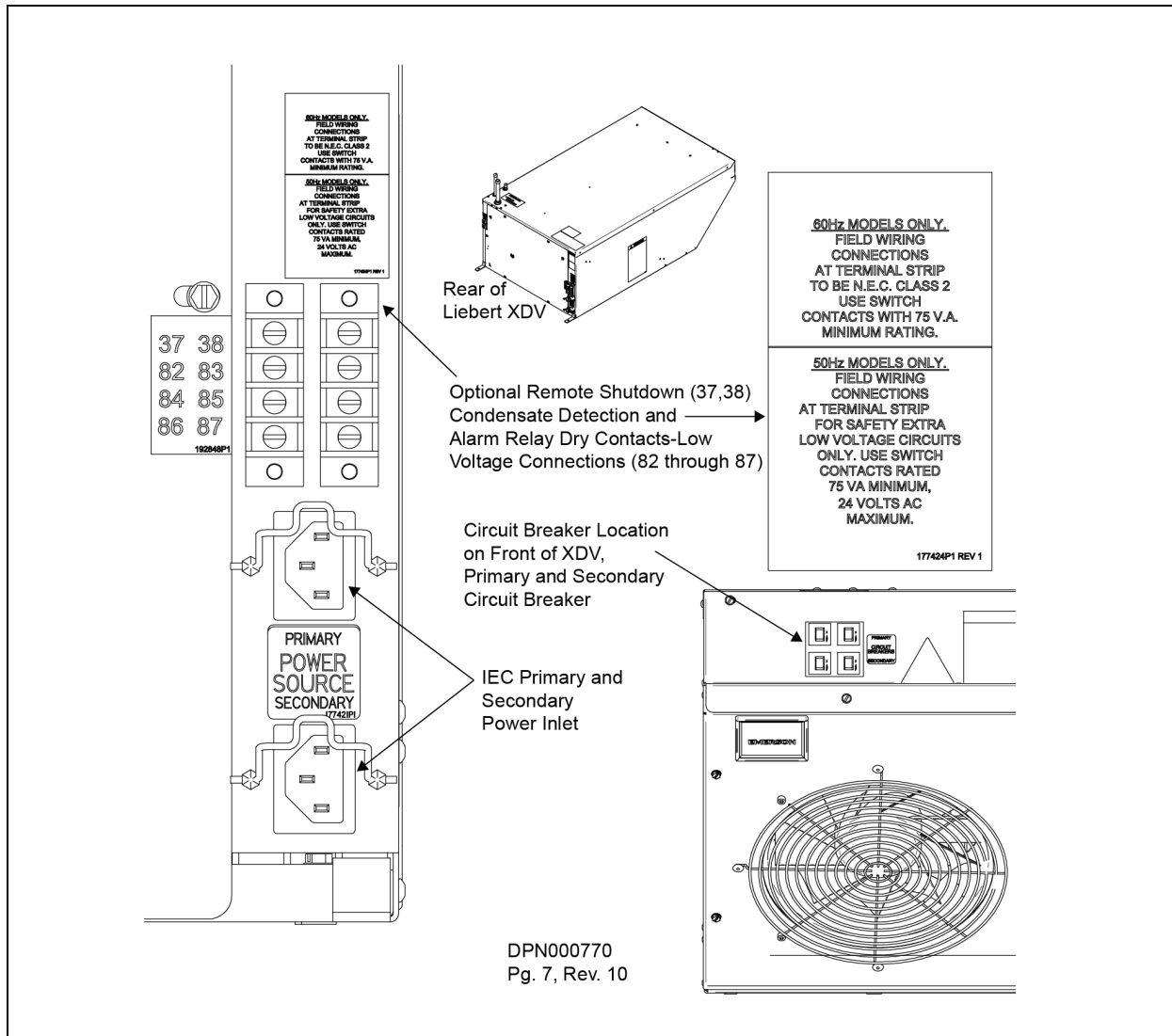
Figure 4.28 Electrical connections for CSA-approved Liebert XDV smart modules
