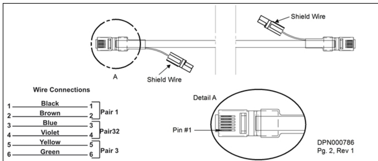
Figure 7.10 CANbus cable plug
