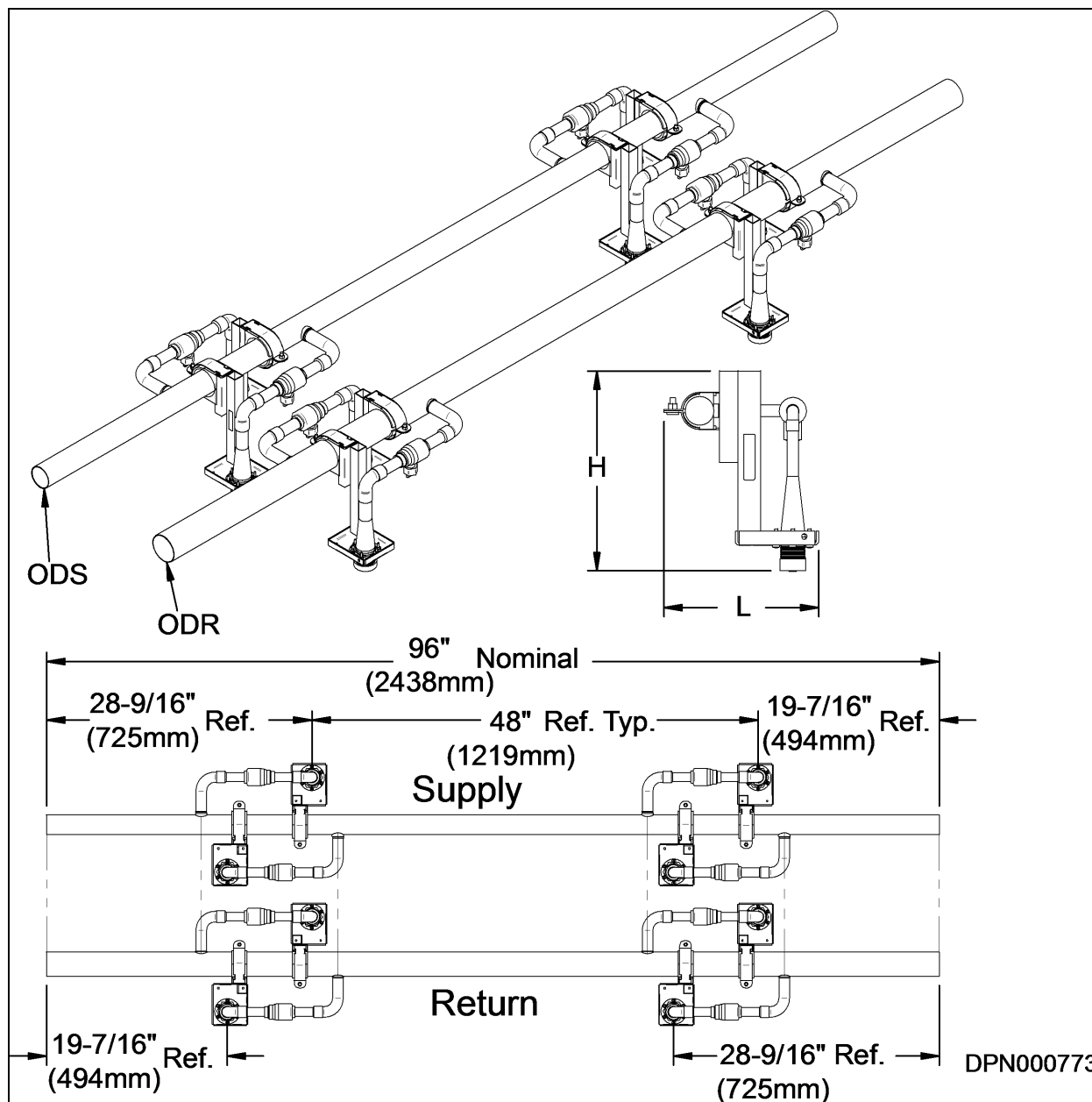
Figure 3.26 Four-port prefabricated piping for Liebert XD cooling modules
