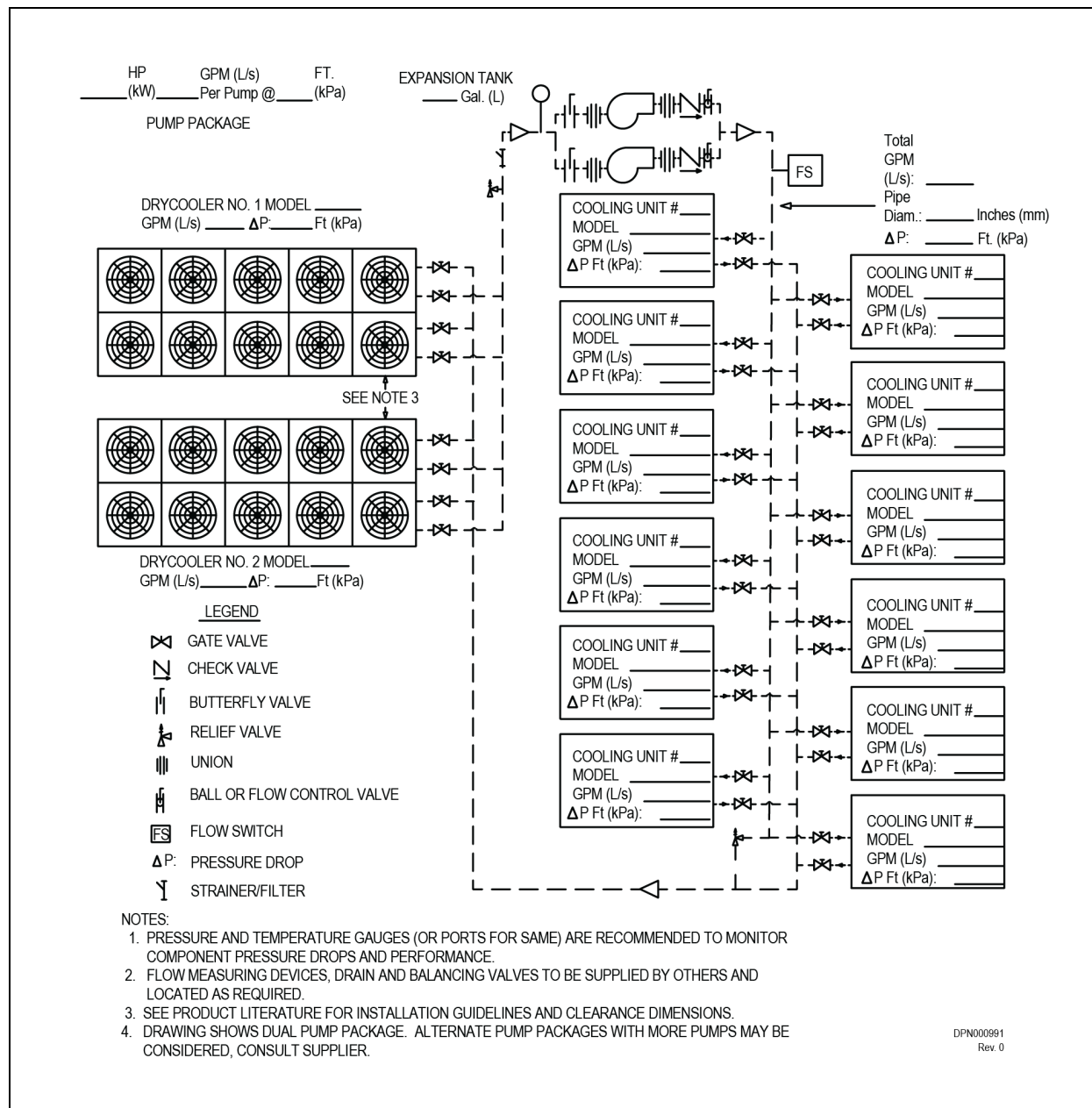
Figure 6.12 Typical piping arrangement for Liebert XDC and two DDNT880A
