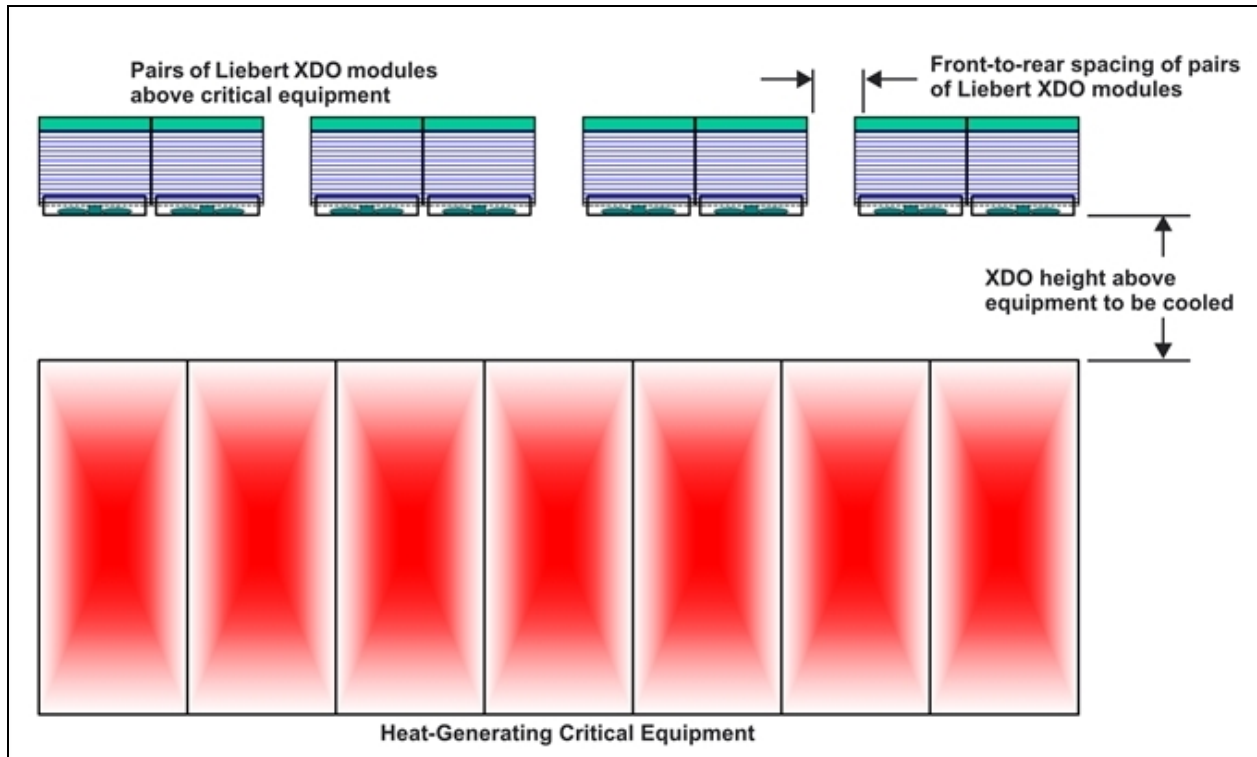
Figure 3.4 Liebert XDO spacing—horizontal (side view)
