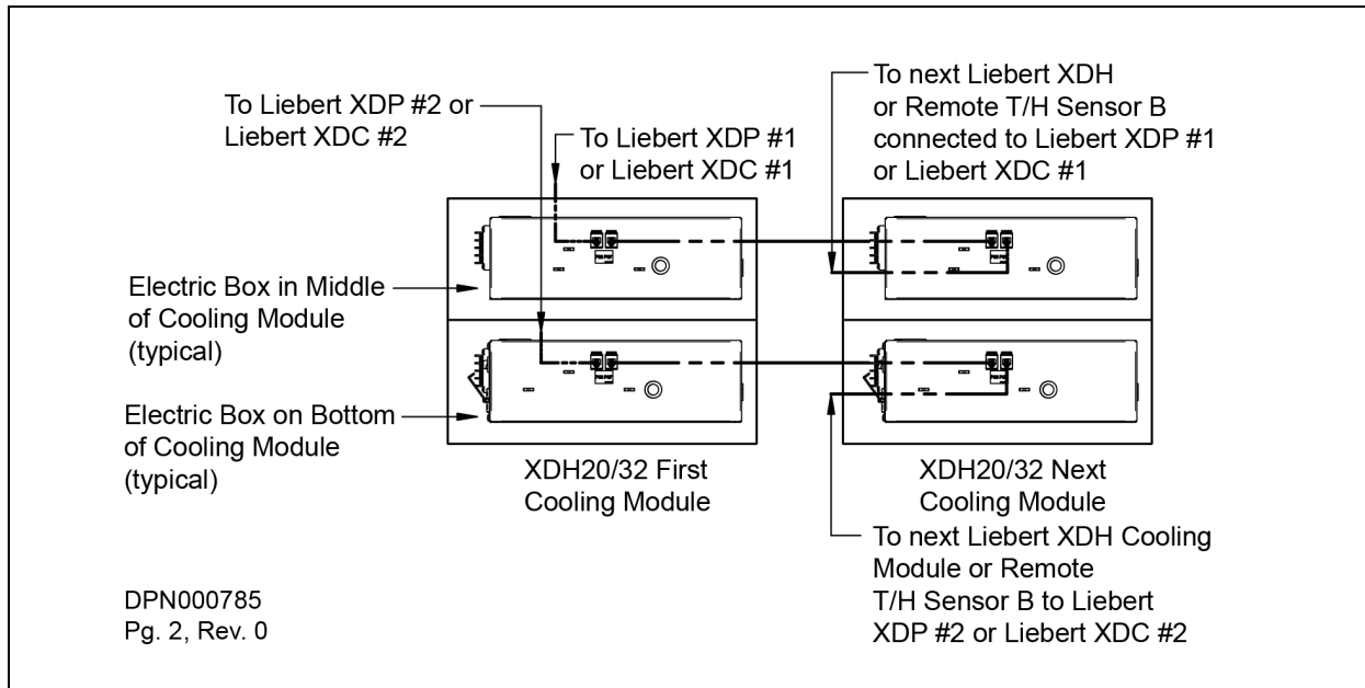
Figure 7.15 Single-circuited Liebert XDHs
