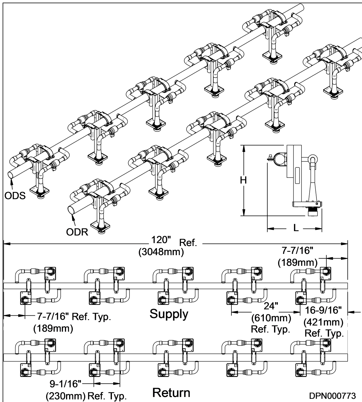
Figure 3.28 Ten-port prefabricated piping for Liebert XD cooling modules
