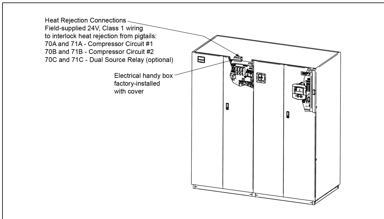
Figure 5.11 Liebert XDC heat rejection electrical connection points
