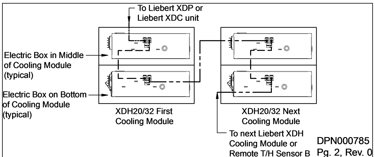
Figure 7.16 Dual-circuited Liebert XDHs
