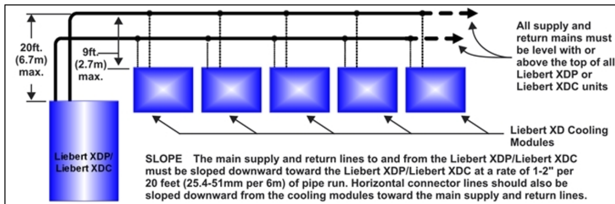
Figure 3.14 Piping for Liebert XDP/Liebert XDC used with Liebert XD cooling modules
