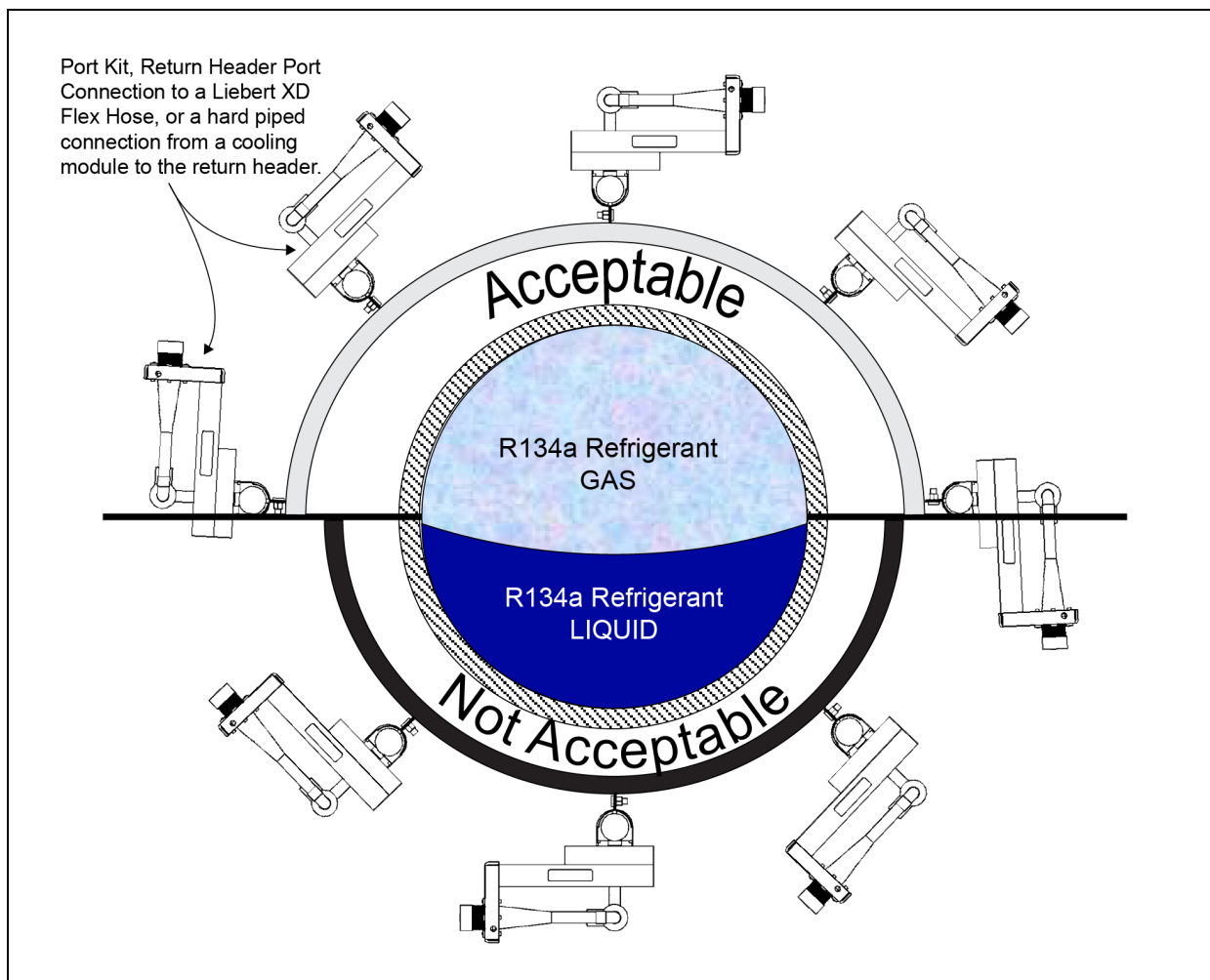
Figure 3.22 Liebert XD return header orientation
