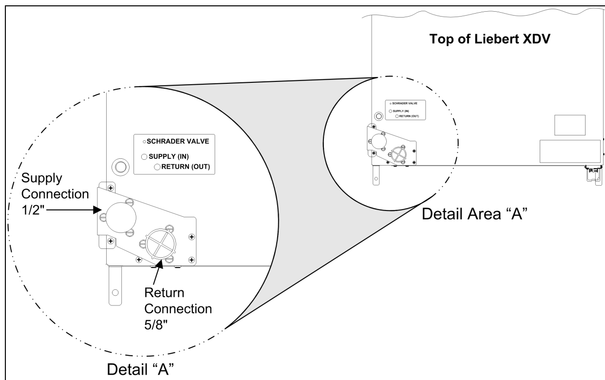
Figure 4.22 Liebert XDV dimensions with one-shot connection
