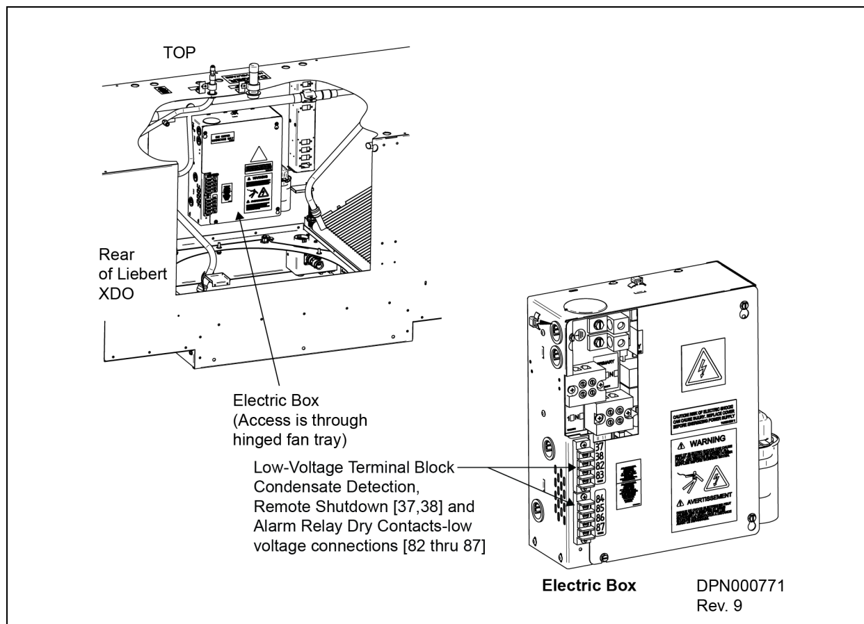
Figure 4.17 Low-voltage wiring—Liebert XDO smart modules
