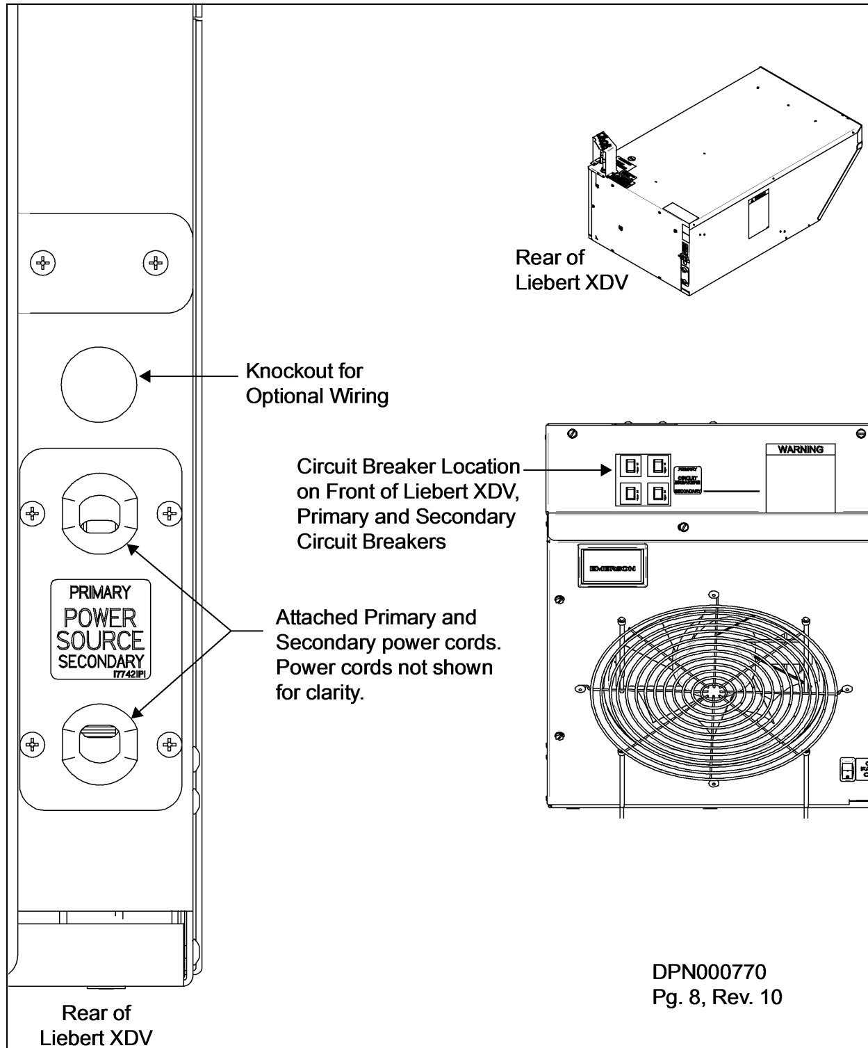
Figure 4.27 Electrical connections for CE-approved Liebert XDV basic modules
