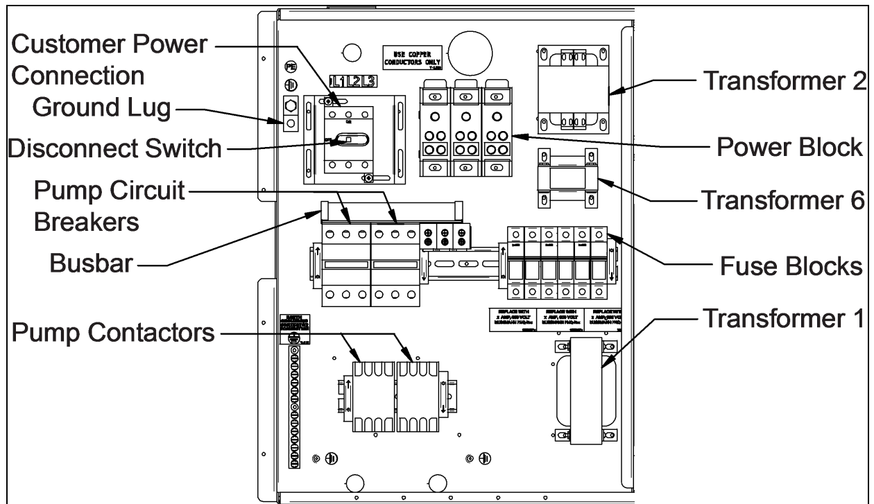
Figure 5.20 Liebert XDP high-voltage connections—50Hz
