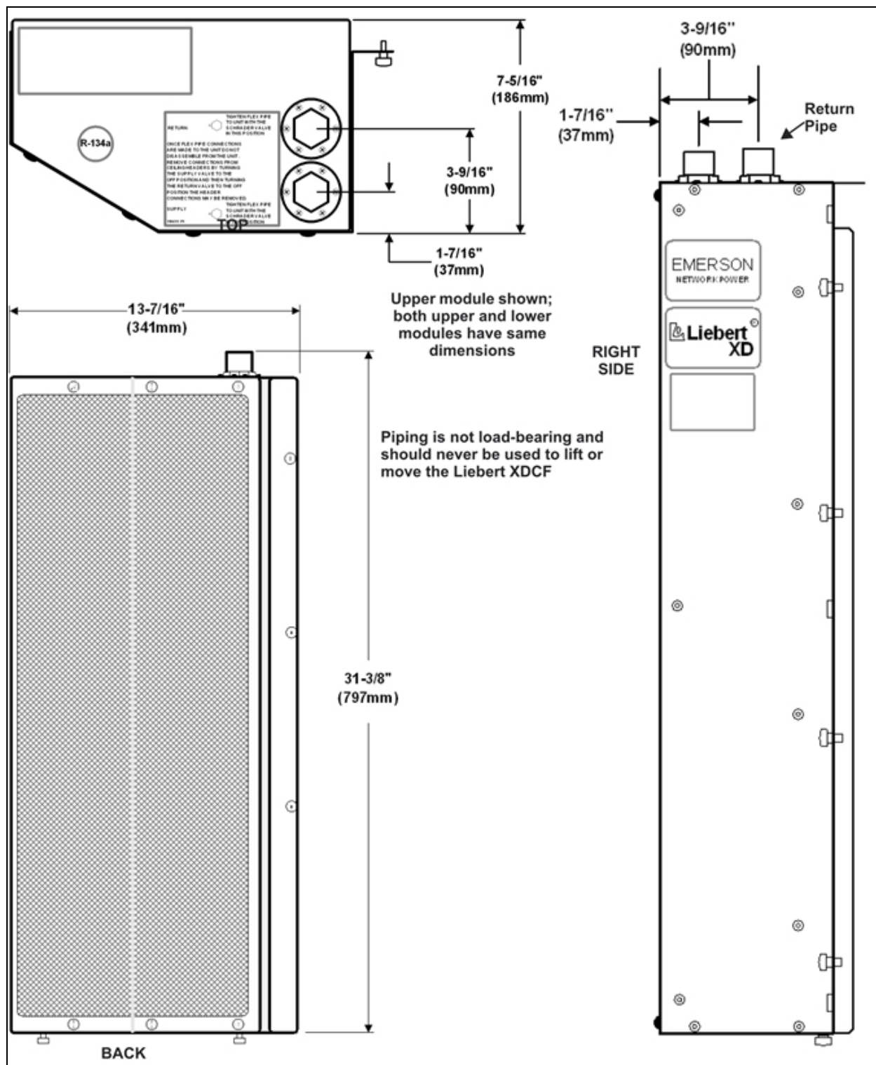
Figure 4.2 Overall dimensions
