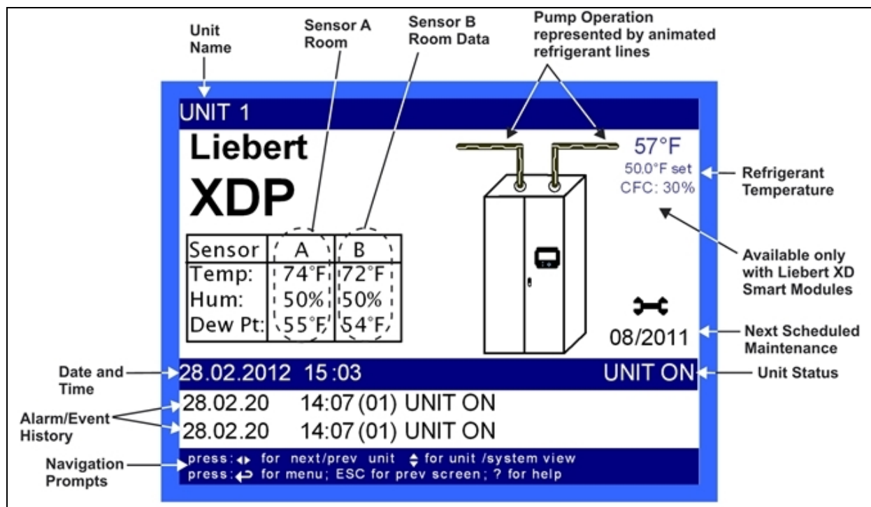
Figure 7.3 Liebert iCOM default home screen for Liebert XDP
