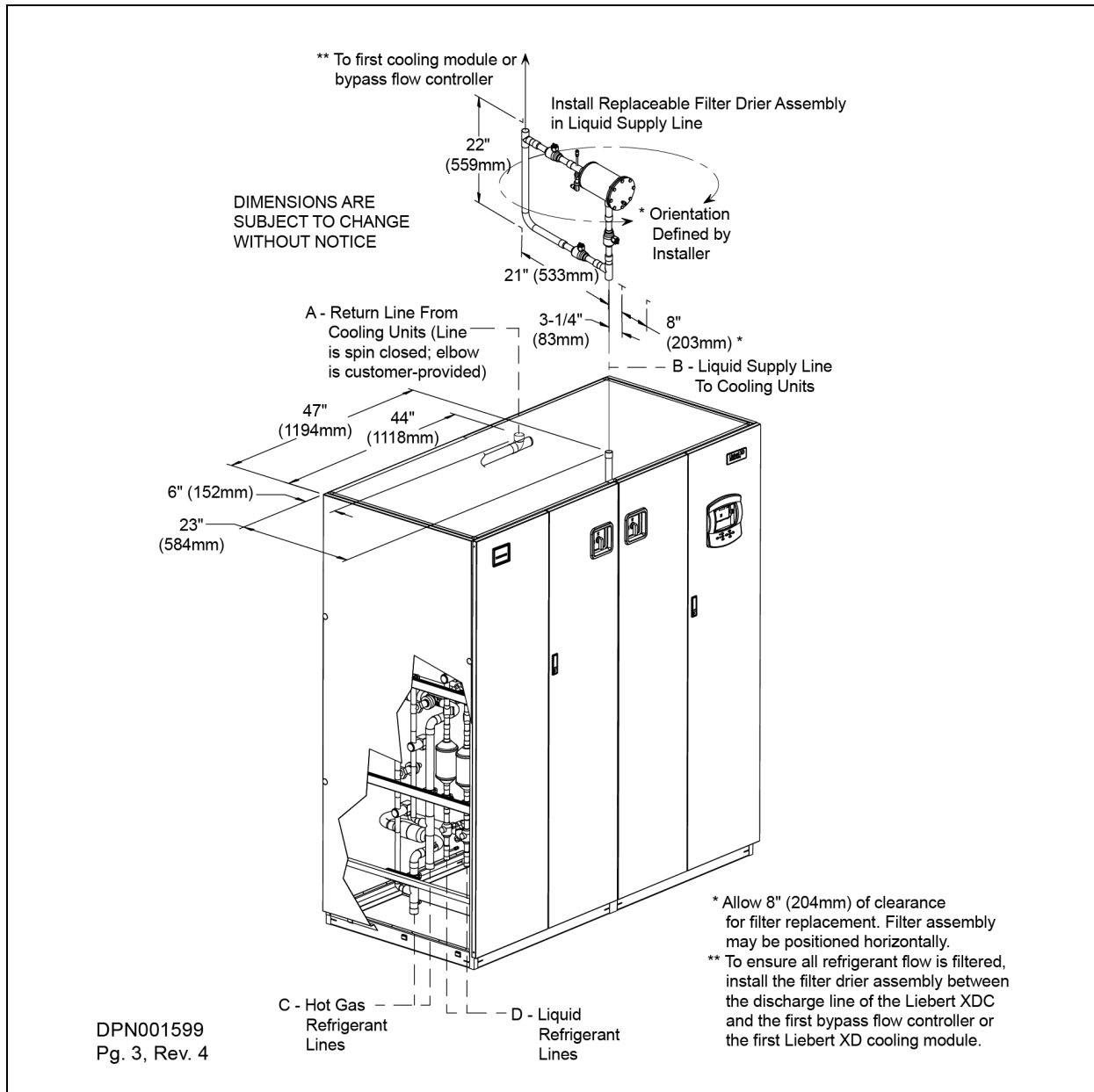
Figure 5.2 Piping locations
