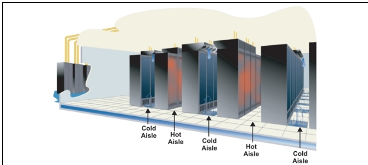
Figure 1.9 Top-mounted Liebert XDV modules with Liebert Flex Pipe in hot aisle-cold aisle arrangement
