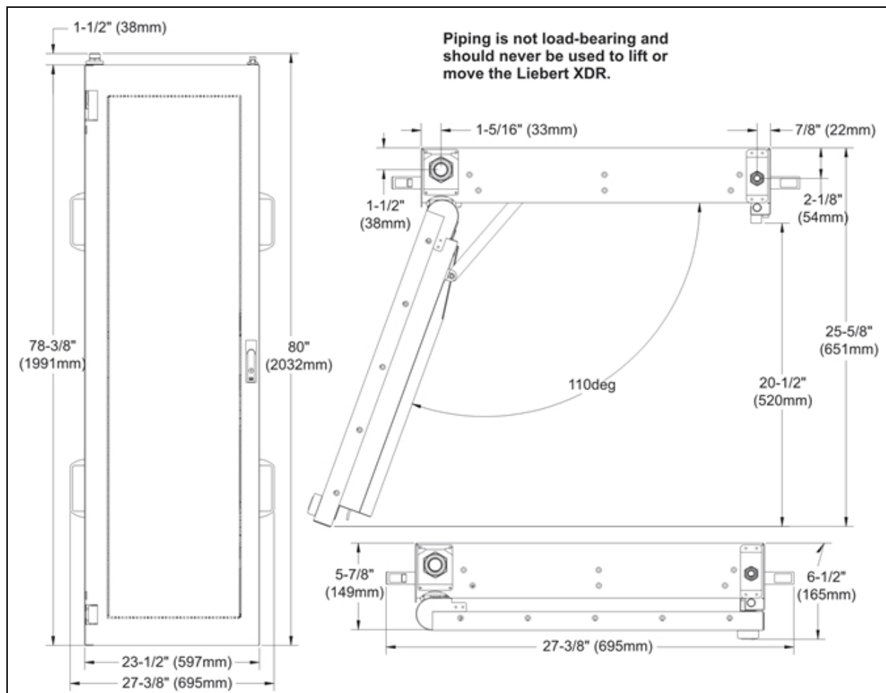
Figure 4.20 Liebert XDR dimensions with removable connections
