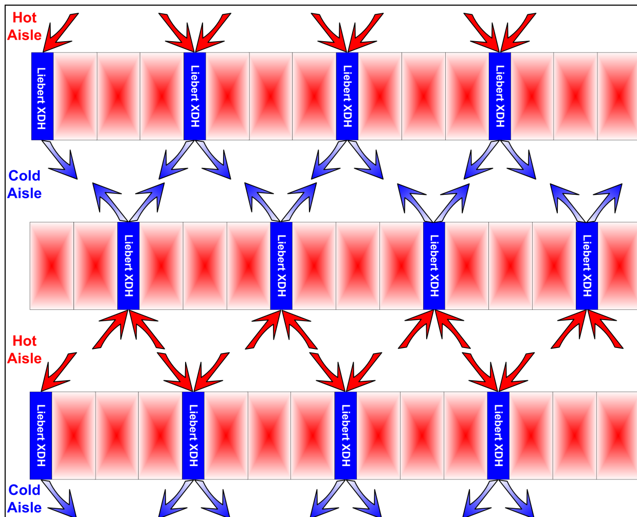
Figure 3.3 Liebert XDH placement (top view)
