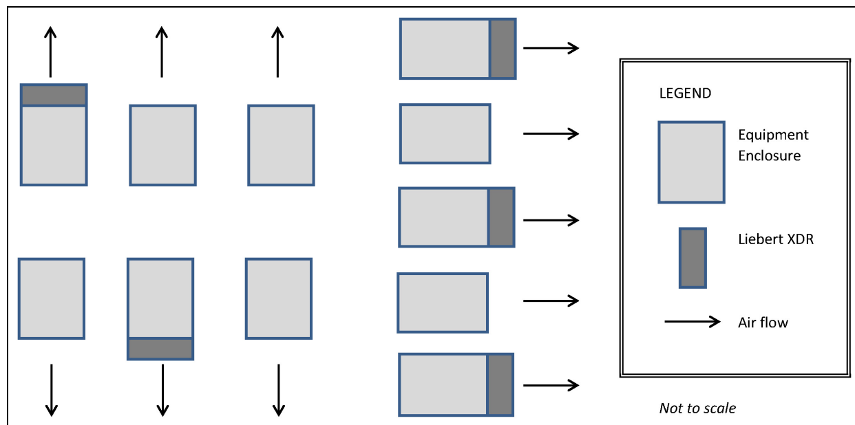
Figure 3.13 Liebert XD modules not in hot aisle/cold aisle configuration
