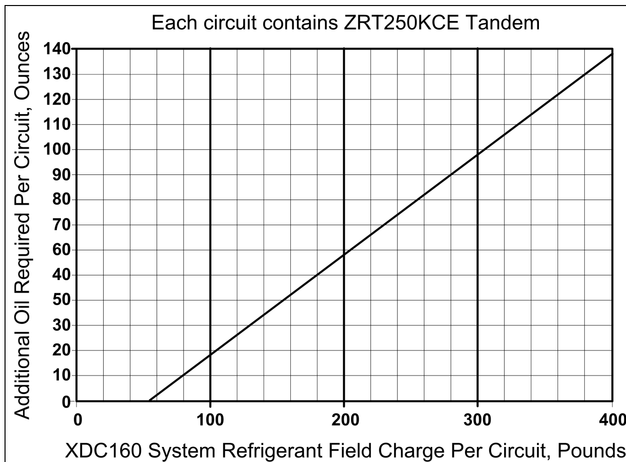
Figure 6.11 Additional oil requirements for refrigerant charge
