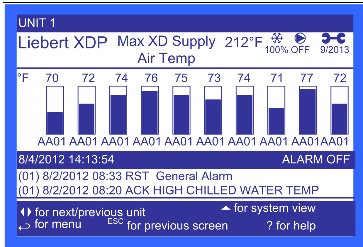
Figure 7.4 Cooling module overview
