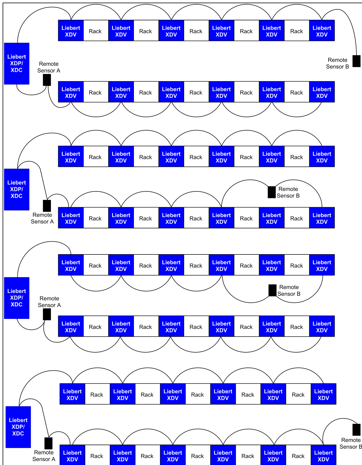
Figure 7.8 Modules on two chains
