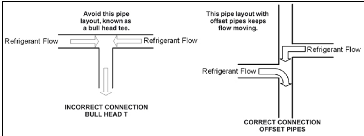
Figure 3.24 Efficient piping layout—avoid “bull head T” connections
