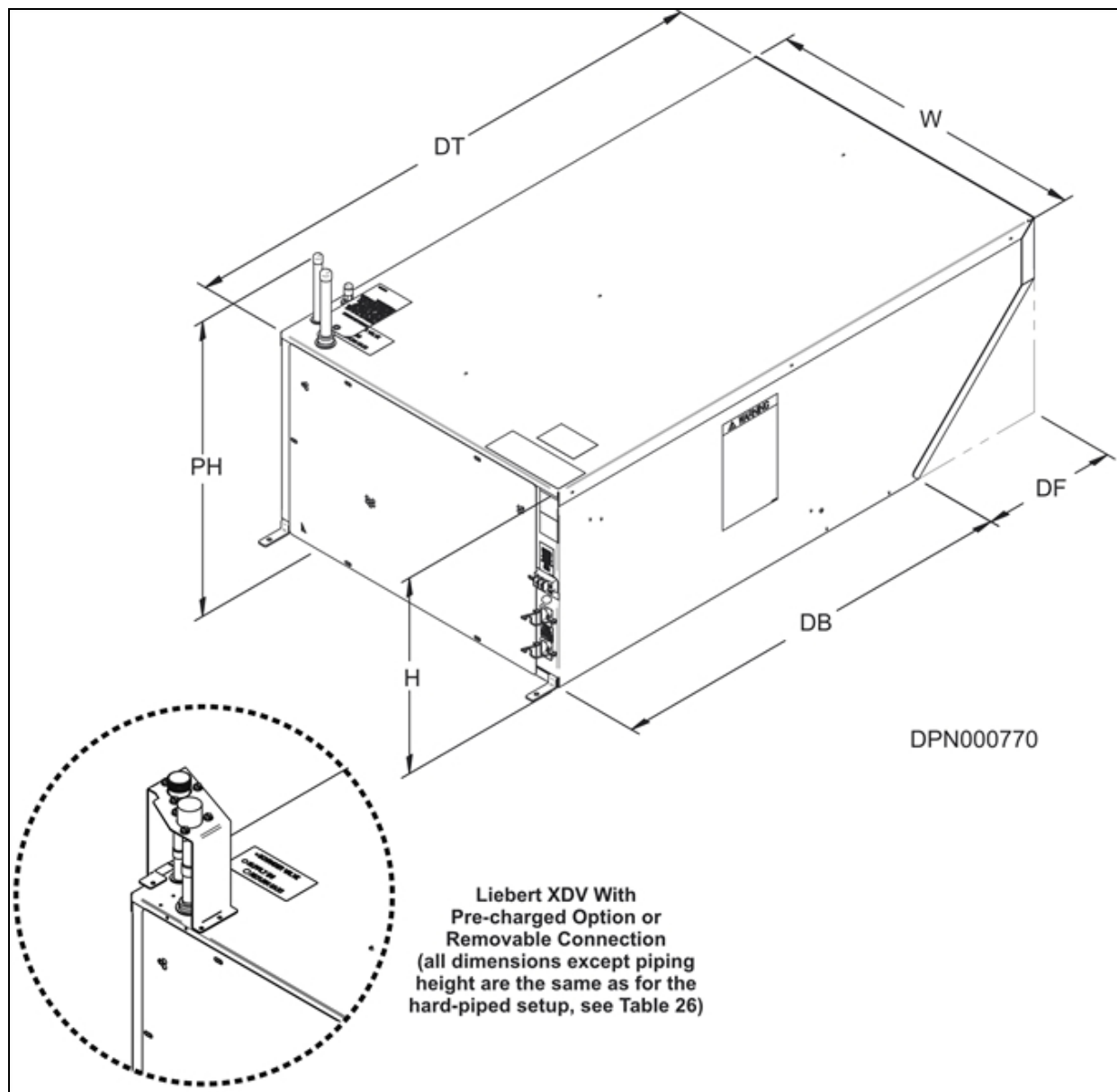
Figure 4.21 Liebert XDV dimensions
