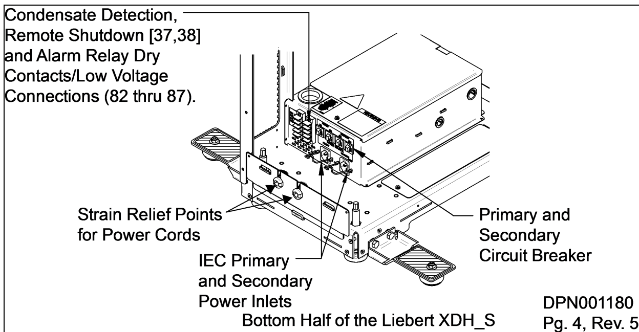
Figure 4.8 Smart Liebert XDH electrical connections
