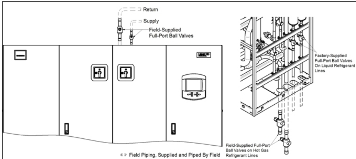
Figure 3.19 General piping details
