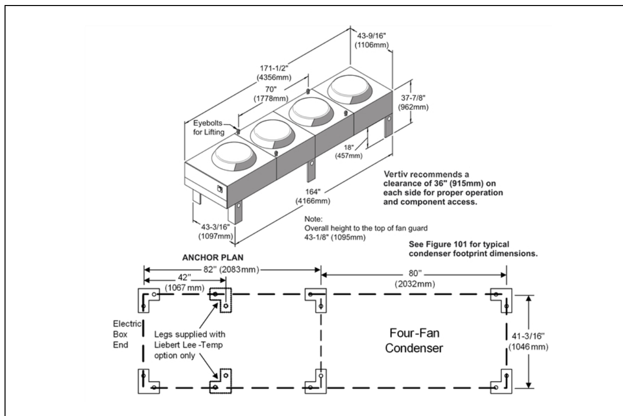
Figure 6.1 Condenser planning dimensional data—Four-fan units
