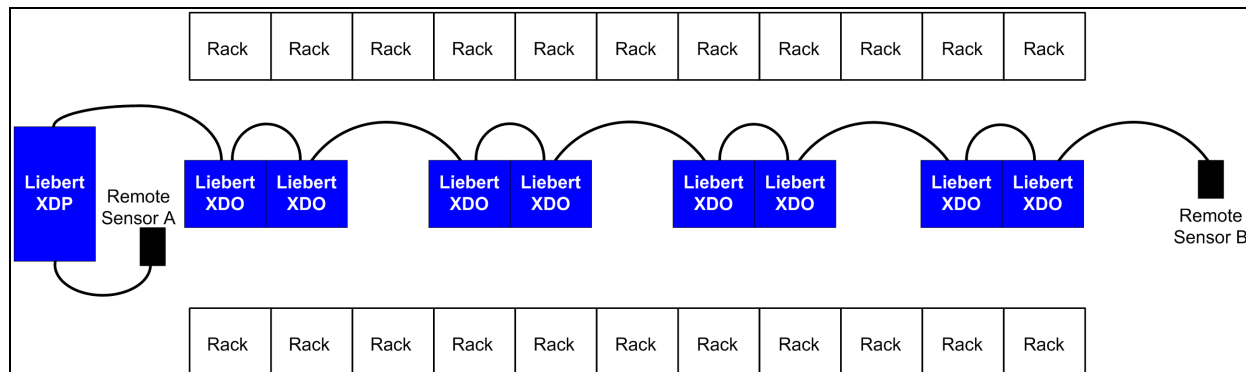
Figure 3.33 Sensor at the end of daisy chain of Liebert XDO smart modules in CANbus network
