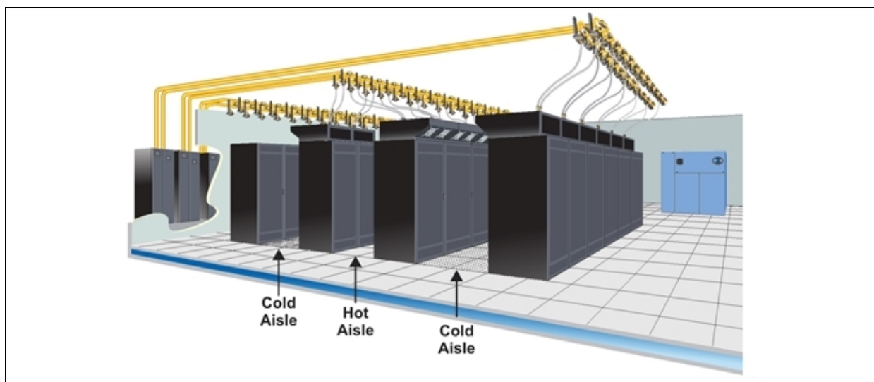
Figure 1.9 Top-mounted Liebert XDV modules with Liebert Flex Pipe in hot aisle-cold aisle arrangement
