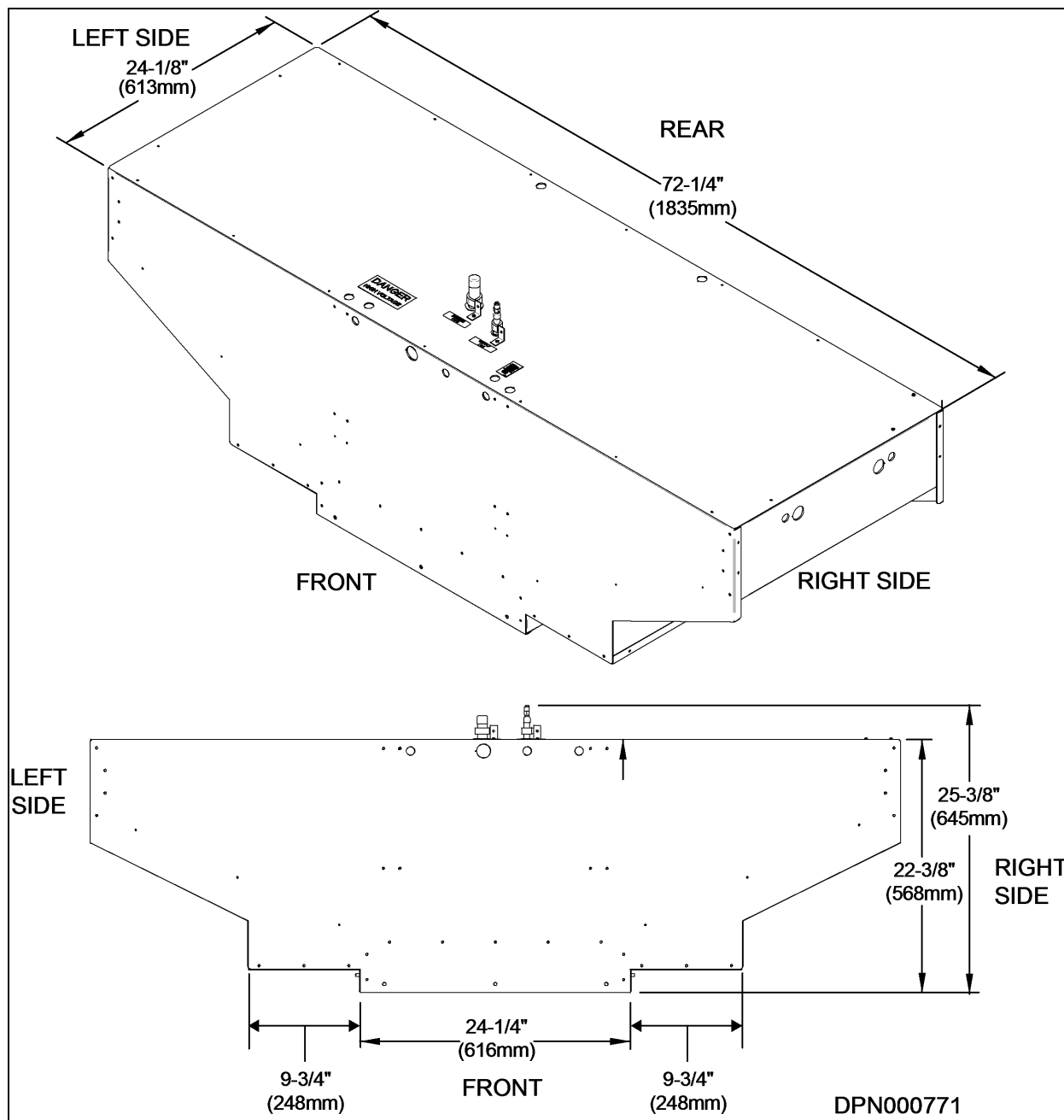
Figure 4.10 Dimensional data—Liebert XDO hard-piped modules
