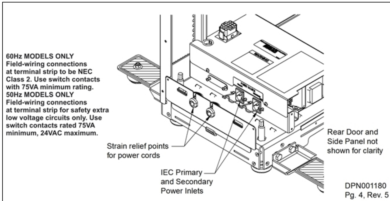
Figure 4.8 Smart Liebert XDH electrical connections
