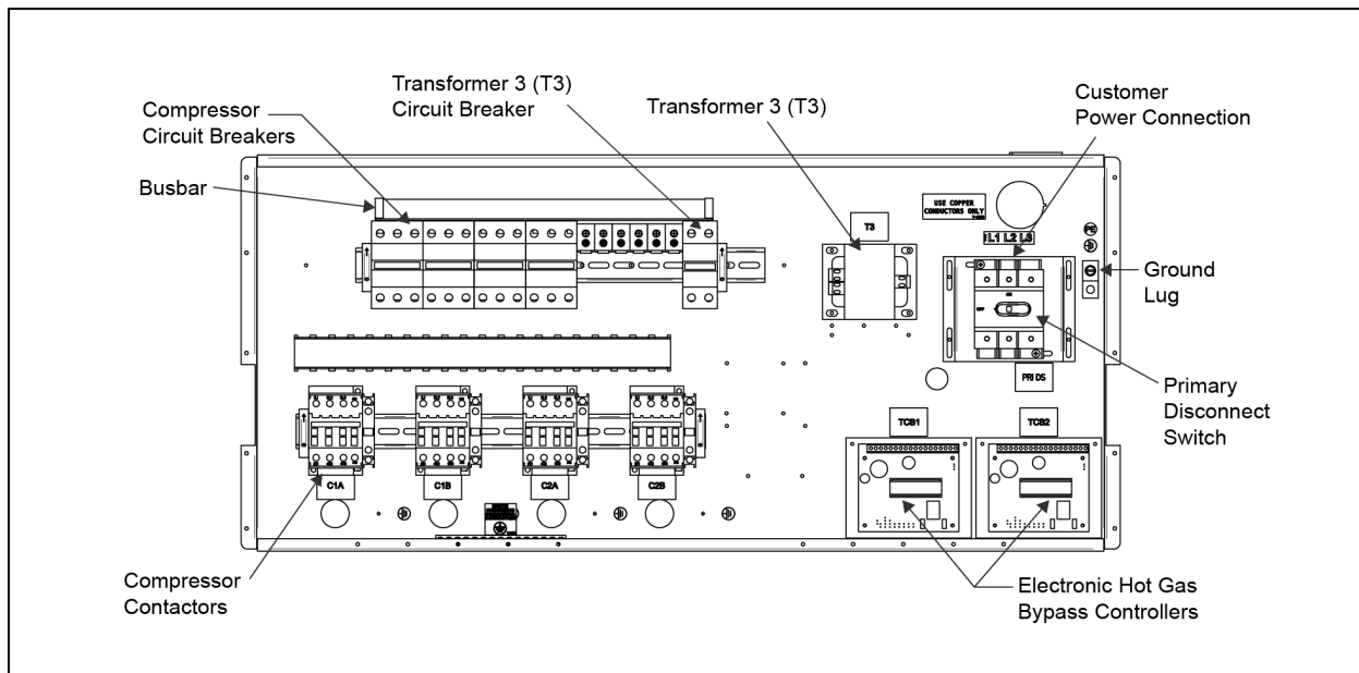
Figure 5.8 Liebert XDC high-voltage connections—primary disconnect switch, 50Hz models
