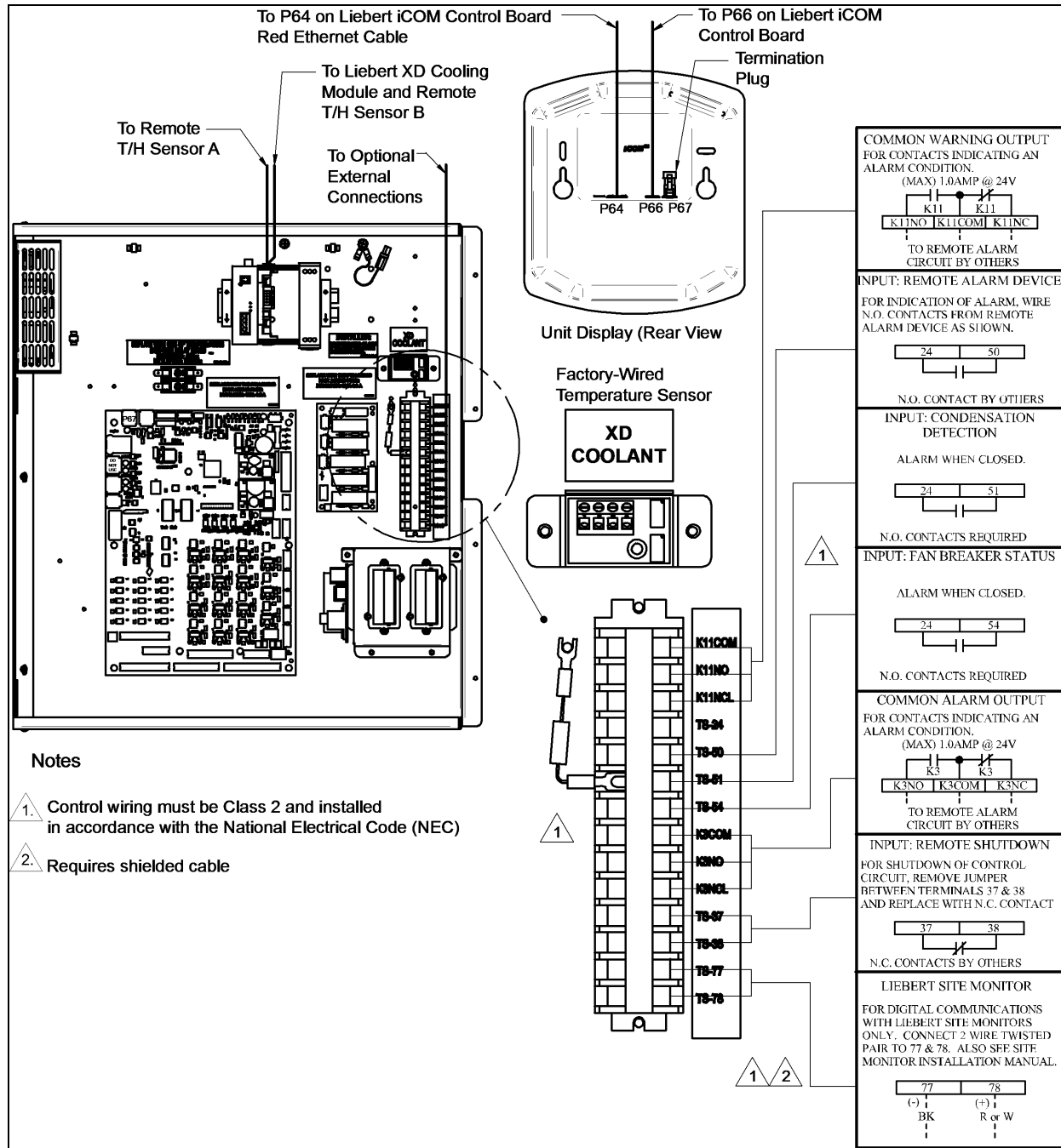
Figure 5.13 Liebert XDC Extra Low Voltage field connection points
