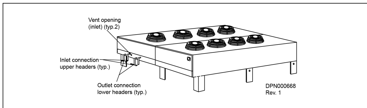
Figure 6.15 Piping connections for 8-fan drycoolers
