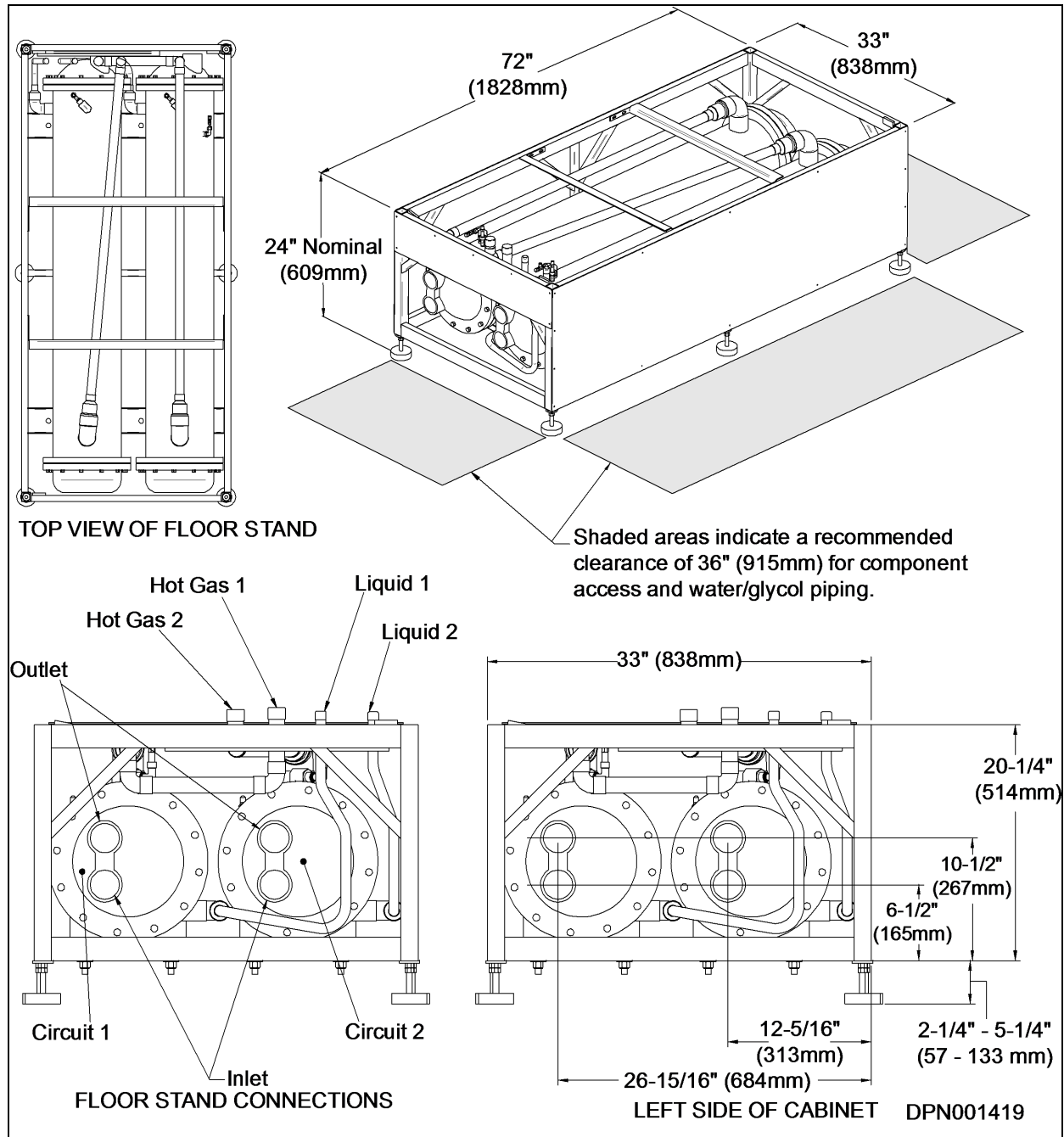
Figure 5.4 Piping locations—floor stand and valve assembly
