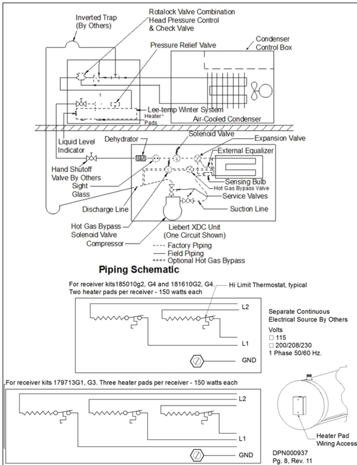
Figure 6.7 Liebert XDC piping schematic and Liebert Lee-Temp heater pad wiring
