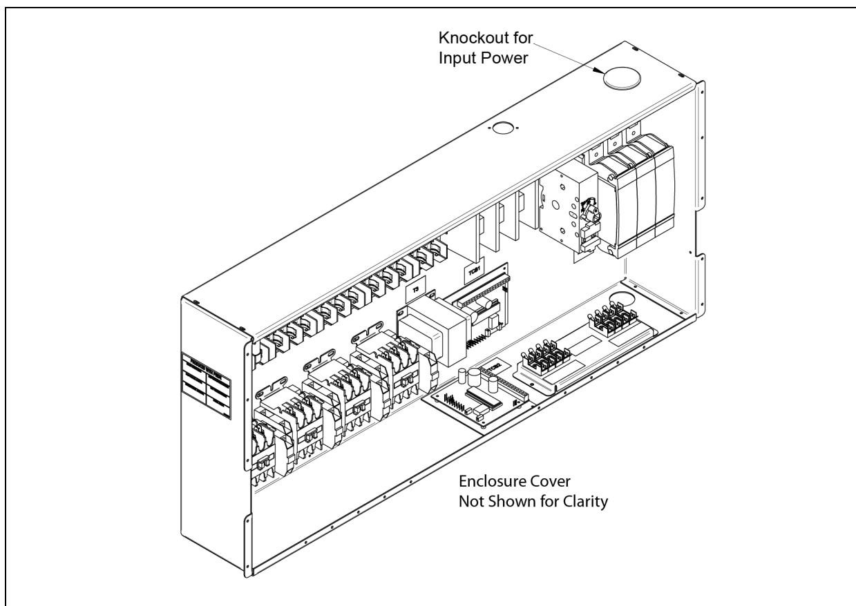
Figure 5.6 Liebert XDC electrical enclosure knockout locations for field wiring
