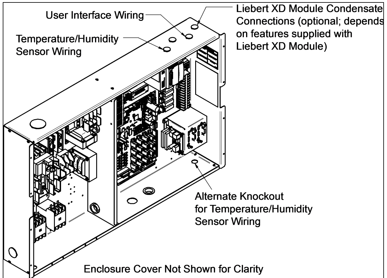
Figure 5.12 Liebert XDC electrical enclosure knockout locations for Extra Low-Voltage connections
