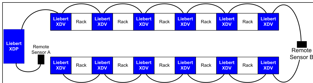
Figure 3.34 Sensor within the daisy chain of Liebert XDV smart modules in CANbus network
