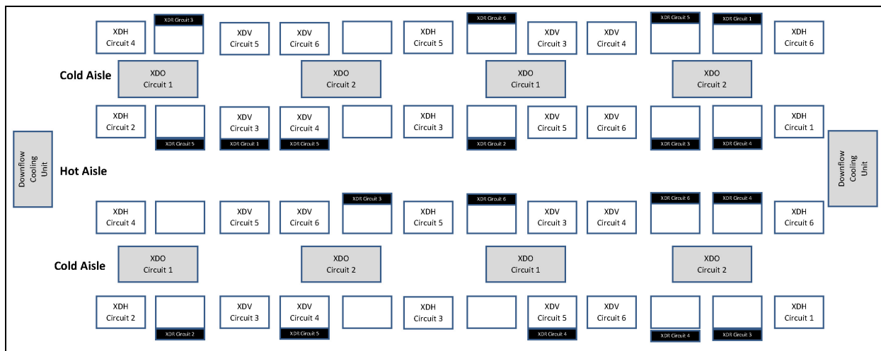
Figure 3.12 Multiple Liebert XD modules in an interlaced system
