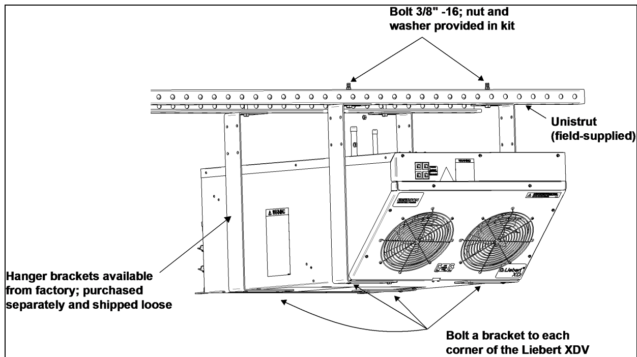
Figure 4.23 Suspending single Liebert XDV from Unistruts
