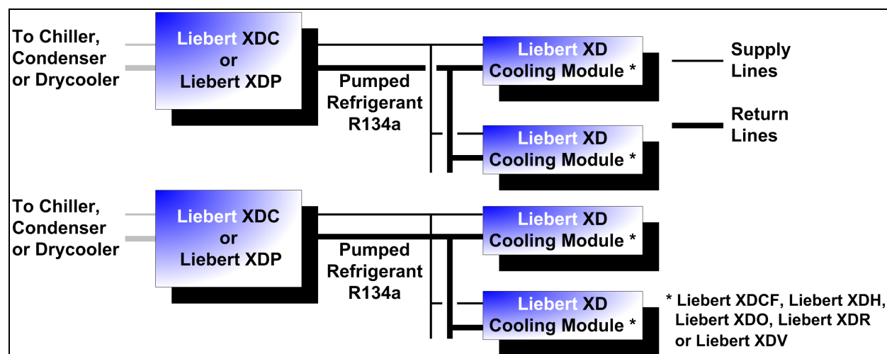
Figure 4.1 Liebert XDCF generic piping layout
