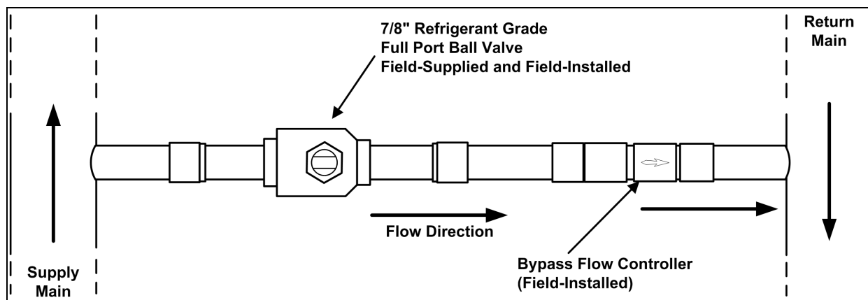
Figure 3.17 Bypass flow controller arrangement
