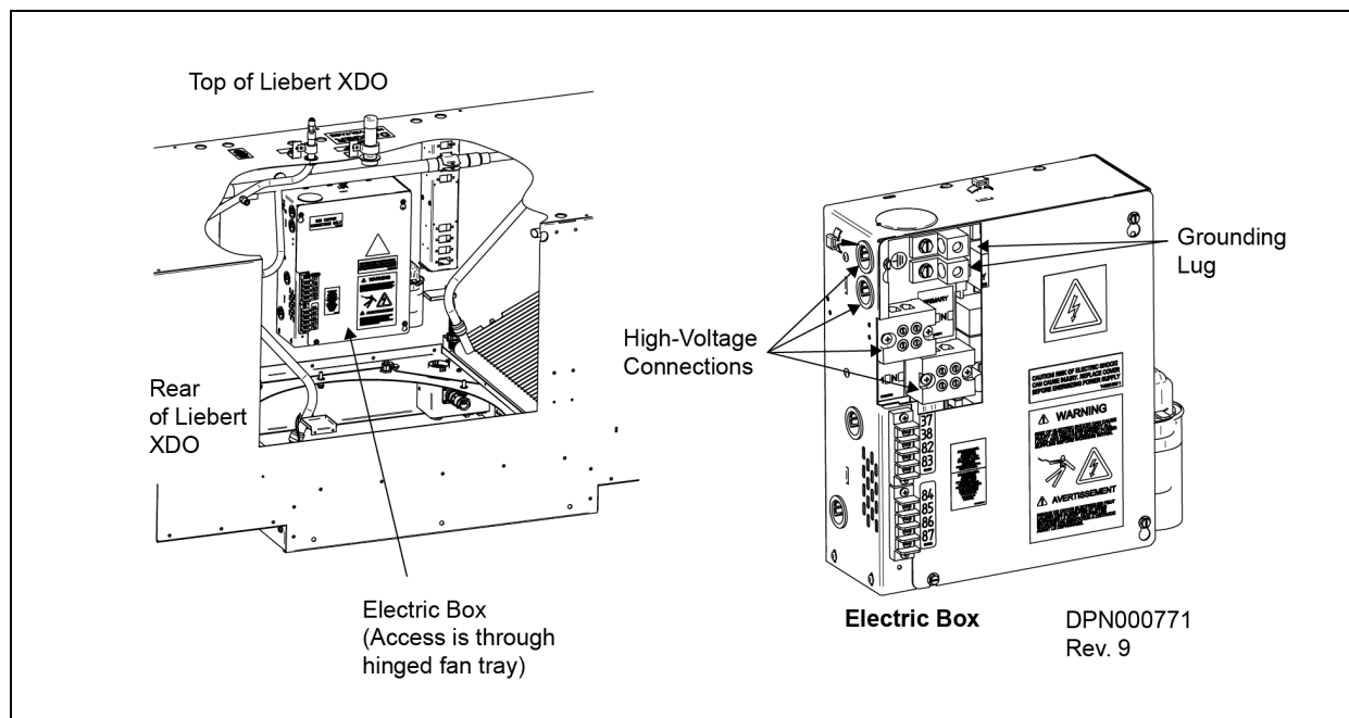
Figure 4.16 High-voltage terminal block connection locations—Liebert XDO smart modules
