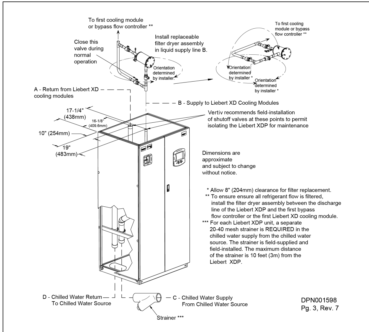
Figure 3.29 Piping access points
