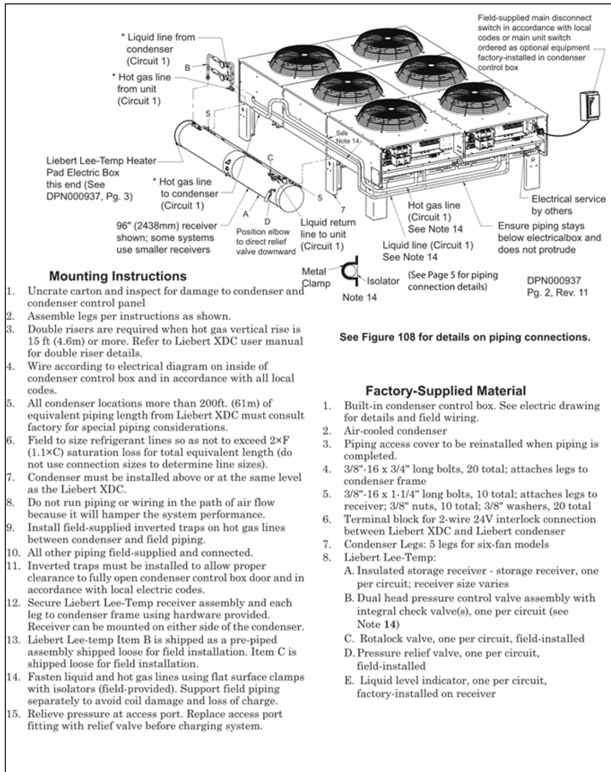
Figure 6.6 Installation data—Liebert Lee-Temp, one-circuit, high ambient six-fan model
