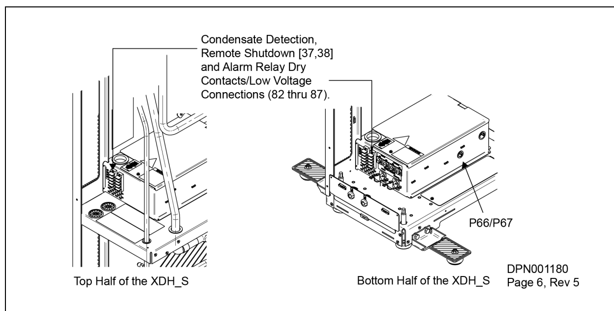
Figure 4.9 Low-voltage connections—Liebert XDH smart module
