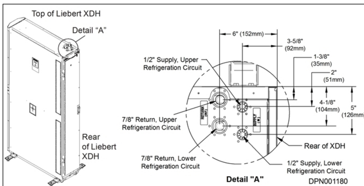
Figure 4.6 Supply and return piping connections—Liebert XDH
