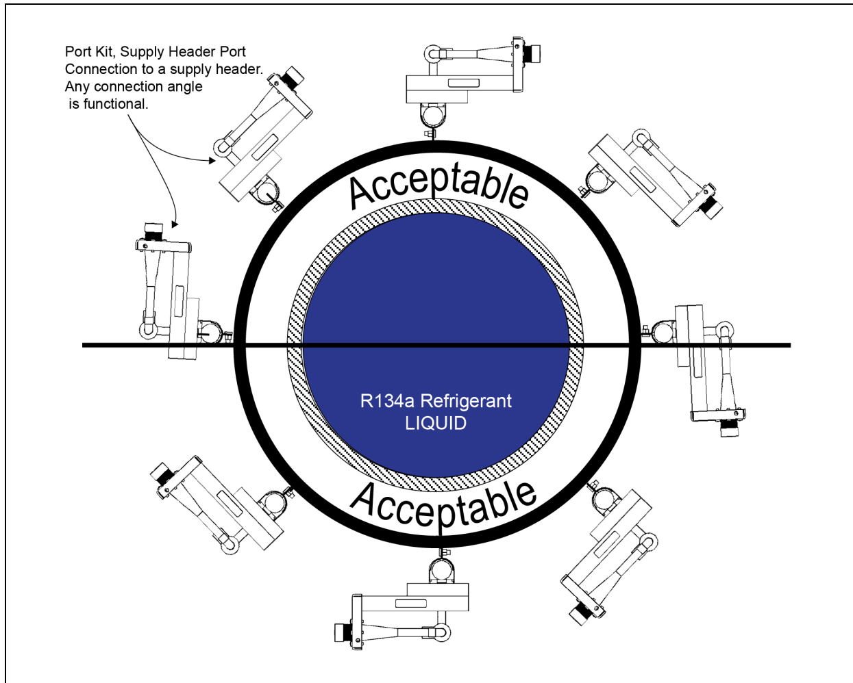
Figure 3.23 Liebert XD supply header orientation
