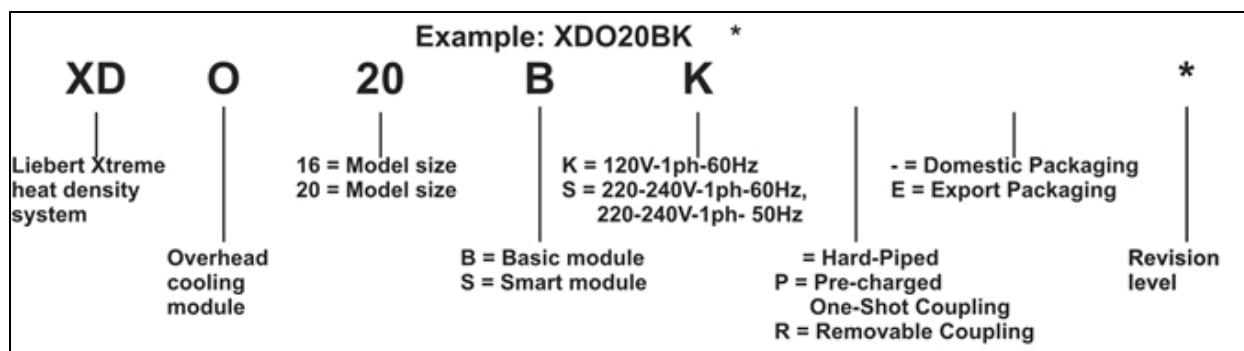
Figure 9.3 Liebert XDO model number nomenclature
