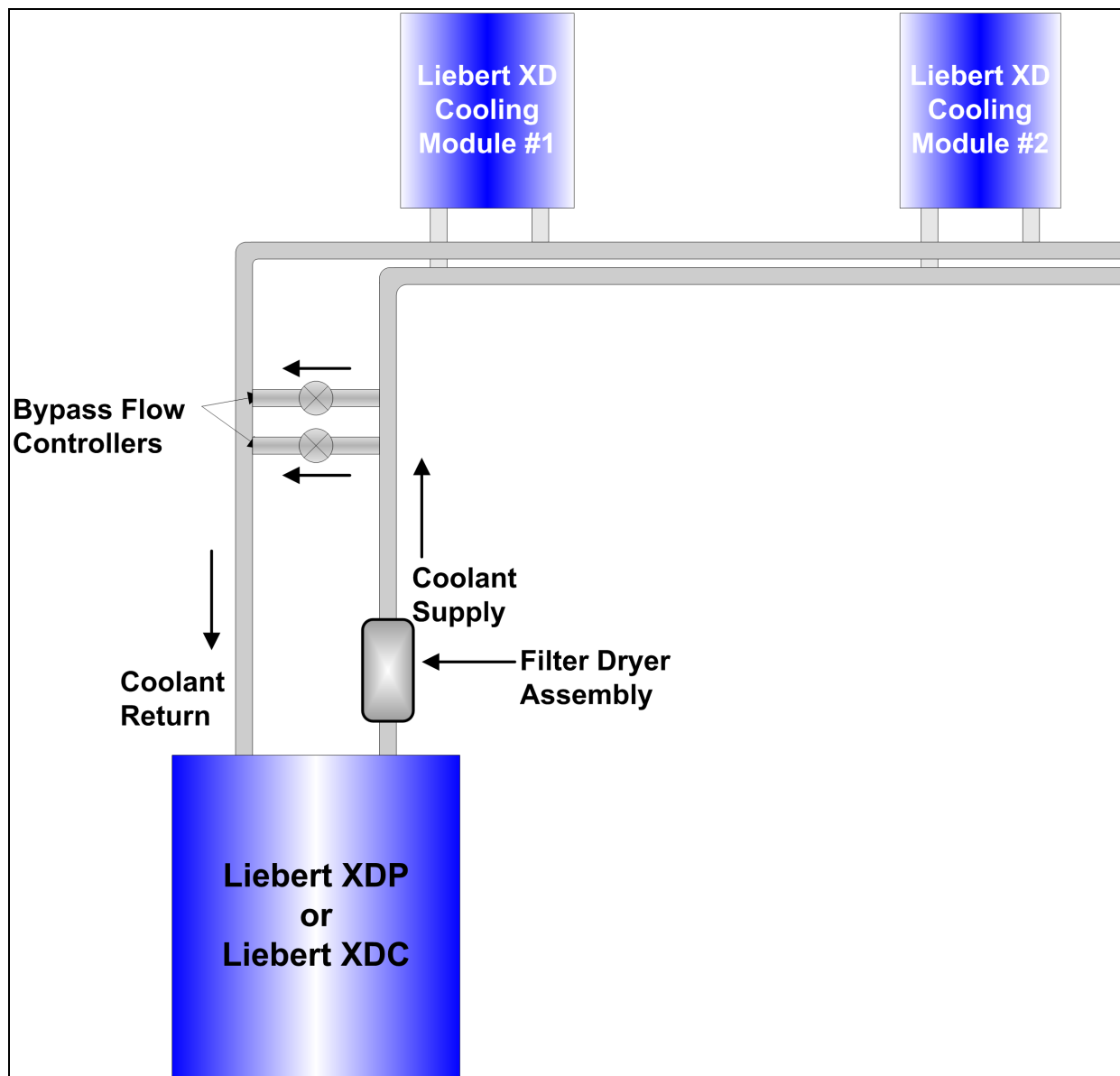
Figure 3.18 Bypass flow controller piping
