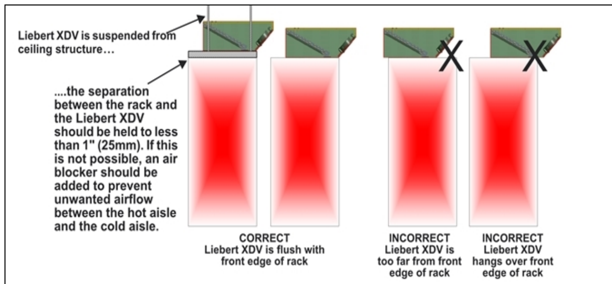
Figure 3.7 Positioning Liebert XDV on top of cabinet
