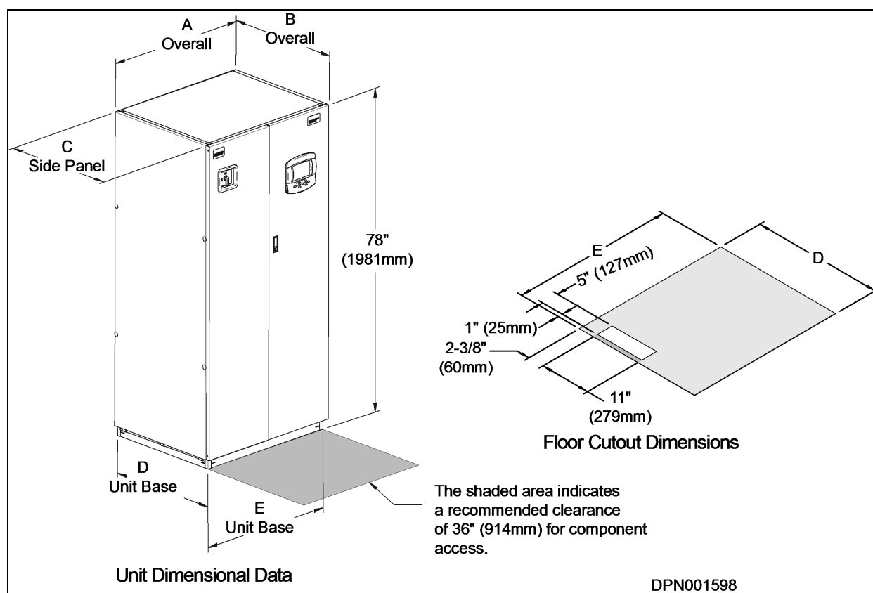
Figure 5.14 Liebert XDP dimensions
