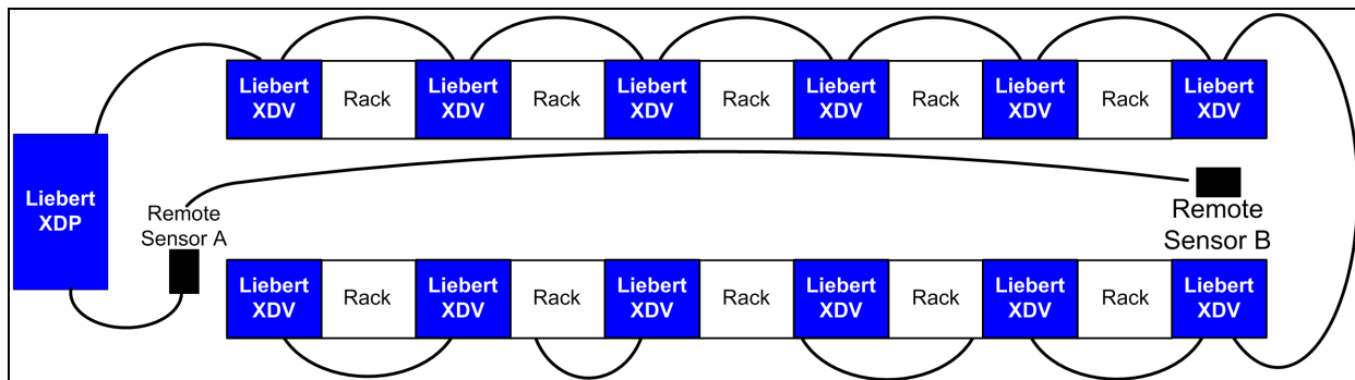
Figure 3.36 Independent smart module and sensor daisy chains in CANbus network
