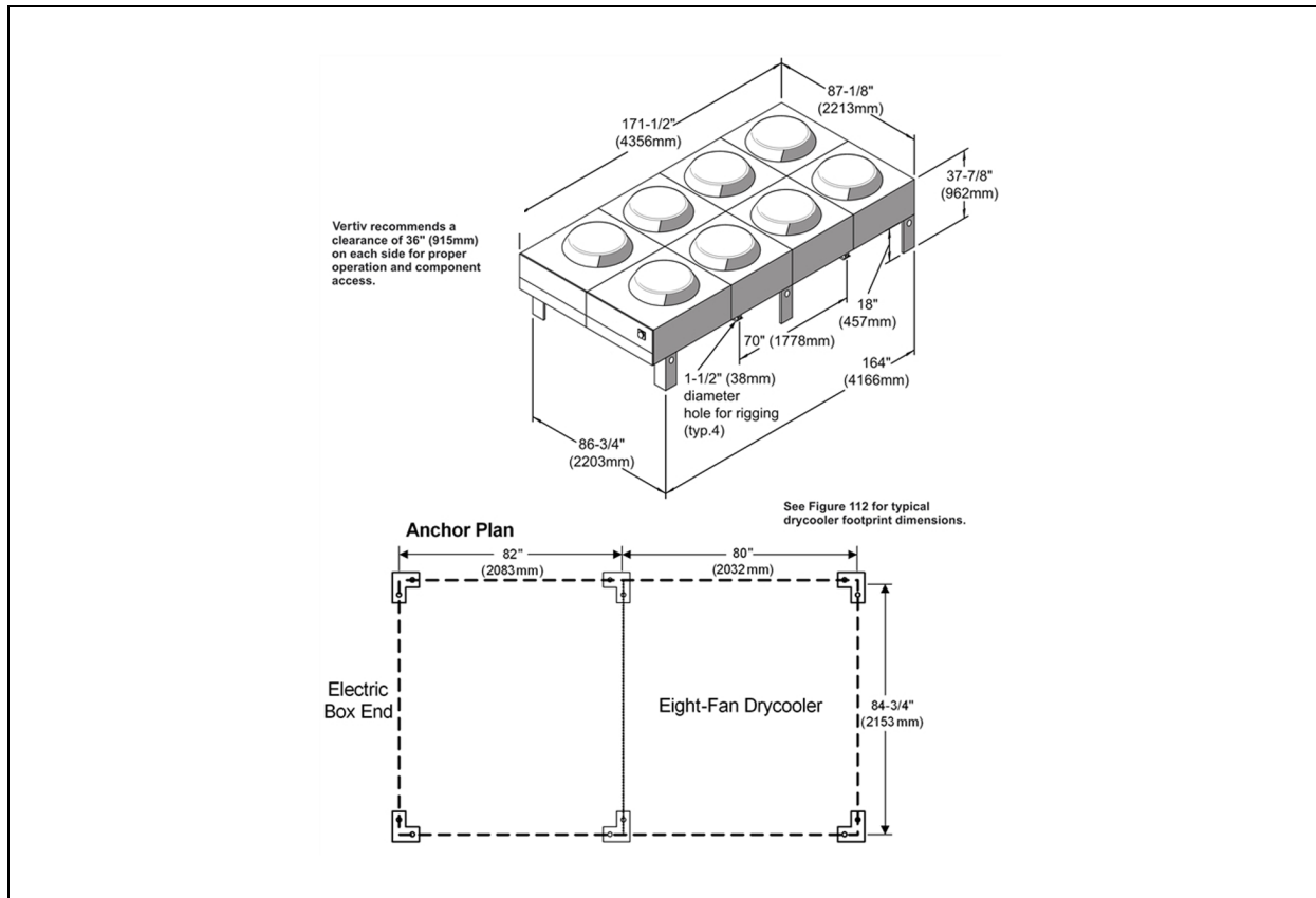
Figure 6.13 Drycooler planning dimensional data—Eight-fan units
