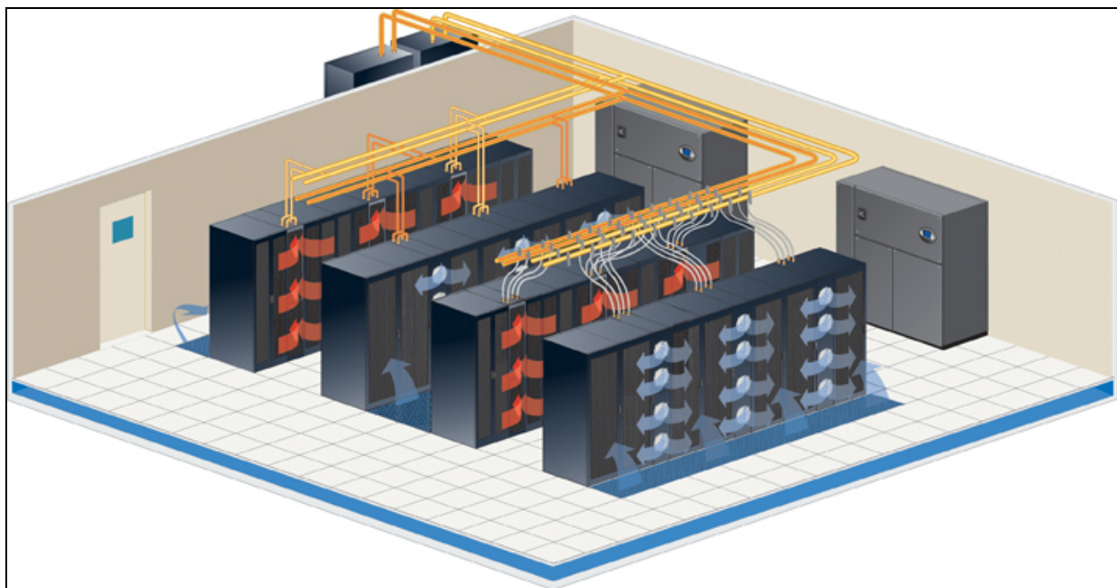
Figure 1.5 Liebert XDH—horizontal cooling module in hot aisle-cold aisle arrangement
