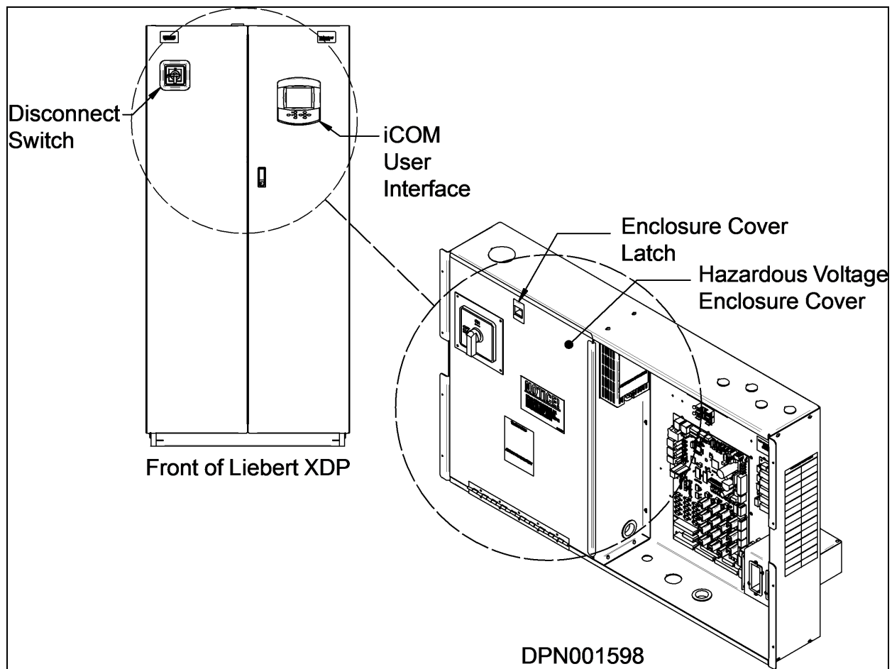
Figure 5.16 Front view of Liebert XDP and electrical enclosure
