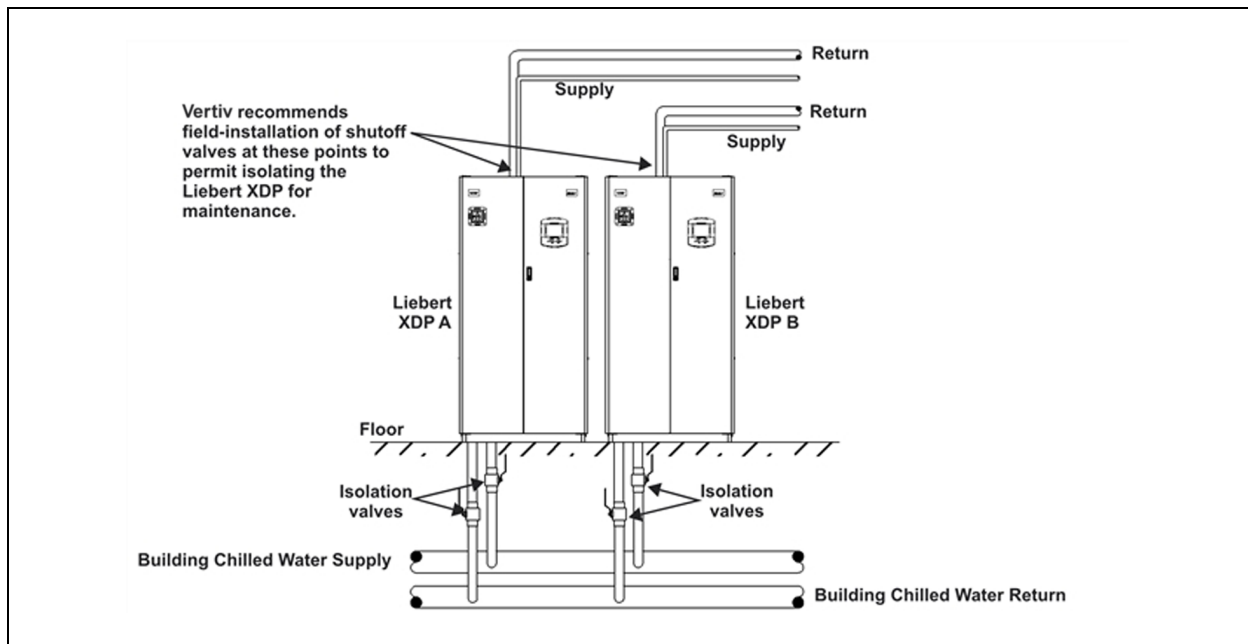
Figure 3.20 General piping details
