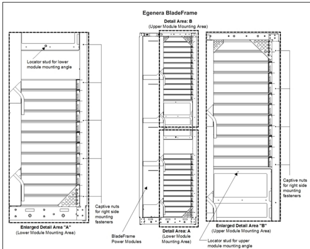
Figure 4.3 Liebert XDCF module mounting locations
