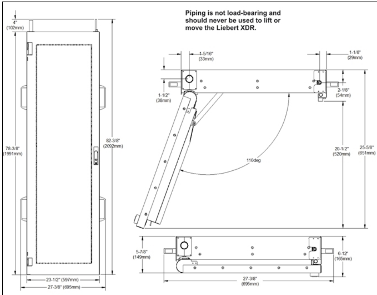
Figure 4.18 Liebert XDR dimensions with hard-piped connections
