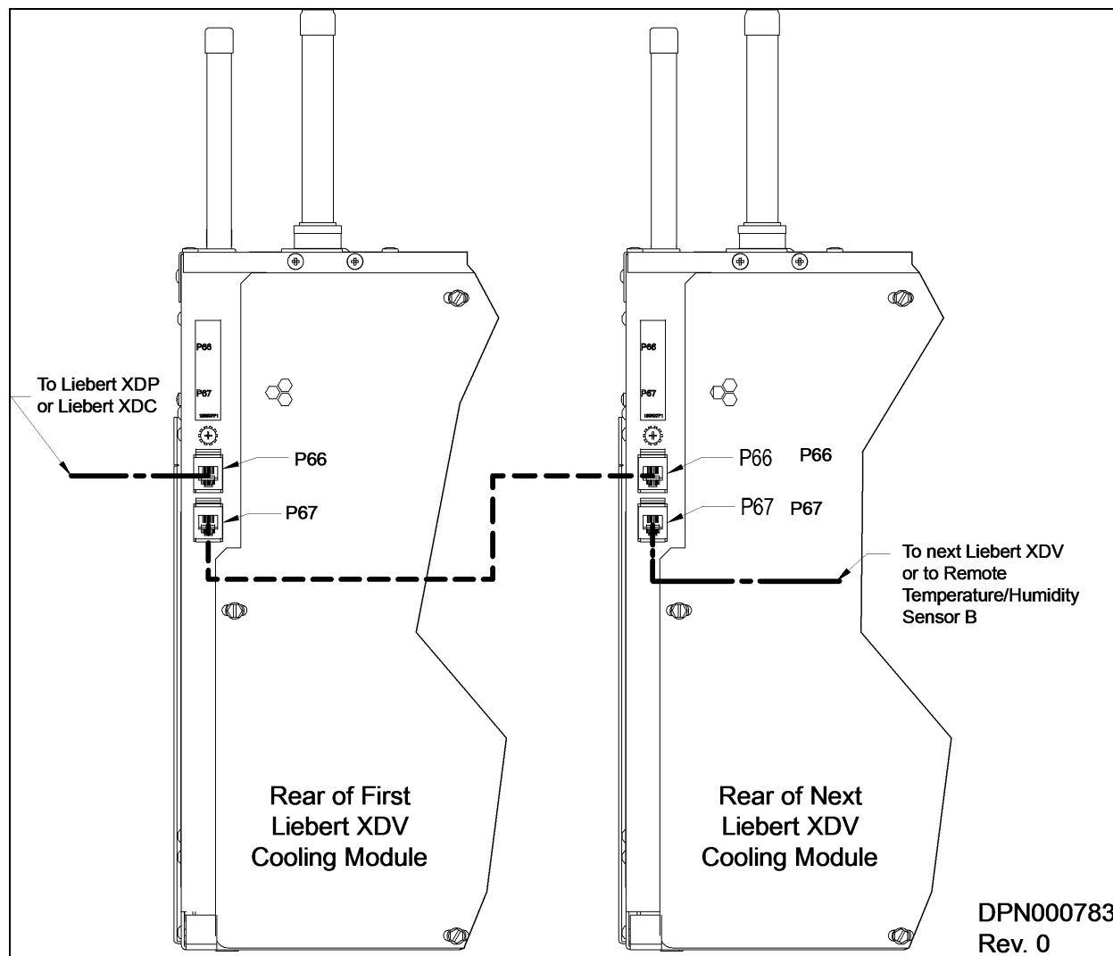
Figure 7.13 Liebert XDV Smart Module CANbus port locations
