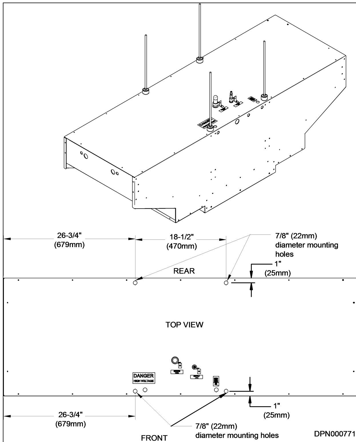
Figure 4.12 Liebert XDO internal mounting location
