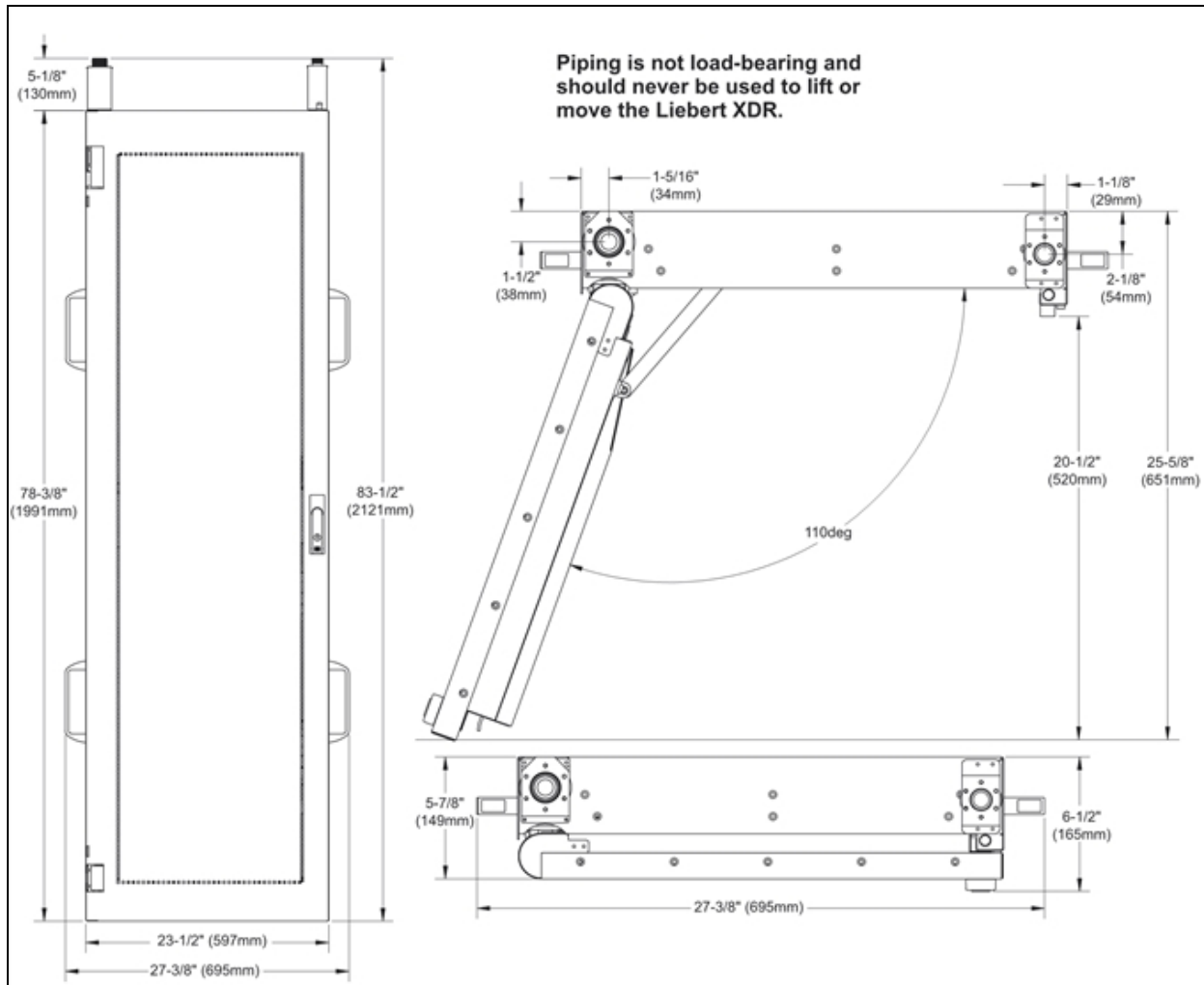
Figure 4.19 Liebert XDR dimensions with one-shot connections (precharged)
