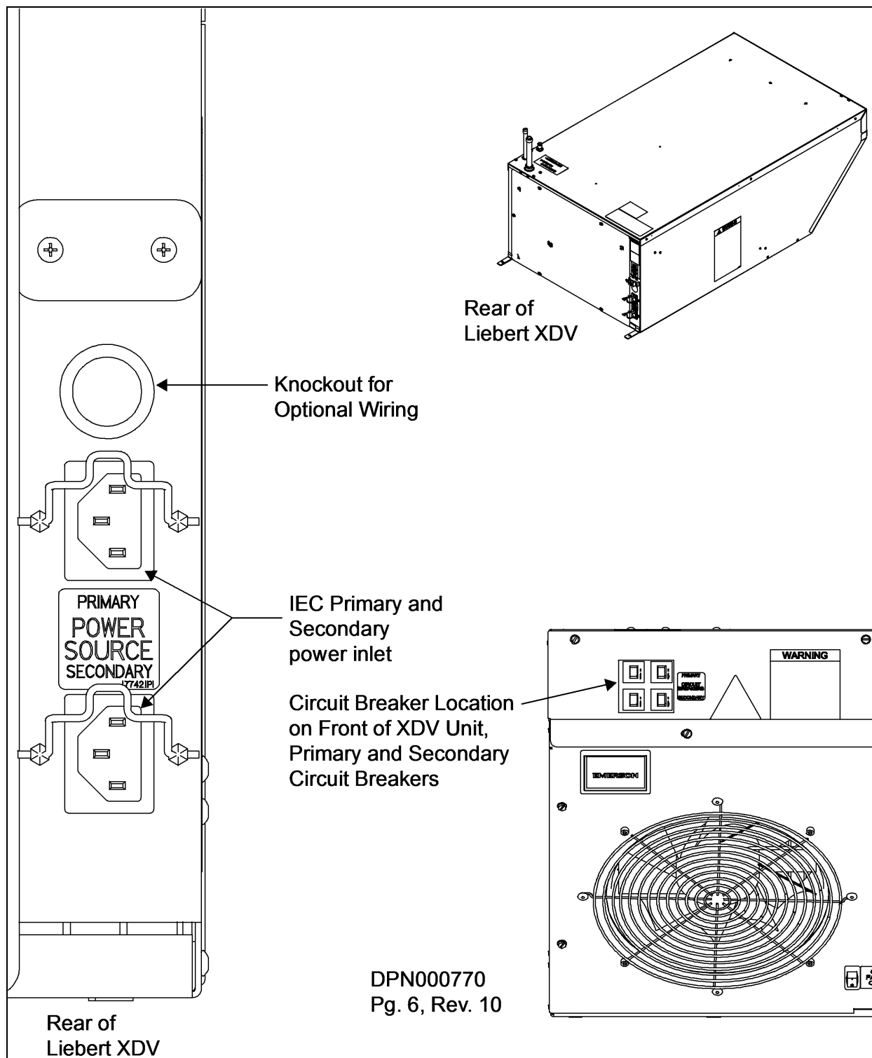
Figure 4.26 Electrical connections for CSA-approved Liebert XDV basic modules
