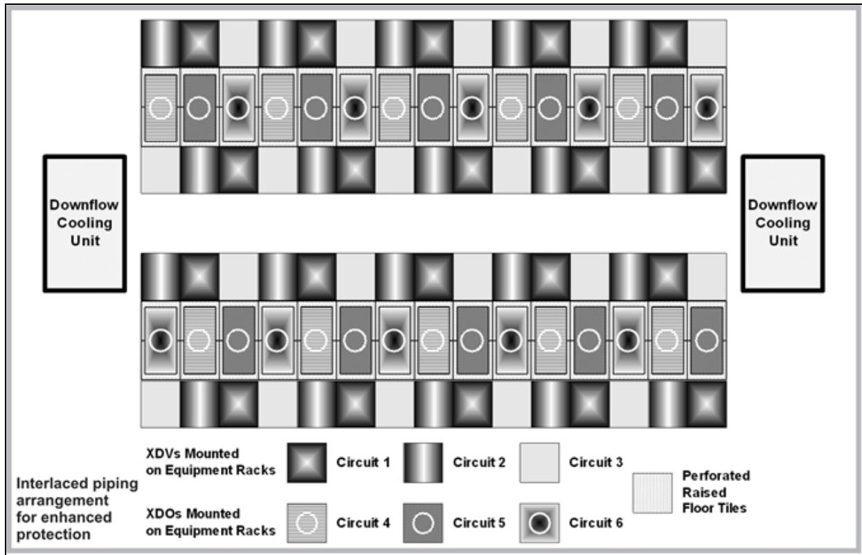
Figure 3.12 Multiple Liebert XD modules in an interlaced system
