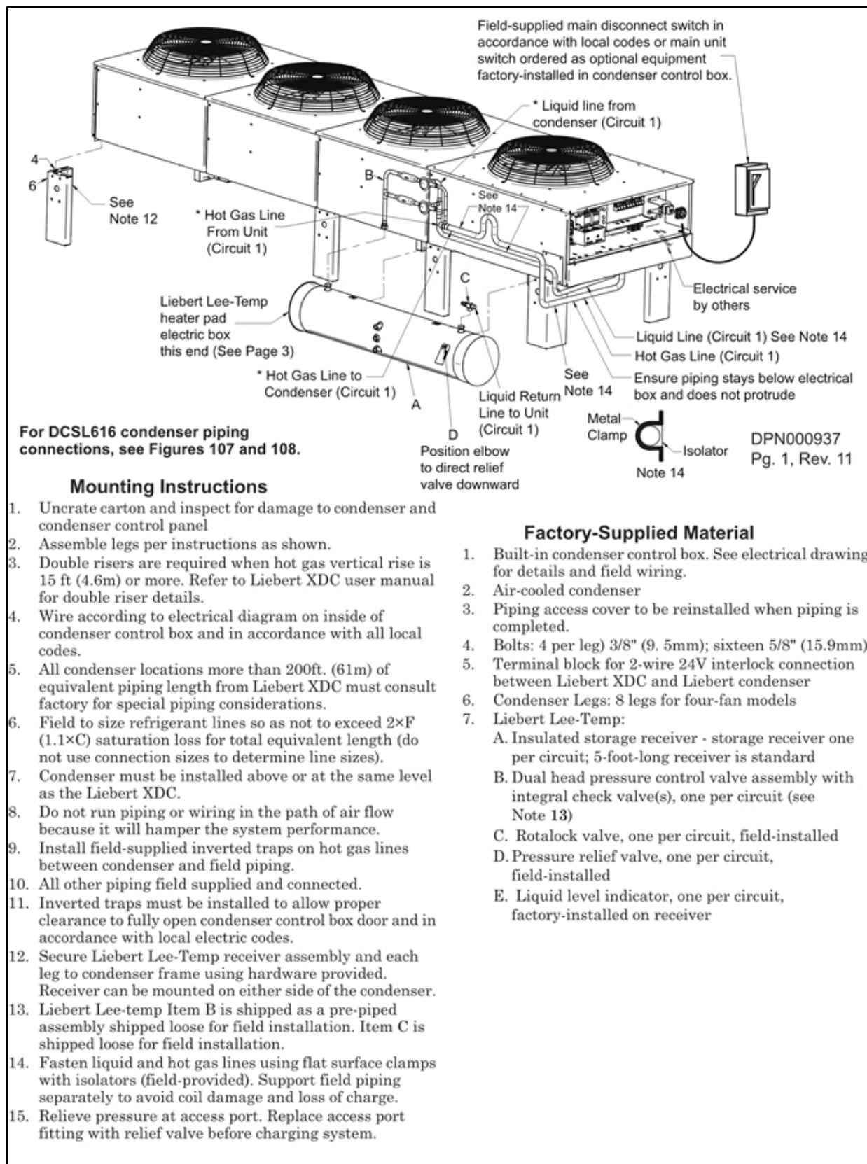
Figure 6.5 Installation data—Liebert Lee-Temp, one-circuit, four-fan model
