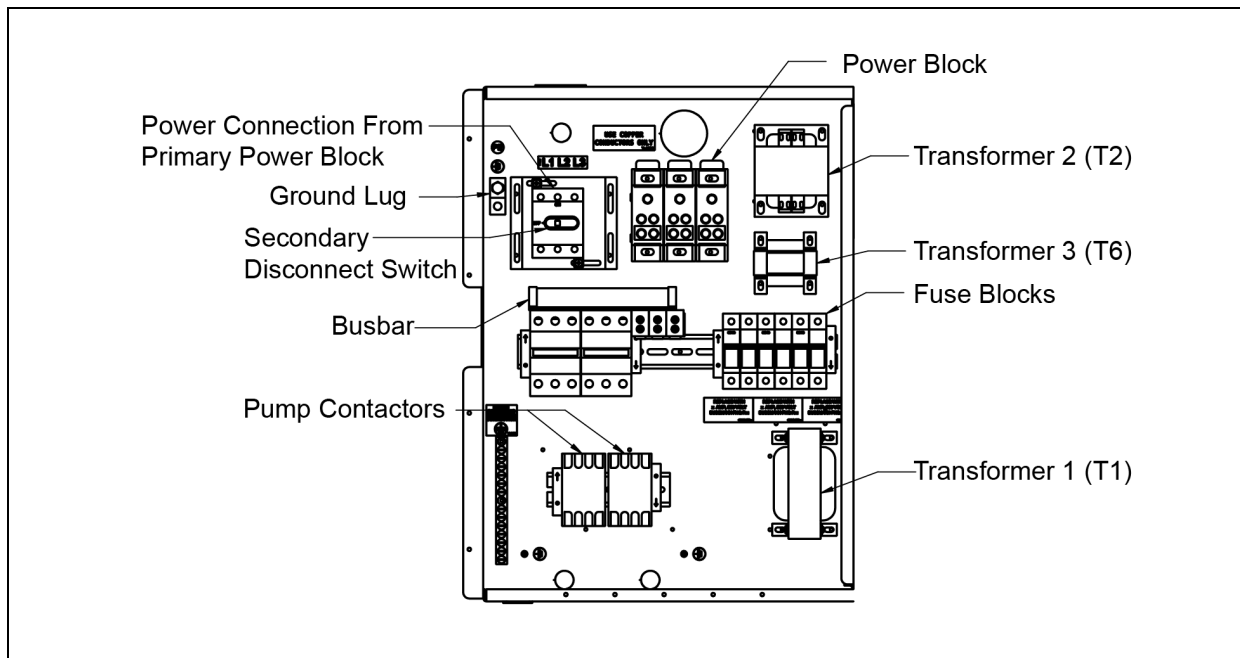
Figure 5.11 Liebert XDC heat rejection electrical connection points
