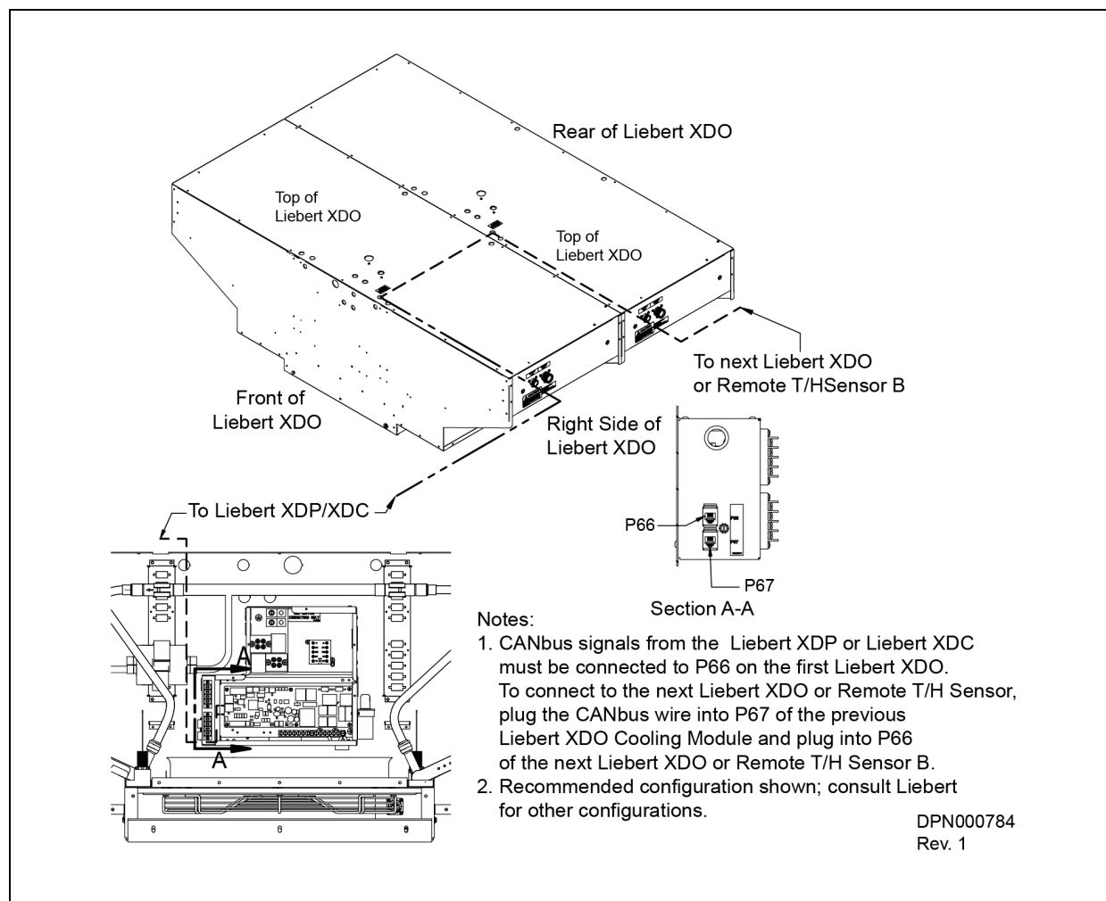
Figure 7.17 Liebert XDO CANbus port locations
