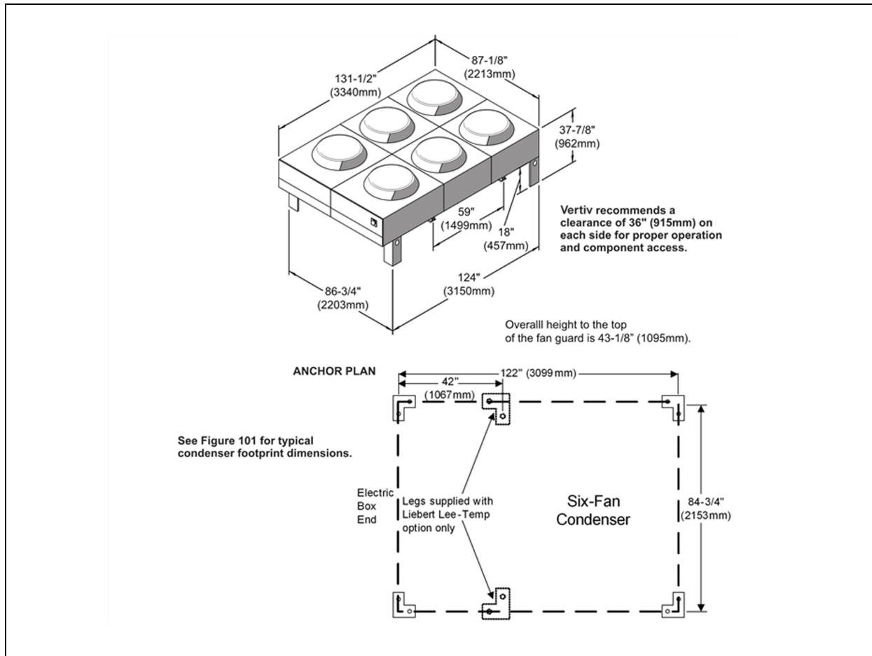
Figure 6.2 Condenser planning dimensional data—Six-fan units
