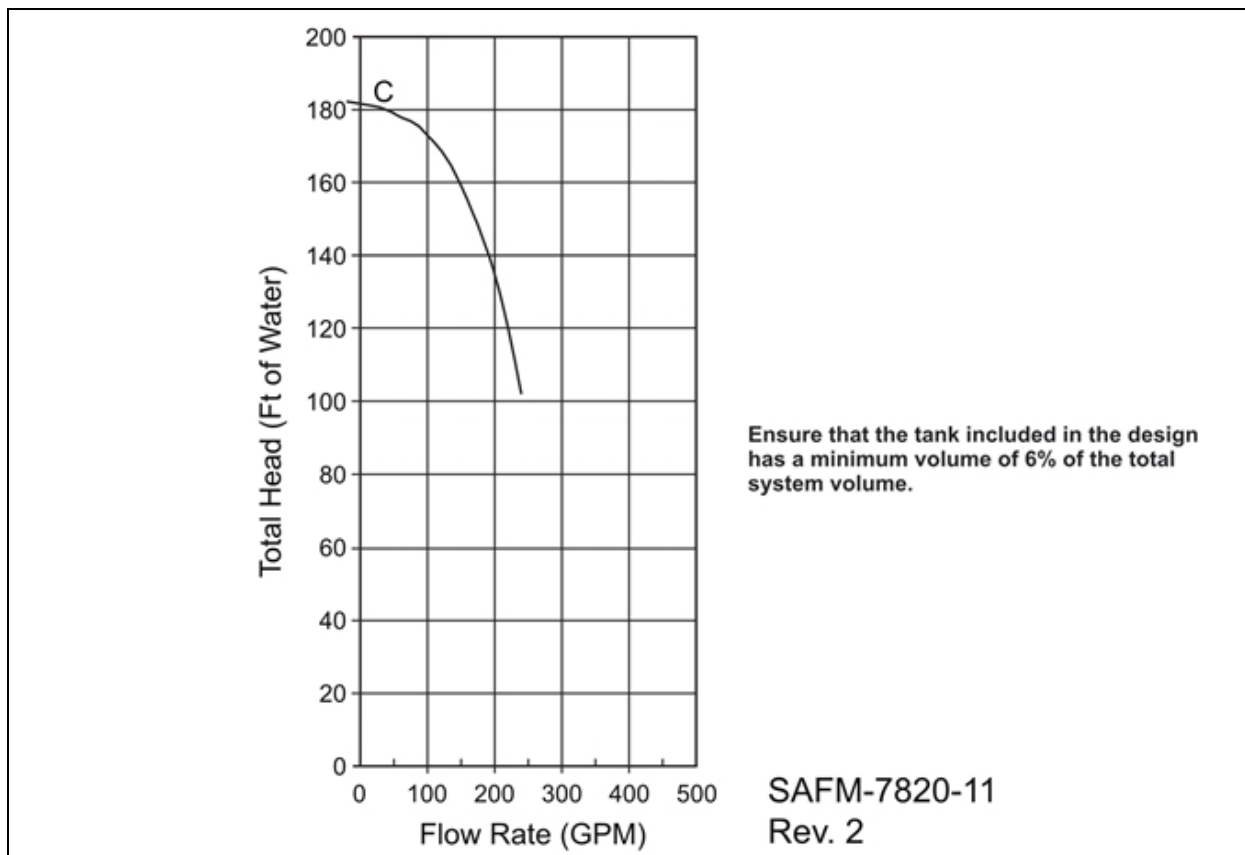
Figure 6.17 Flow rate, 10 hp, 3500 rpm pump package, Model # 9A31258G3 in aluminum enclosure
