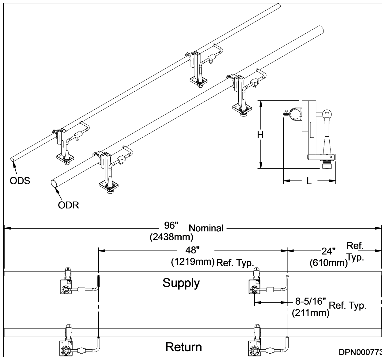
Figure 3.25 Two-port prefabricated piping for Liebert XD cooling modules
