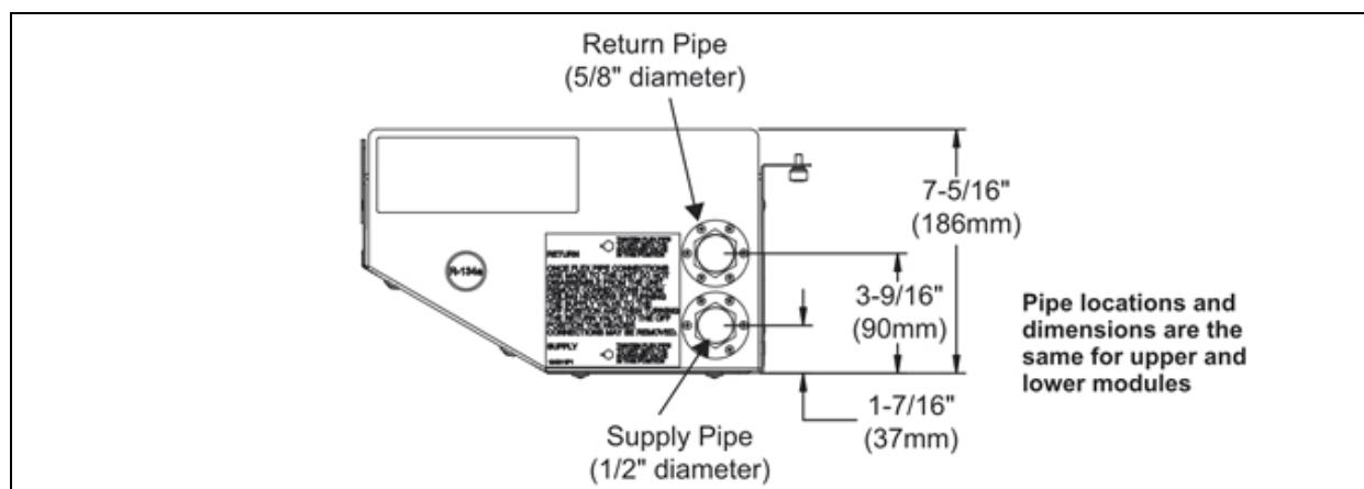
Figure 4.4 Liebert XDCF supply and return piping access points
