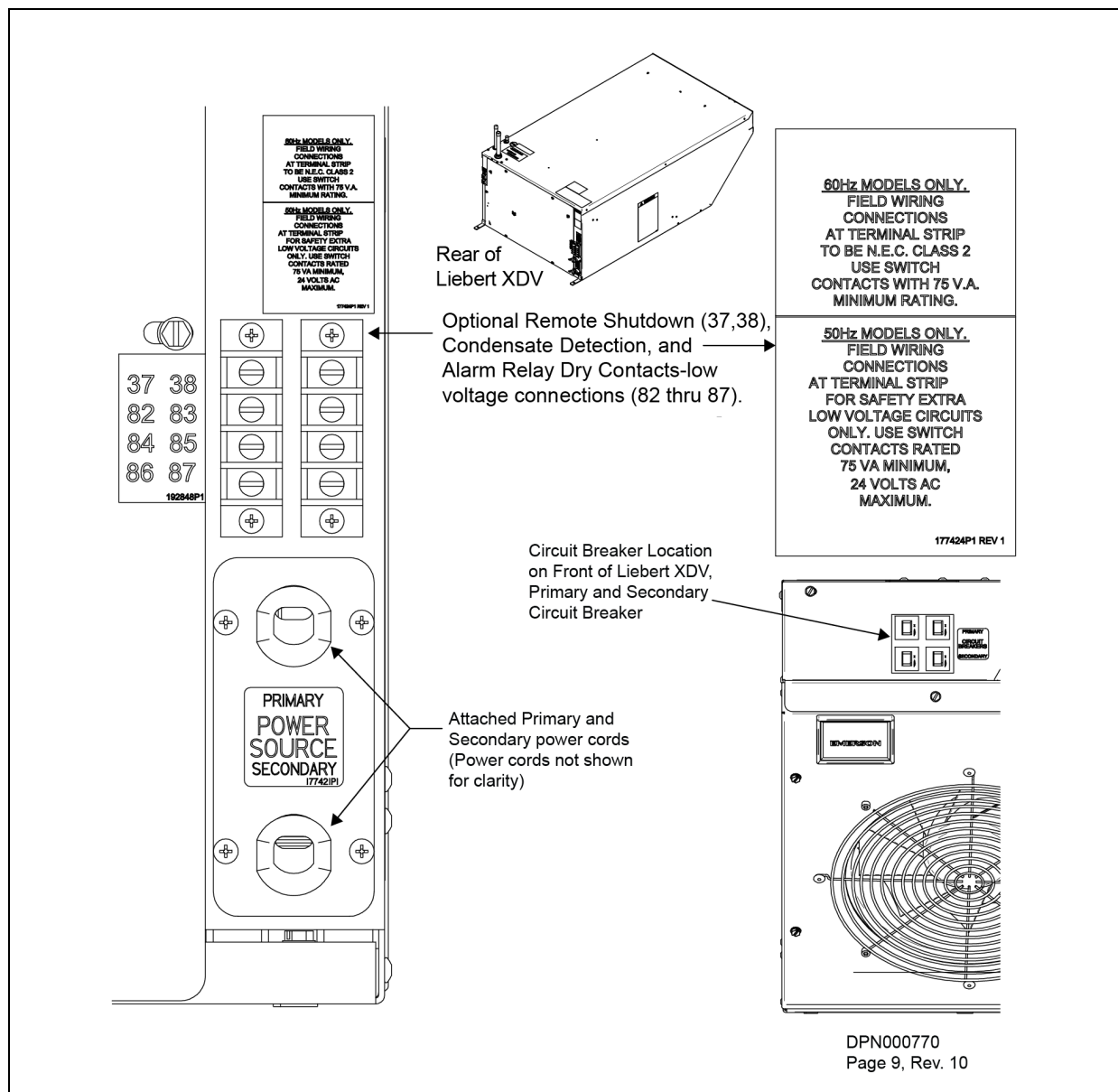
Figure 4.29 Electrical connections for CE-approved Liebert XDV smart modules
