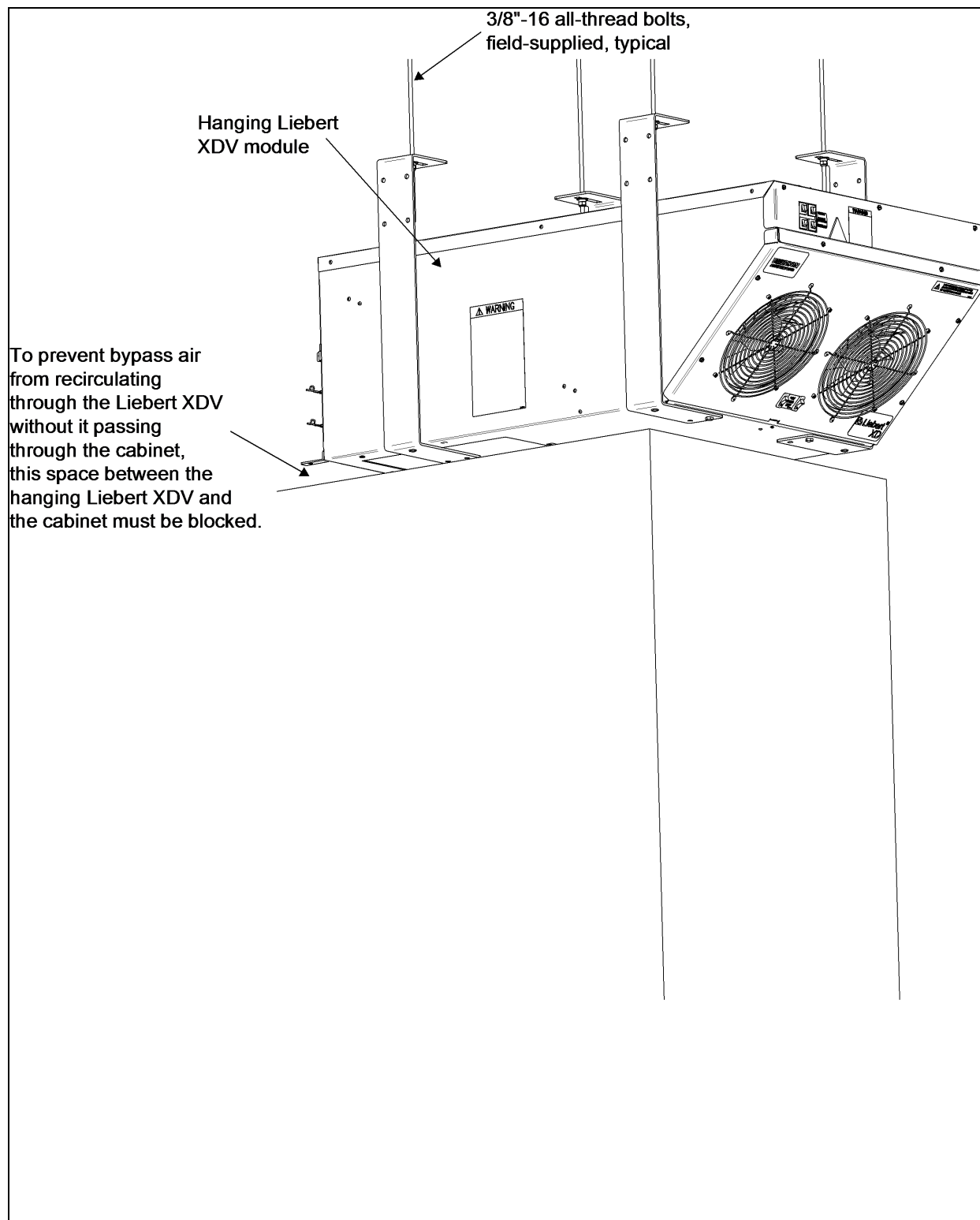
Figure 4.24 Suspending single Liebert XDV from the roof structure
