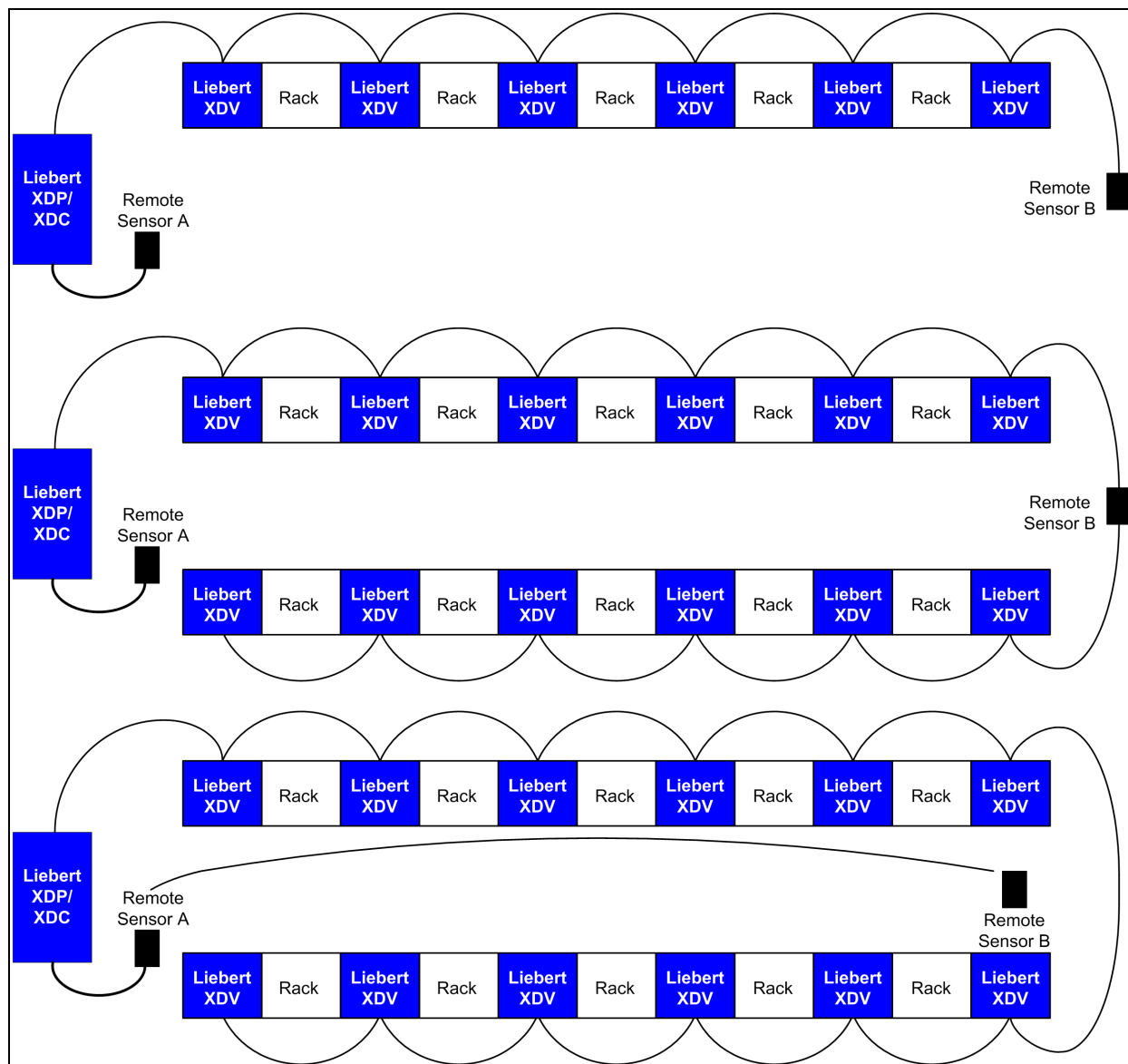
Figure 7.7 Modules on a single chain
