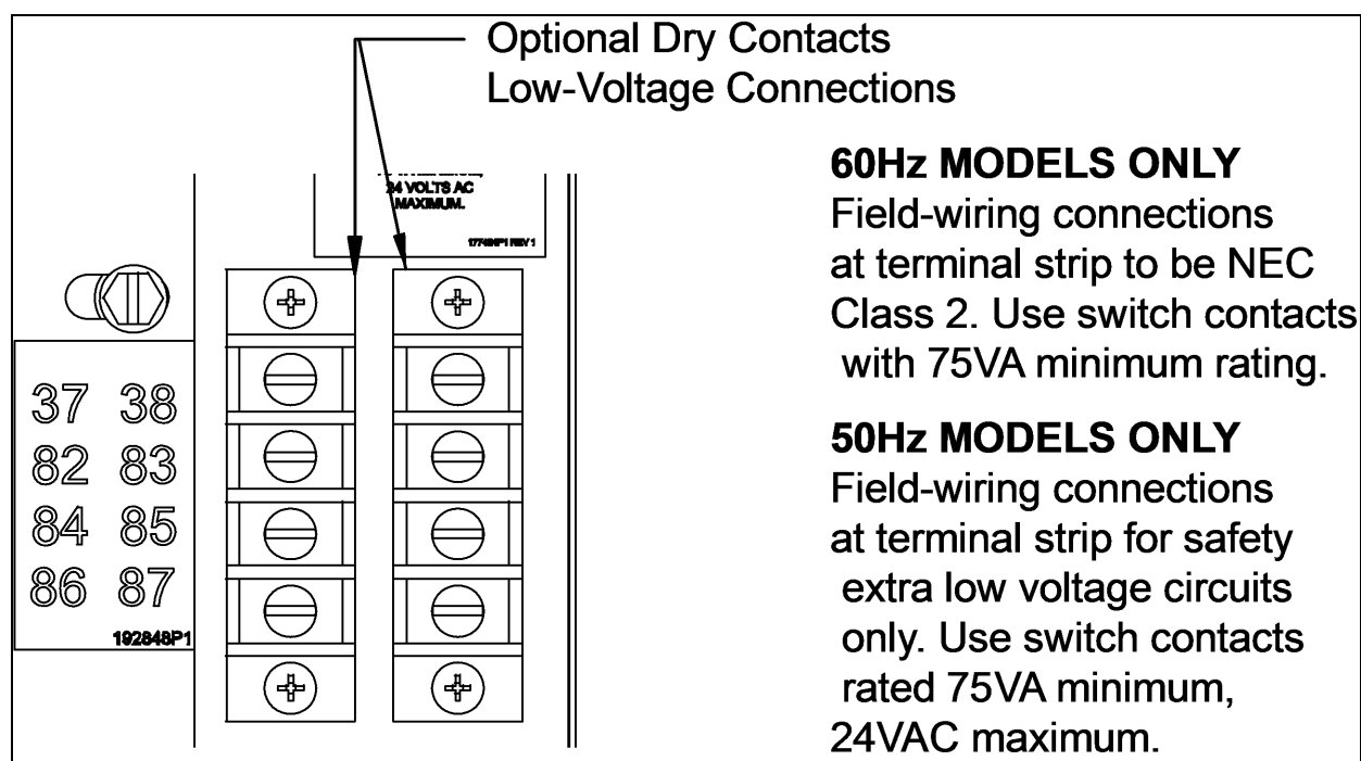
Figure 4.30 Low-voltage connections for Liebert XDV smart modules
