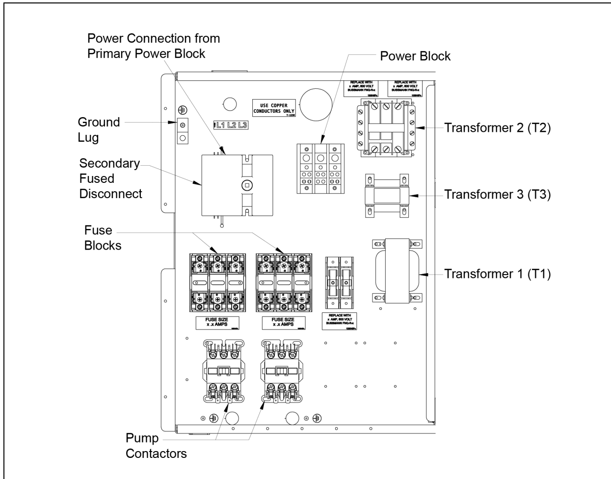
Figure 5.9 Liebert XDC high-voltage connections—secondary disconnect switch, 60Hz models
