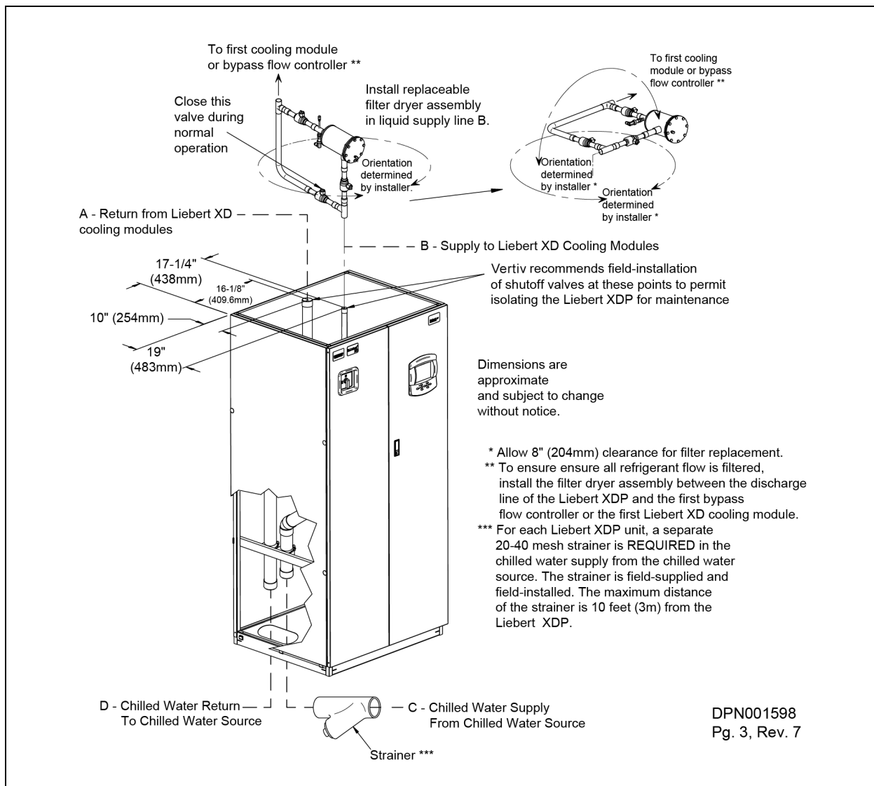
Figure 5.15 Liebert XDP piping access points and external features
