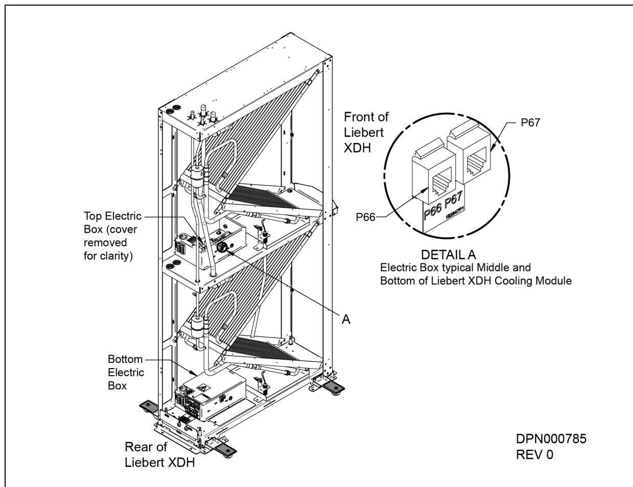
Figure 7.14 Liebert XDH CANbus port locations
