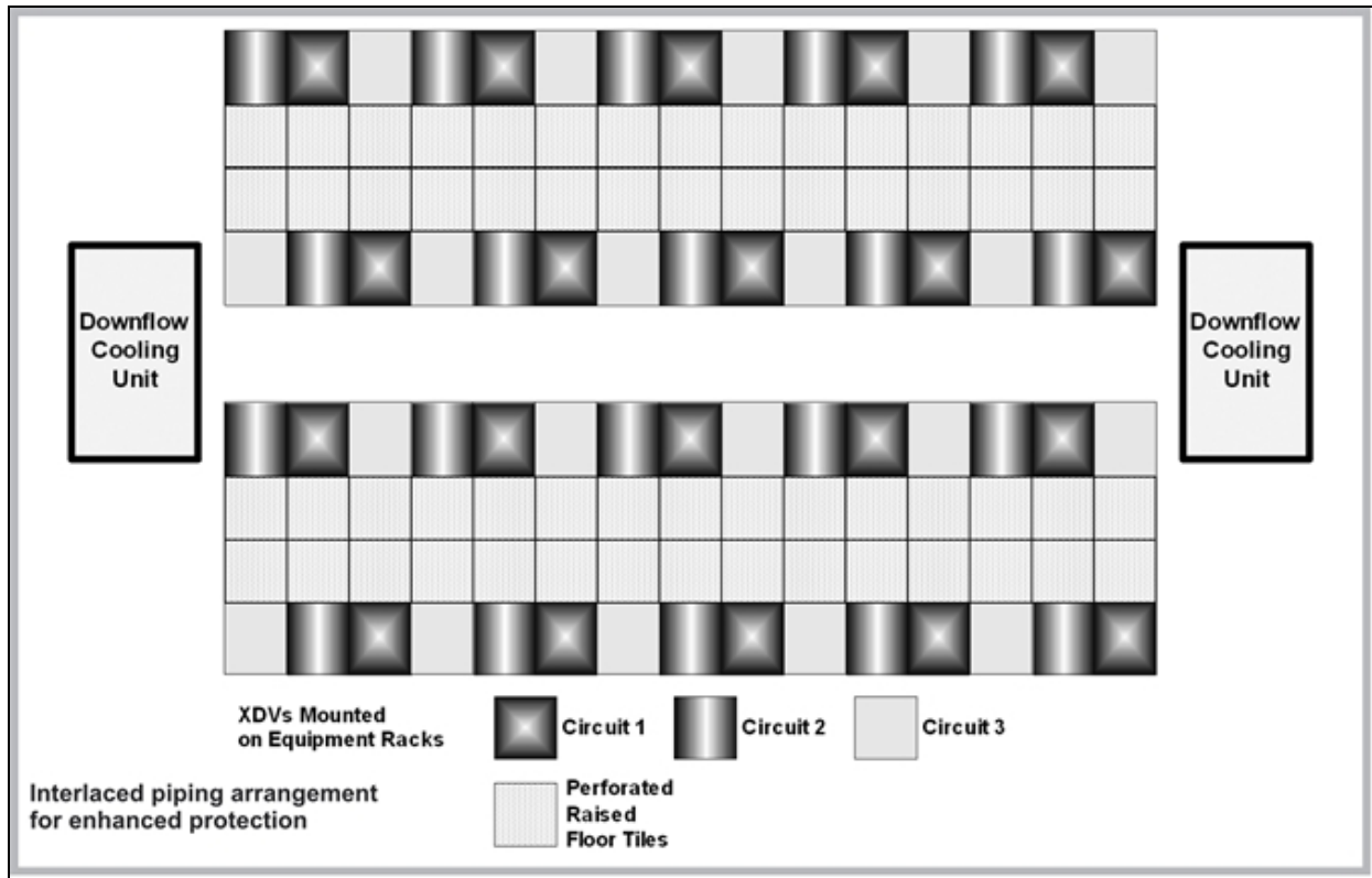
Figure 3.10 Liebert XDV modules mounted on racks emitting 8kW of heat top view
