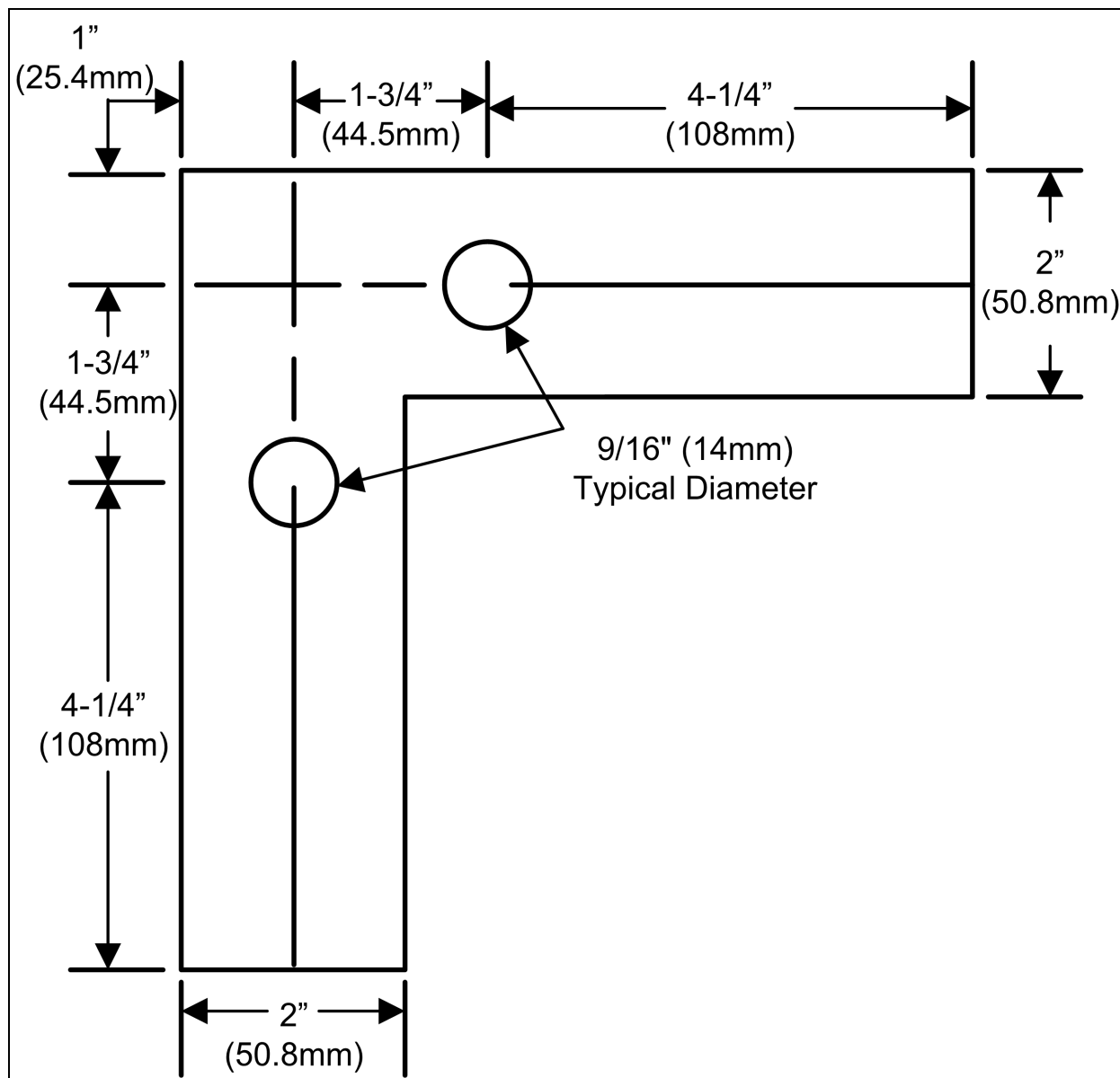
Figure 6.3 Typical condenser footprint—dimensions
