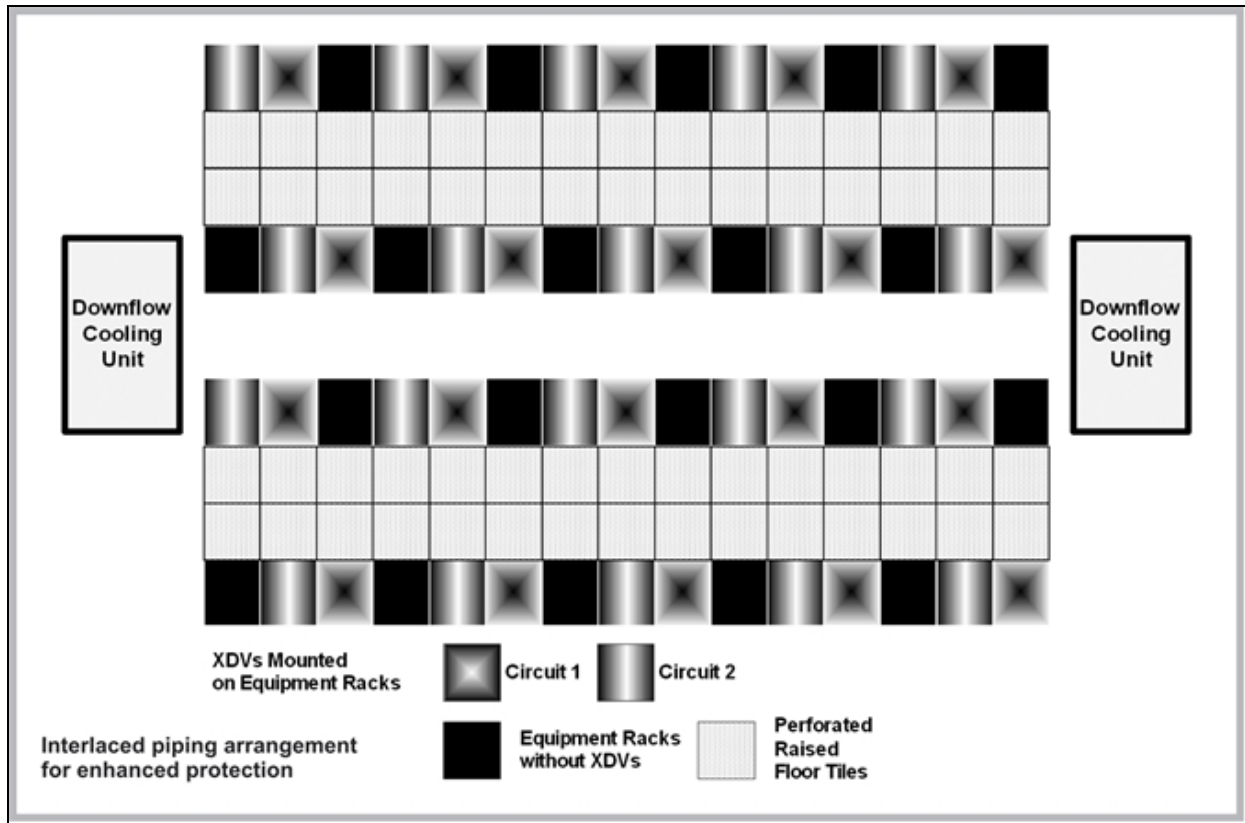
Figure 3.9 Liebert XDV modules mounted on racks emitting 5kW of heat, top view
