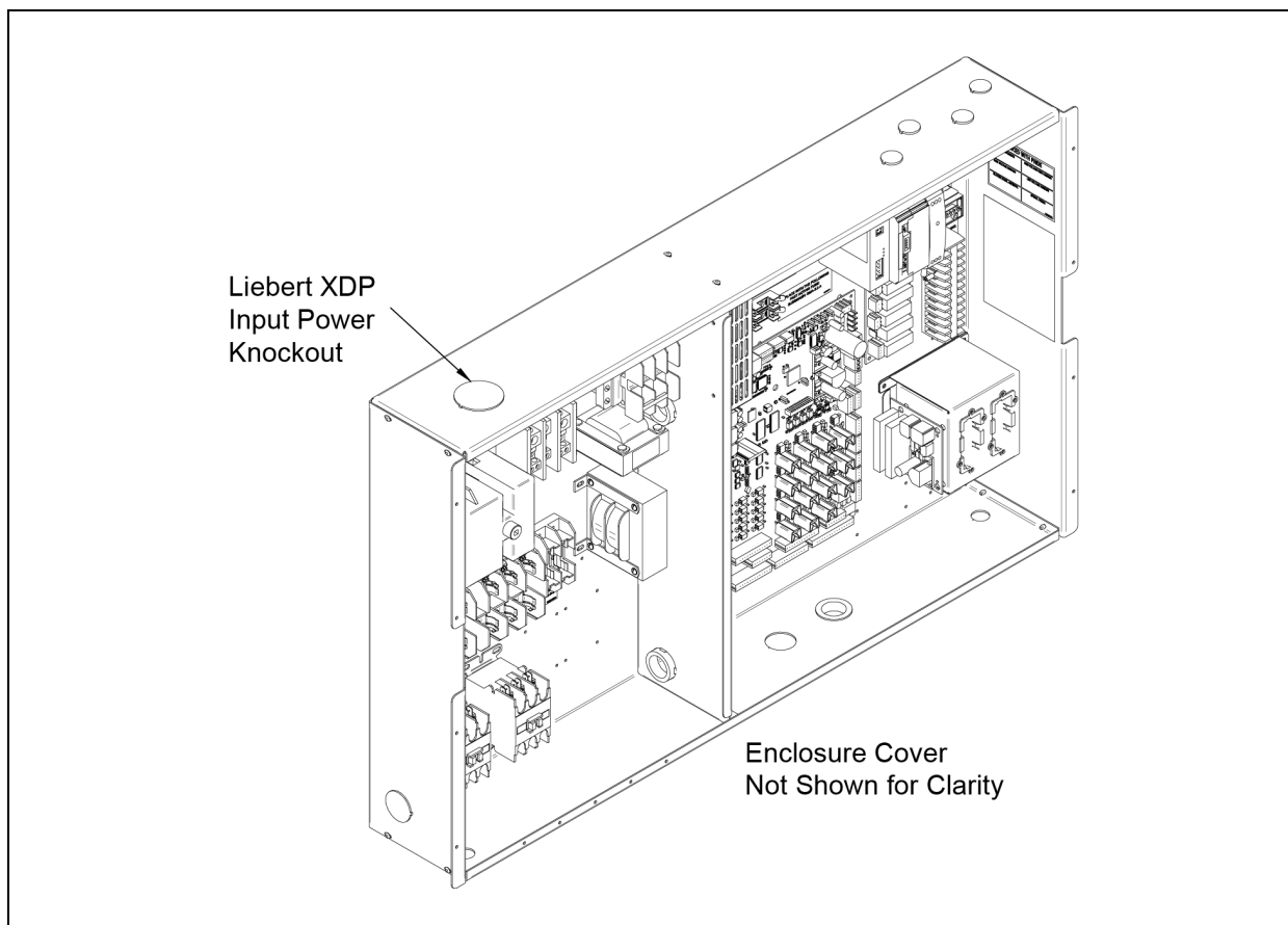
Figure 5.17 Liebert XDP electrical enclosure knockout location for hazardous voltage wiring
