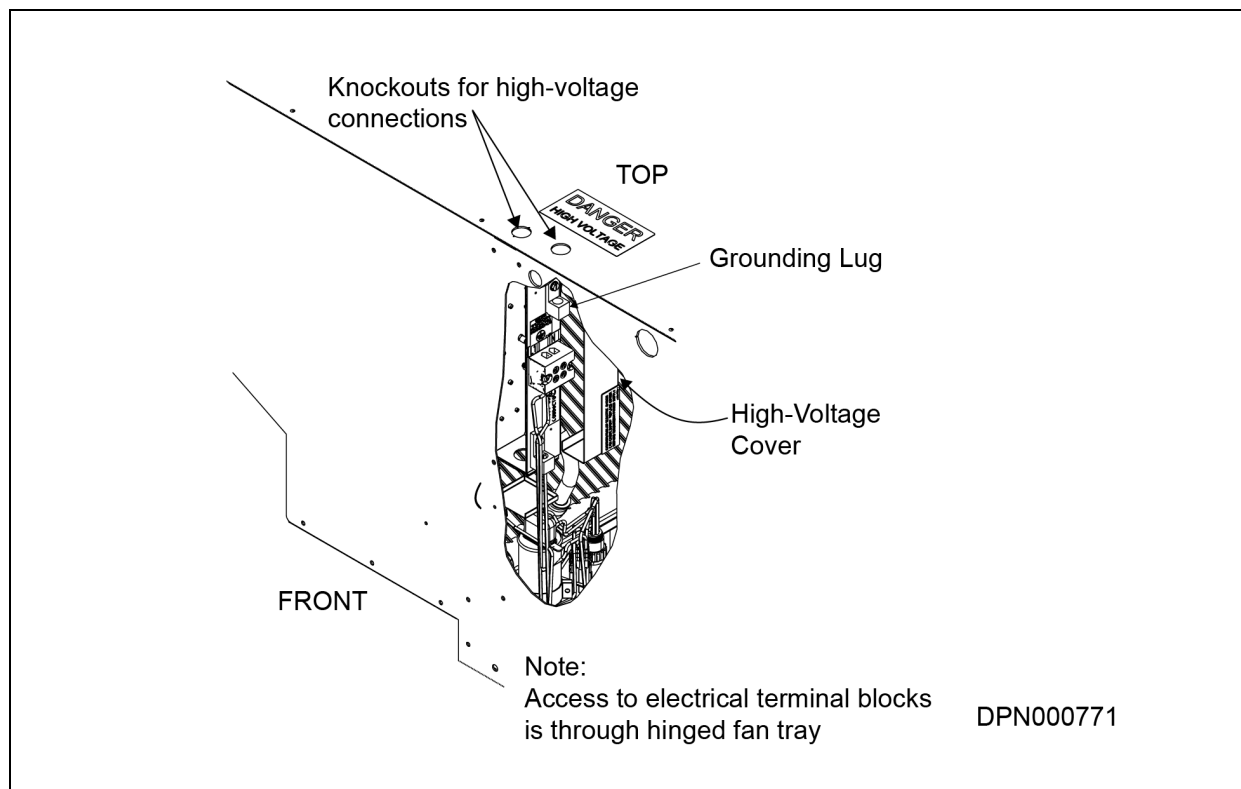
Figure 4.13 Top and front electrical access points and terminal block—standard Liebert XDO modules
