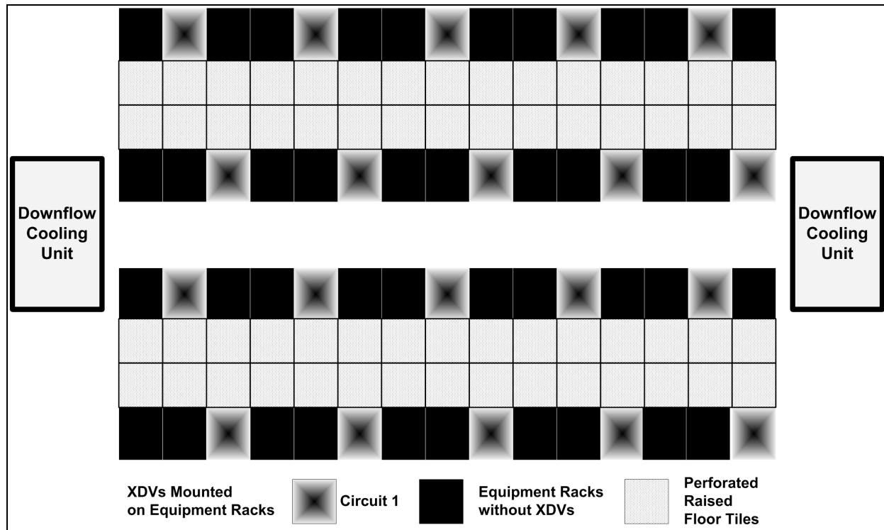
Figure 3.8 Liebert XDV modules mounted on racks emitting 3kW of heat, top view
