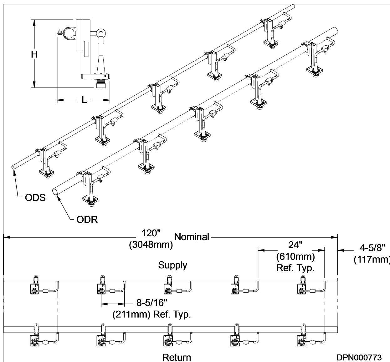
Figure 3.27 Five-port prefabricated piping for Liebert XD cooling modules
