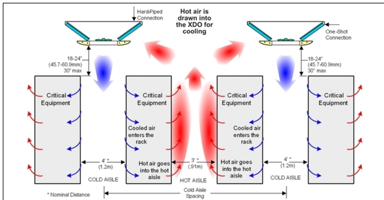
Figure 3.5 Liebert XDO placement over cold aisle
