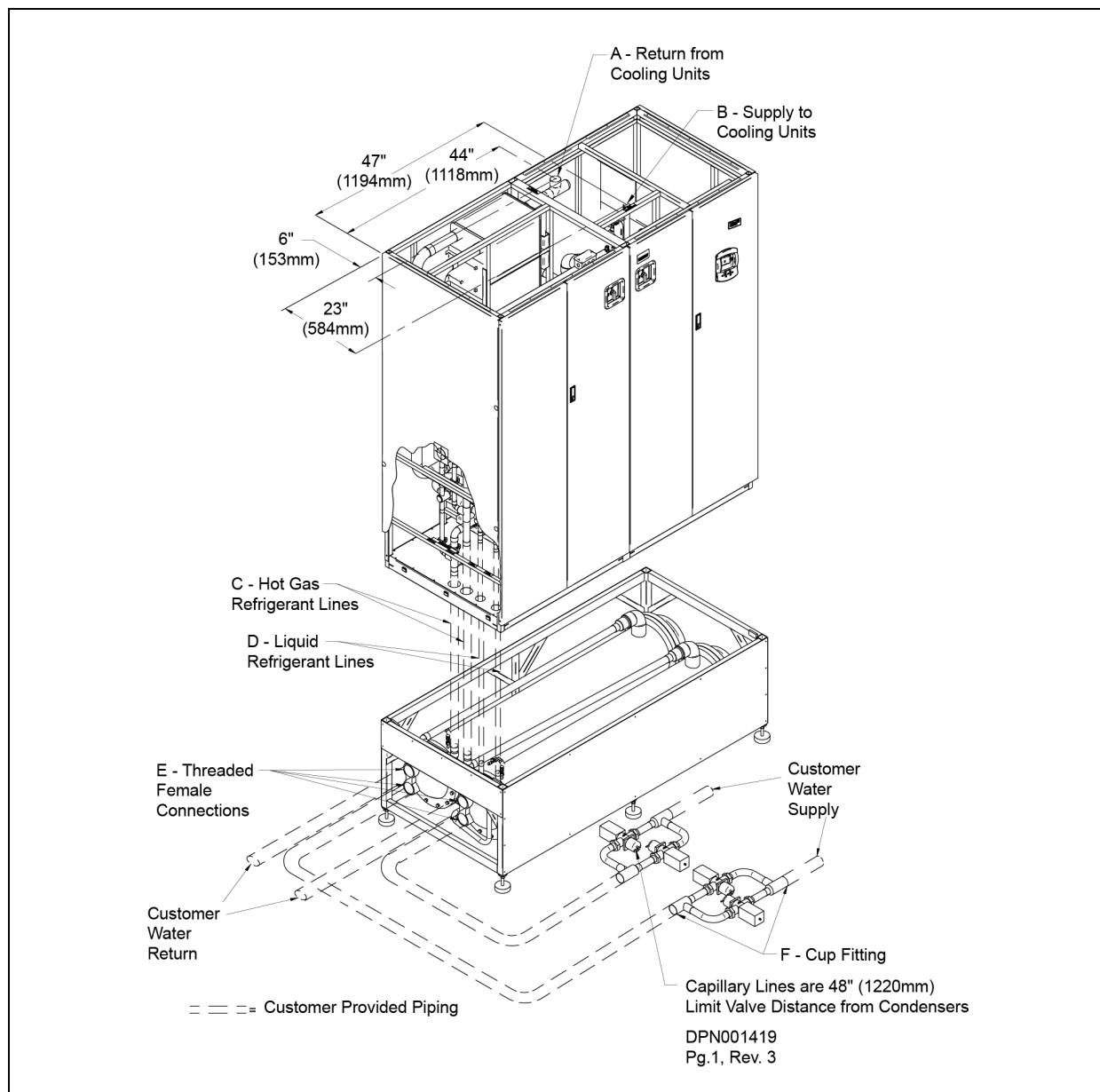
Figure 5.3 Positioning a water/glycol Liebert XDC for placement on a floor stand
