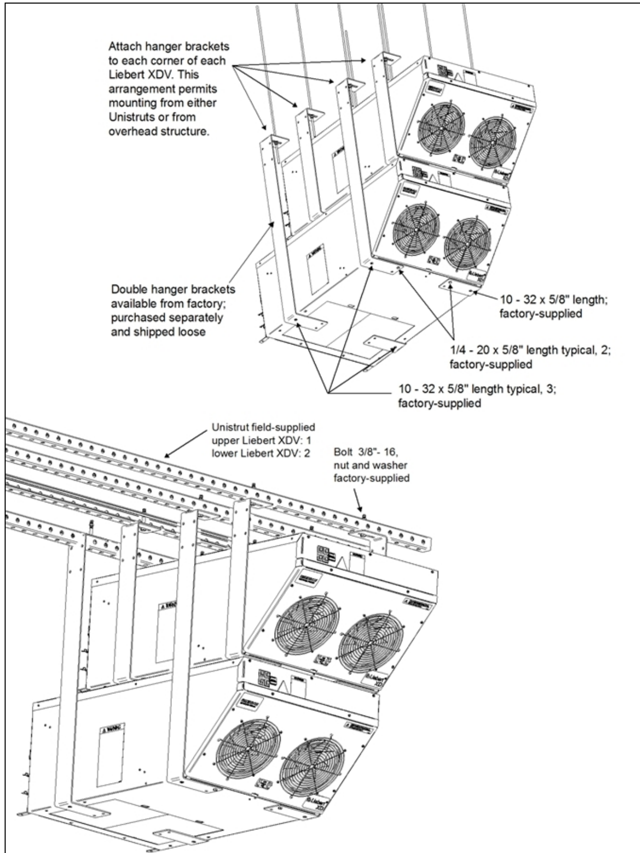
Figure 4.25 Alternate mounting methods—mounting multiple Liebert XDV modules
