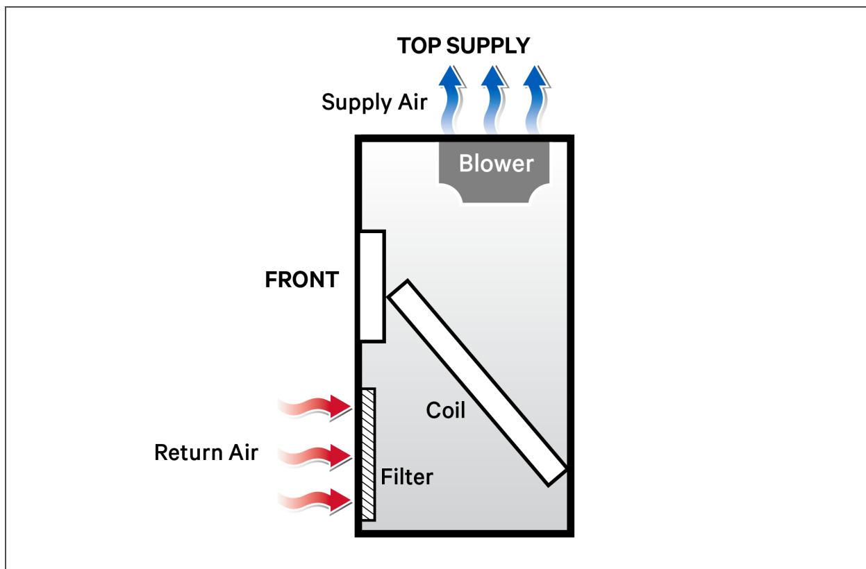
Figure 1.5 Upflow blower configuration, front air return
