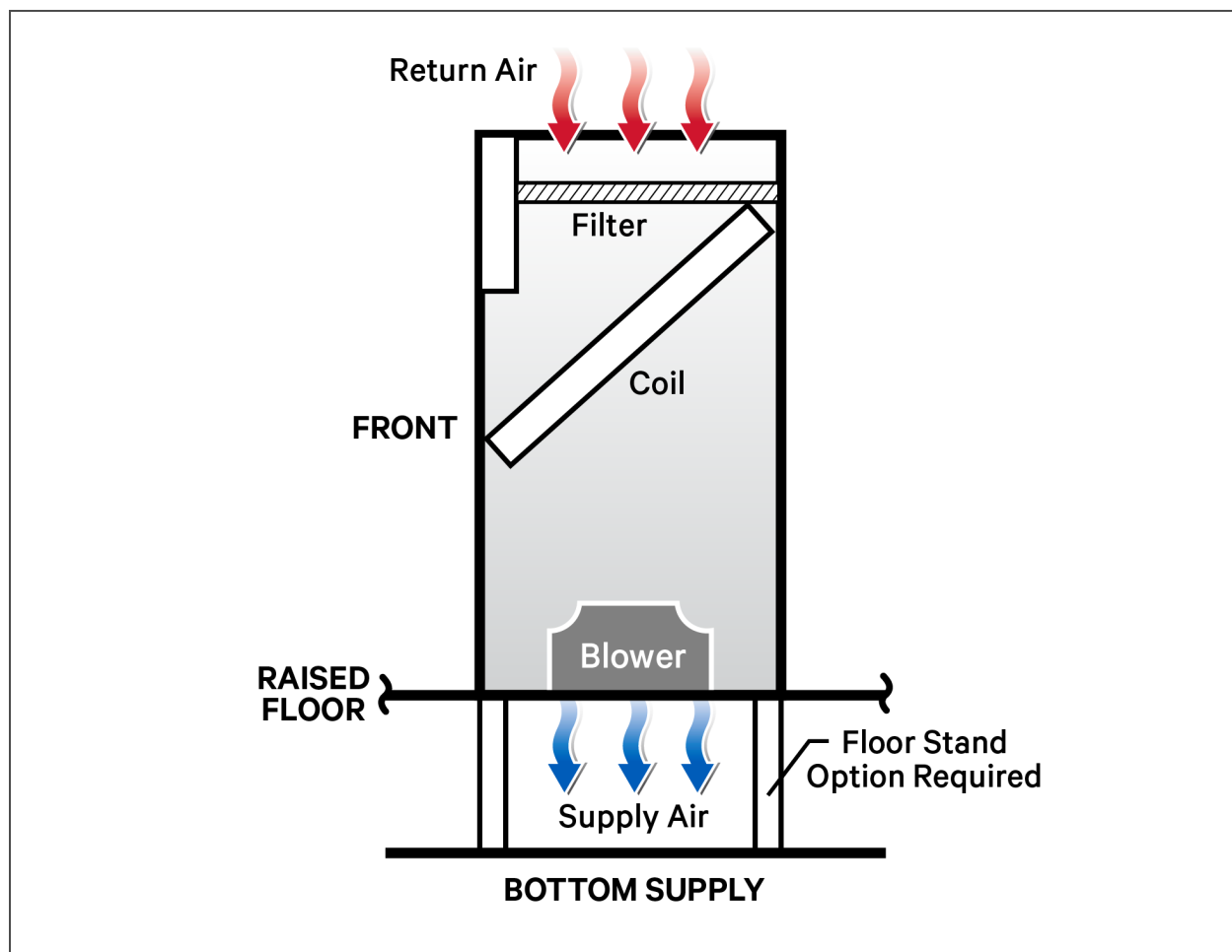
Figure 1.3 Downflow blower configuration, discharge into raised floor
