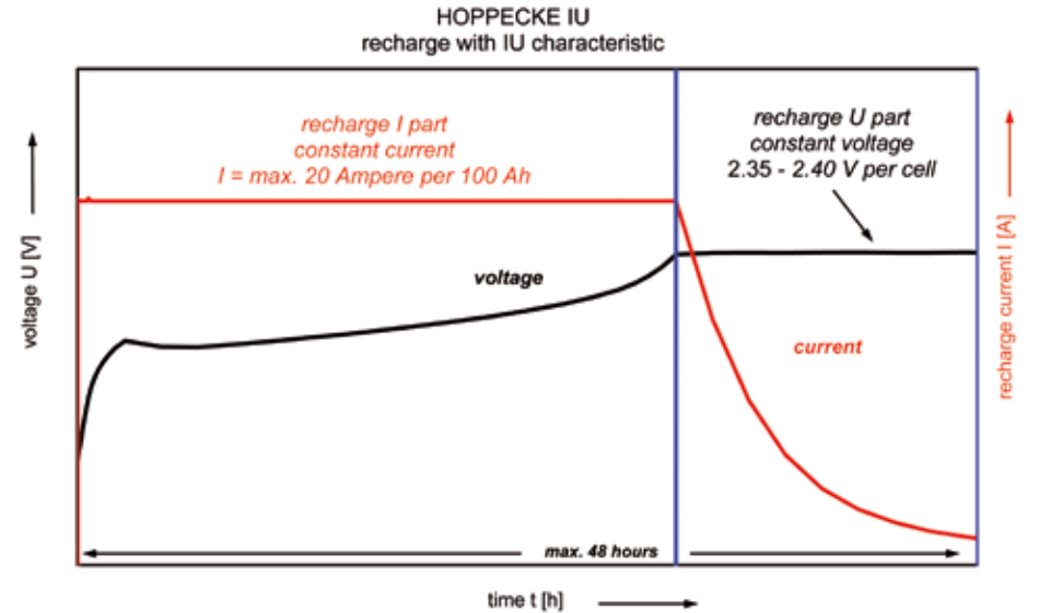
Fig. 9-1: IU characteristic
