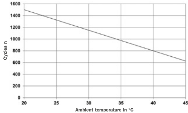
Fig. 7-9: Endurance in cycles of sun | power v L (OPzS solar.power) as a function of ambient temperature
