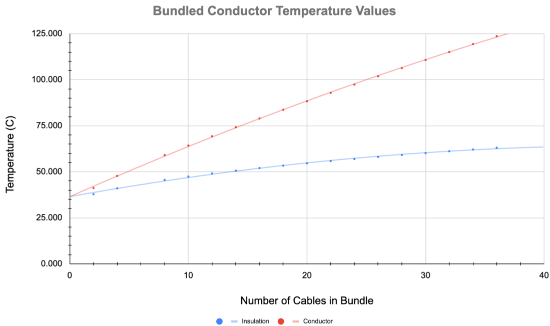
Figure 8 – Conductor temperature (red) and insulation surface temperature (blue) for the ‘fat cable’ approximation using increasing bundle sizes. Calculation is performed for a 1m cable length.
