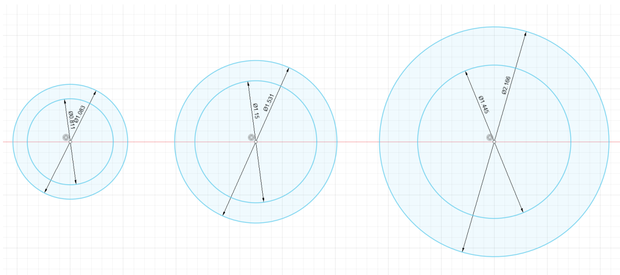
Figure 7 – equivalent representation of a single ‘fat cable’. Left is a single conductor, center is for two conductors, and right is for four conductors. The conductive area for four conductors is four times that of a single cable, and the current carried by the ‘fat cable’ is four times that of the single cable.
