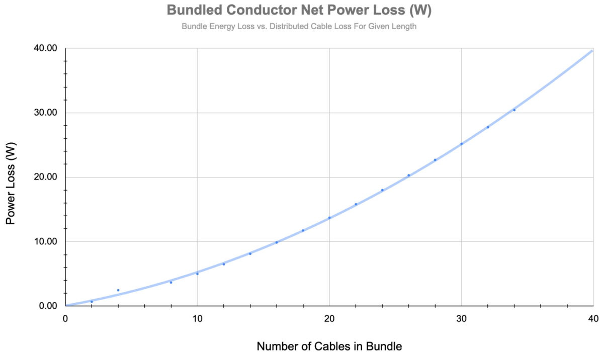
Figure 9 – Bundled power loss. The power loss is calculated in comparison to that of a single/discrete cable. For a 10-cable bundle, the power lost to Joule heating is compared to the power lost by 10 individual cables. Calculations are for a 1m cable length.
