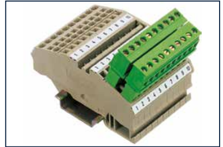
ZRK 2.5/4A combined with STL 950/10/5.08-G-L
