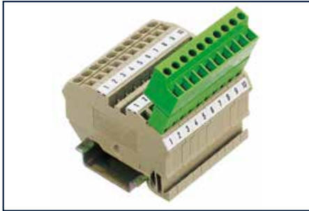
ZRK 2.5/2A combined with STL 950/10/5.08-G-L
