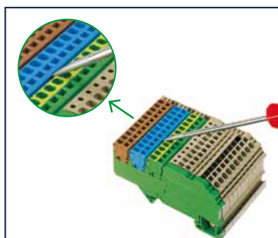
The ZPL potential distribution strip is easy to plug in or remove from the base terminal.
