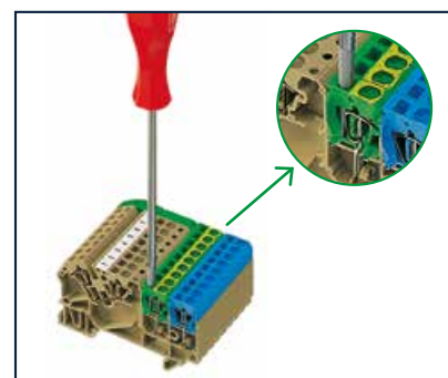
The TOP connection is easy to operate in cramped working conditions.
