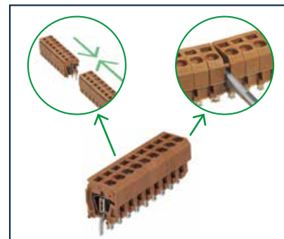
Potential distribution strip is easy to link and separate
