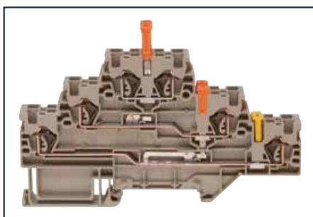
Vertical connection ZVQI
