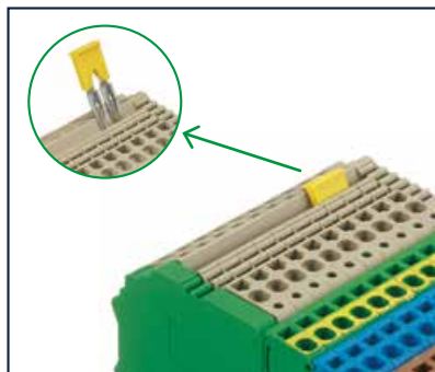
Pluggable cross-connection system ZQI , for the signal level, 2 – 10 poles (only ZINI/ZAKTO ).
