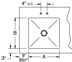
FLAT TOP, 1" or 1-1/2" REAR SPLASH
