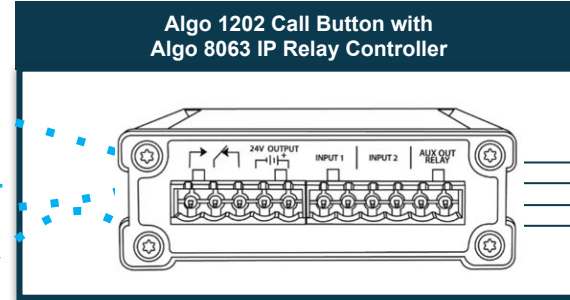
2 wire connections button input RJ 11
