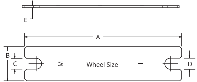
Wheel Stud Wrench
