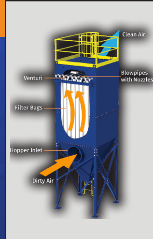
Top load filter change out and hinged filter access door
