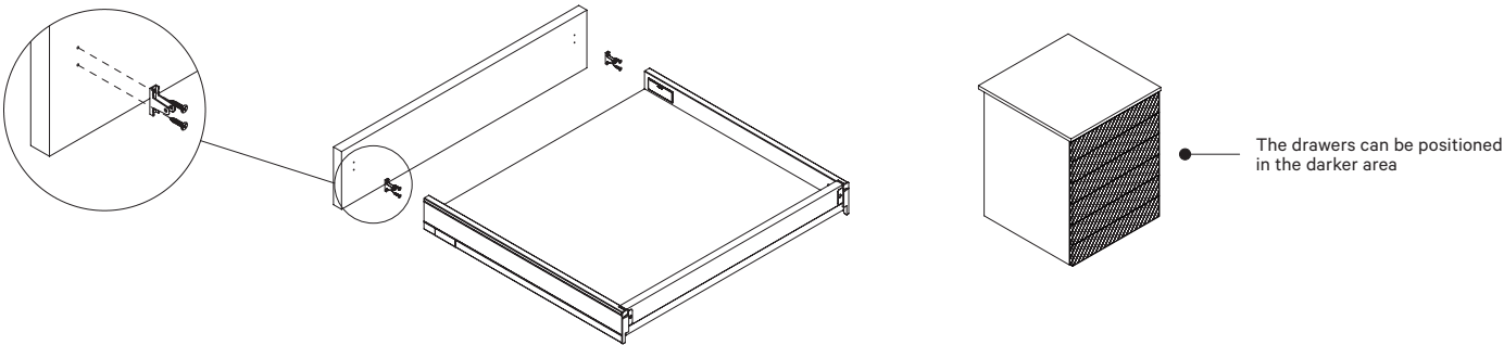
DRAWER FRONT POSITIONED IN: 1ST AND 2ND HOLE COUNTING FROM THE BOTTOM.
