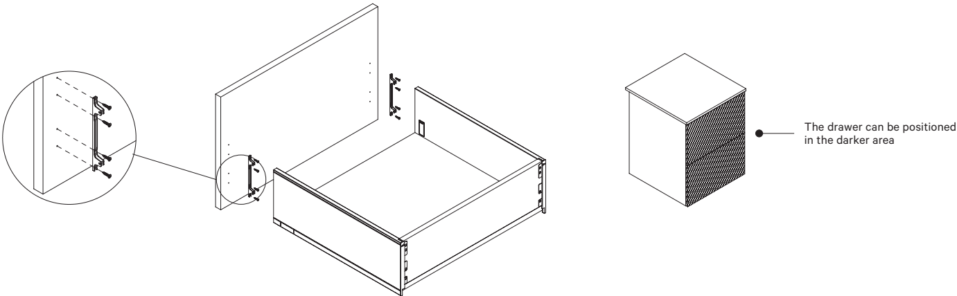
DRAWER FRONT POSITIONED IN: ALL HOLES COUNTING FROM THE BOTTOM.
