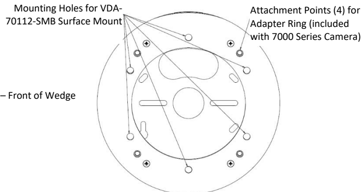
Figure 3 – Adapter Ring Orientation
