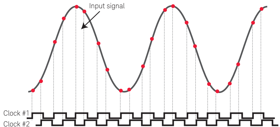
Figure 9. Timing diagram showing non-evenly spaced samples.
