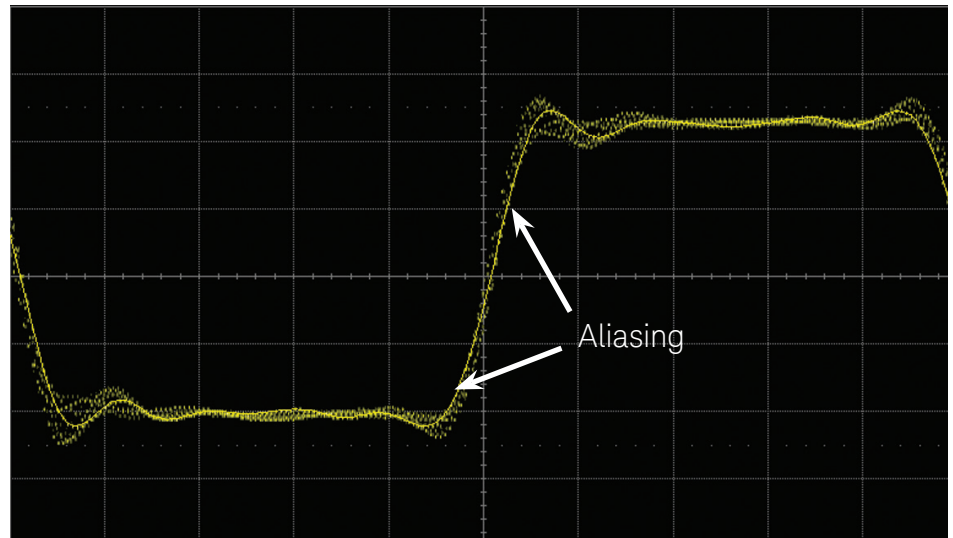
Figure 4. 500-MHz bandwidth scope sampling at 1 GSa/s produces aliased edges.
