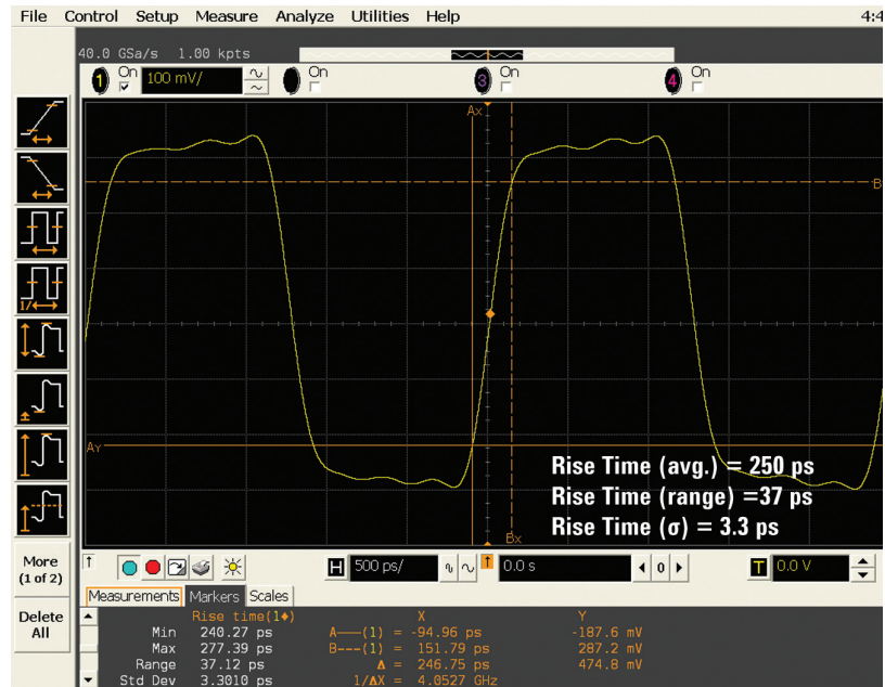
Figure 15a. 400-MHz clock captured on a Keysight Infiniium 3-GHz oscilloscope sampling at 40 GSa/s.
