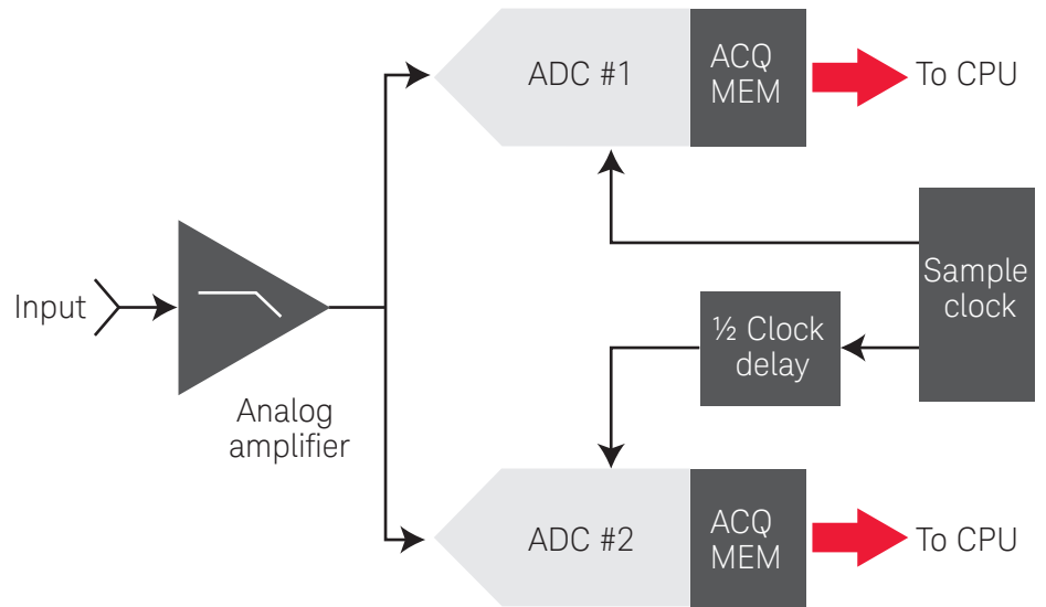
Figure 8. Real-time sampling system consisting of two interleaved ADCs.
