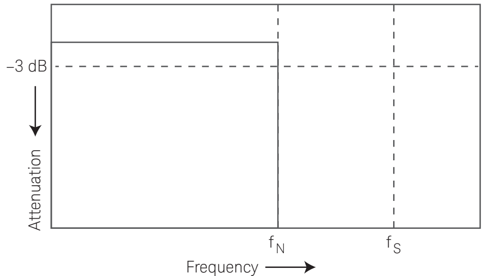
Figure 2. Theoretical brick-wall frequency response.
