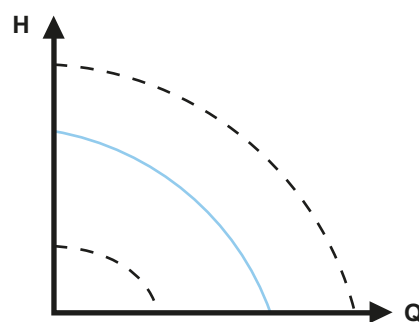
Fig. 26 Constant-curve duty
