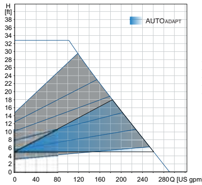
Proportional pressure
