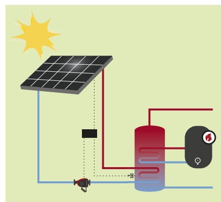
Fig. 13 Functional drawing of a solar-heating system
