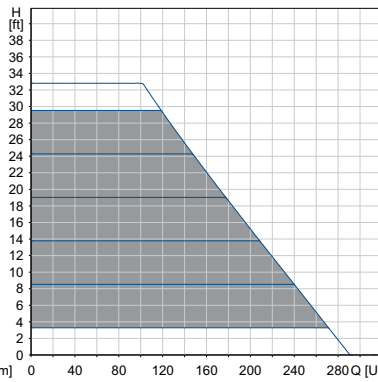
Constant pressure
