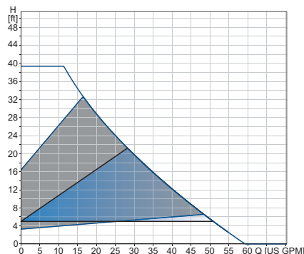
Proportional pressure
