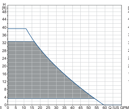
Constant pressure
