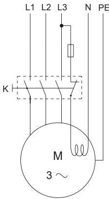
Three-phase motor with space heater
