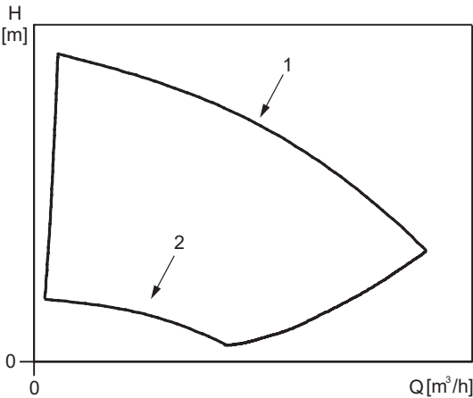
Maximum (1) and minimum (2) performance curves
