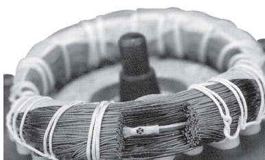
PTC sensor incorporated in winding
