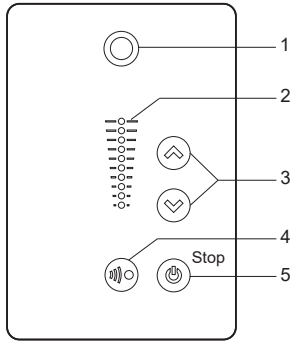
Standard operating panel for CRE pump, 1/2-15 HP
