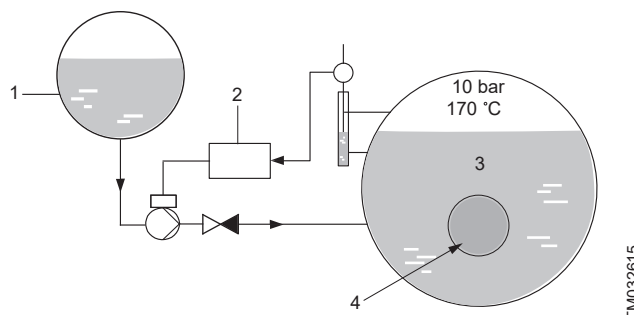
Boiler-feed application with speed-controlled pump
