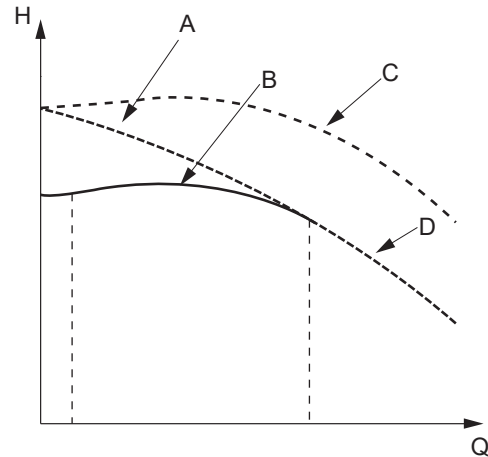
Pump curve with a stabilized operating range
