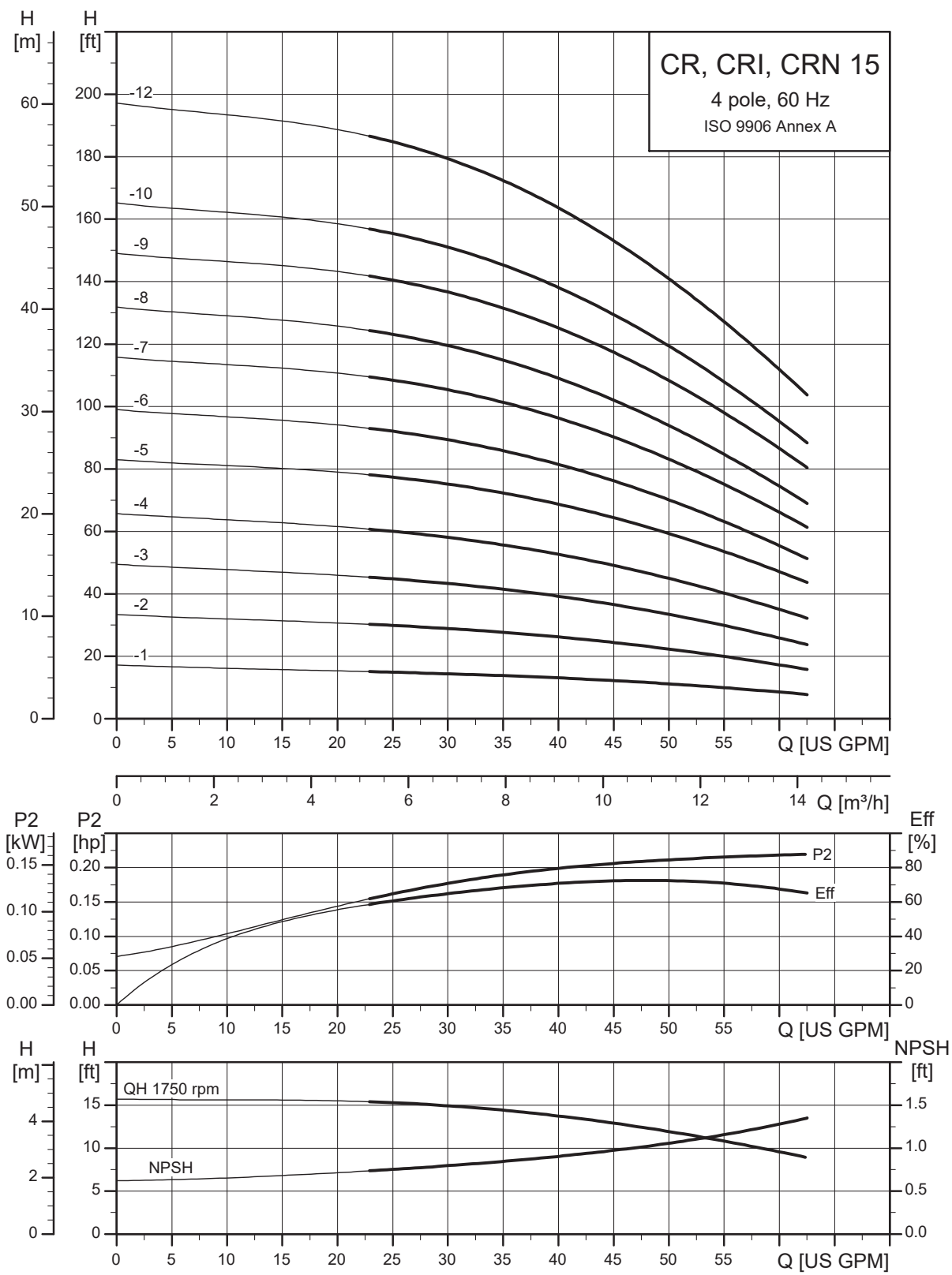
CR pumps with 4-pole motor: CR, CRI, CRN 15
