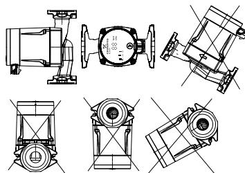
Fig. 2 Installation positions
