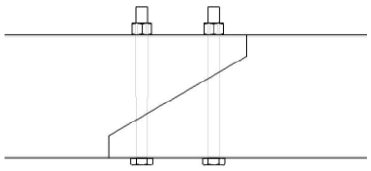
“Angled Shiplap”
