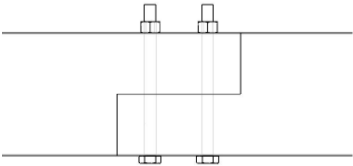
“Standard Shiplap”
