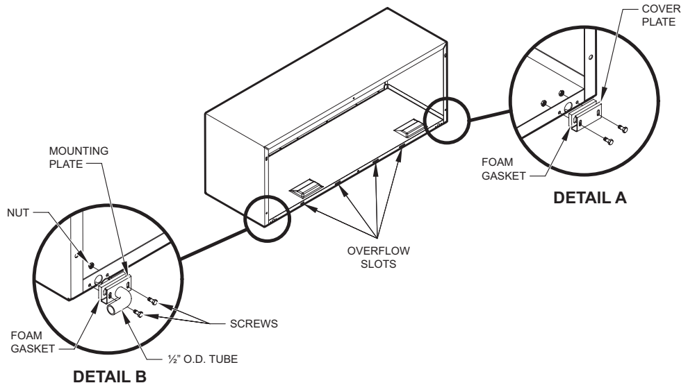
DETAIL B
