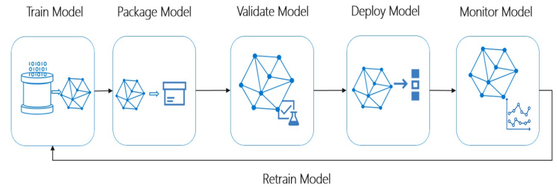
ML Model Life Cycle
